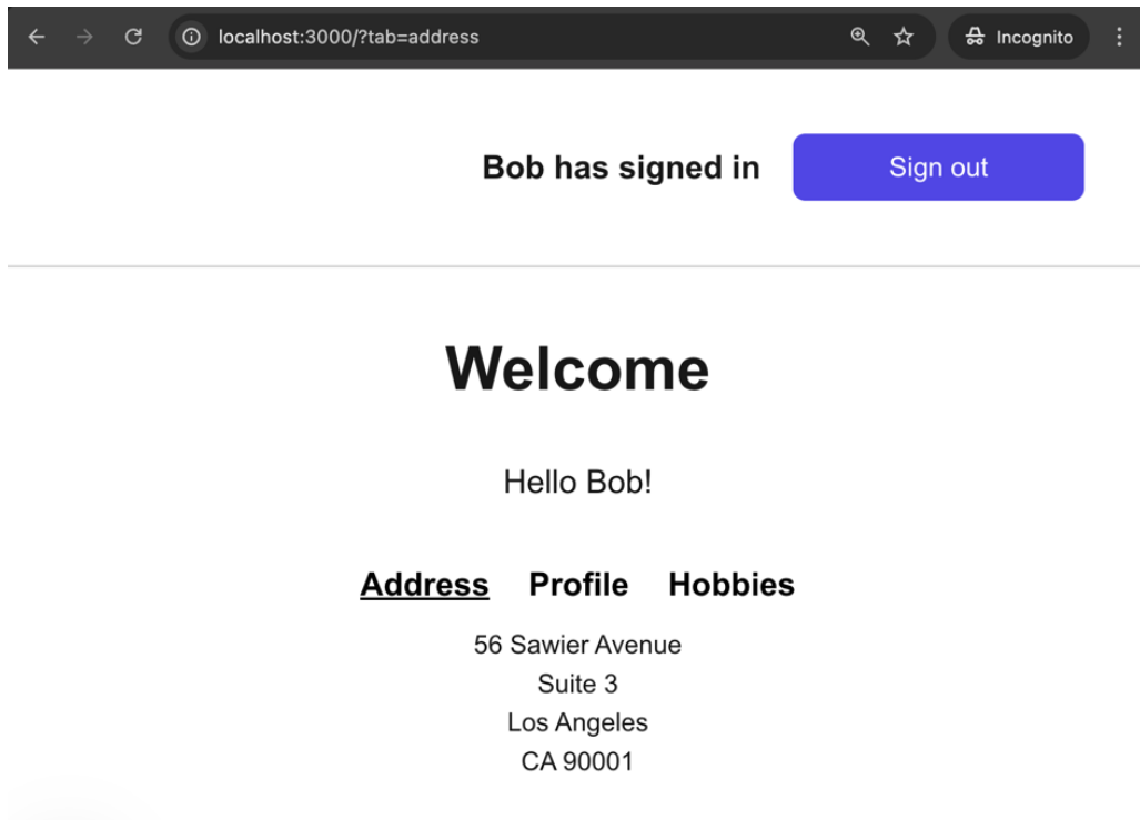
Figure 10.6 – Extended app
