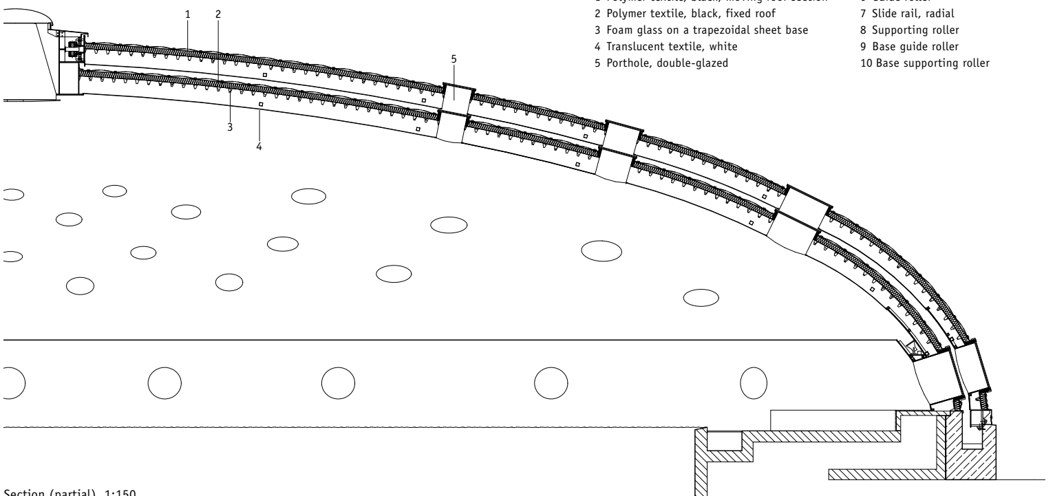
Section (partial), 1:150
