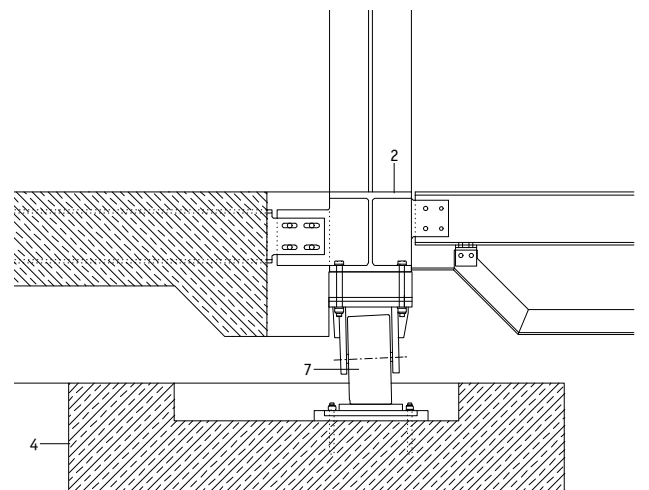
Wheel assembly, 1:35
