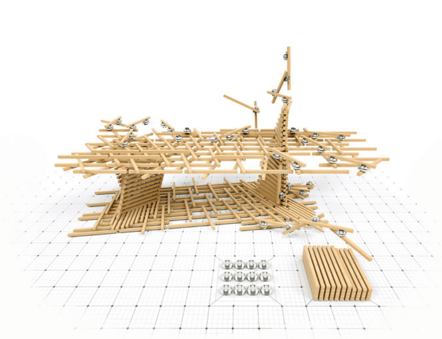
Distributed robotic assembly system for in situ timber construction, ITECH, Samuel Leder, Ramon Weber, 2018
