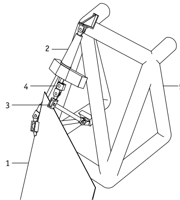
Axonometric projection showing drive, truss beam and lamella anchorage – 200 to 30 mm reinforcement at the vertical edges of the lamella
