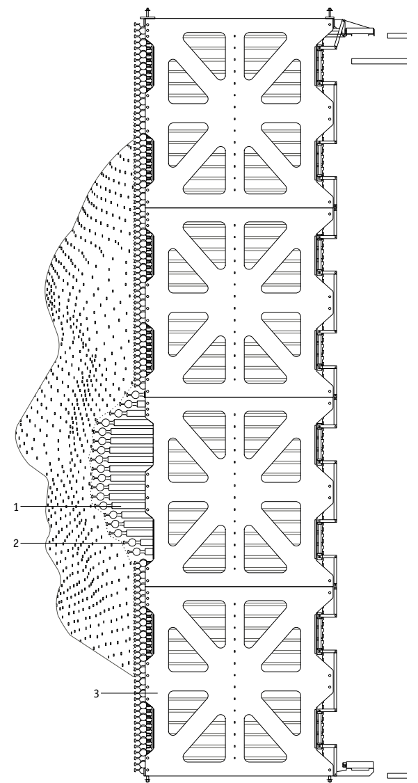
Vertical section, 1:65
