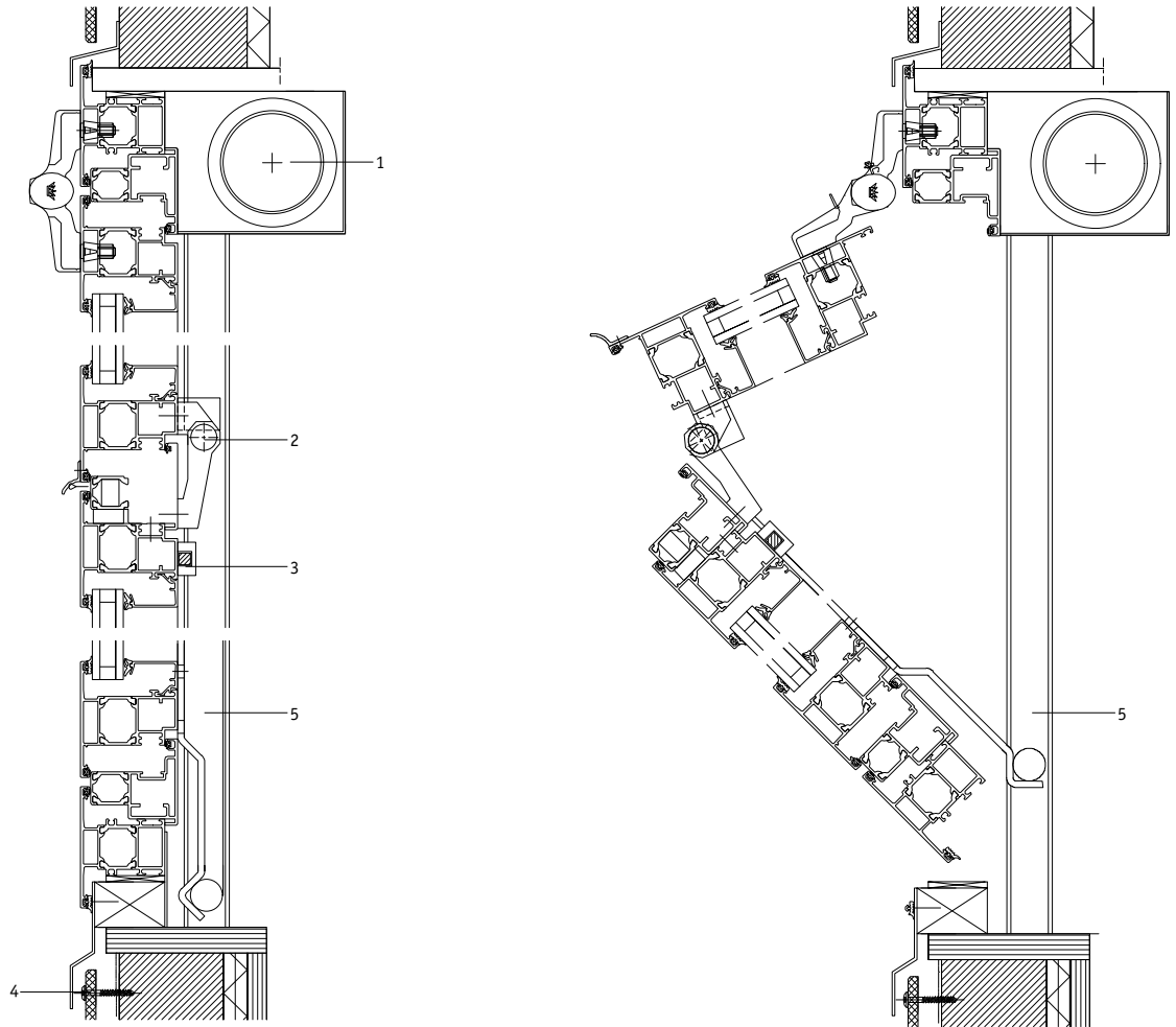
Vertical section, 1:5
