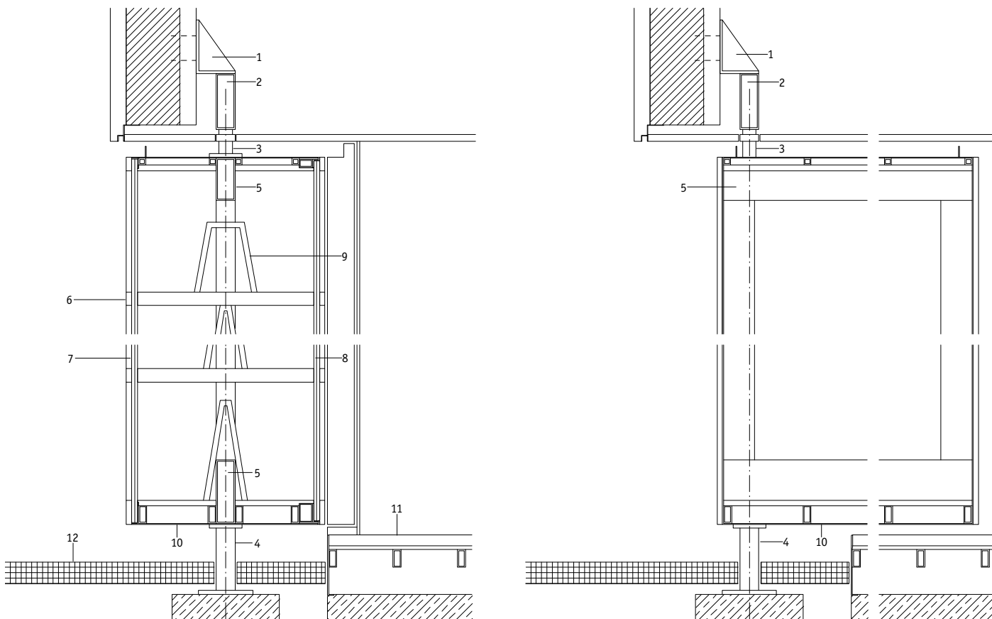
Vertical section with closed and open facade element, 1:10
