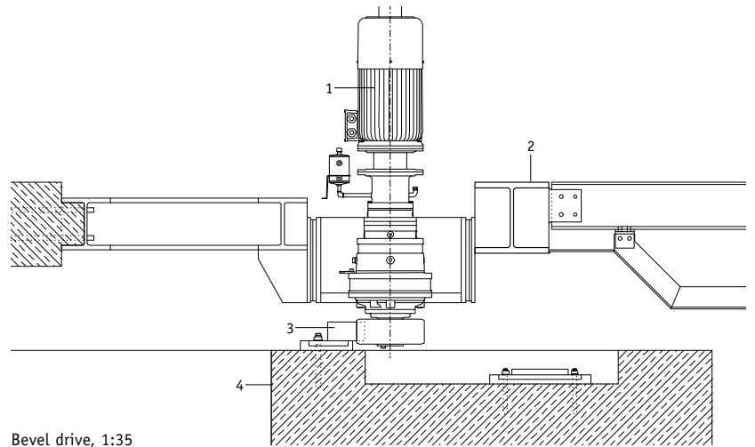
Bevel drive, 1:35
