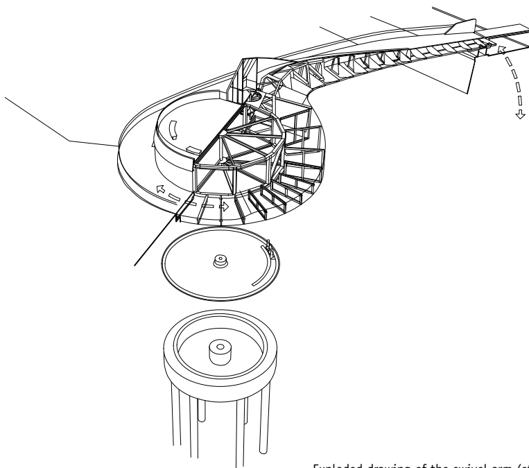
Exploded drawing of the swivel arm (steel structure) showing movement mechanism and support
