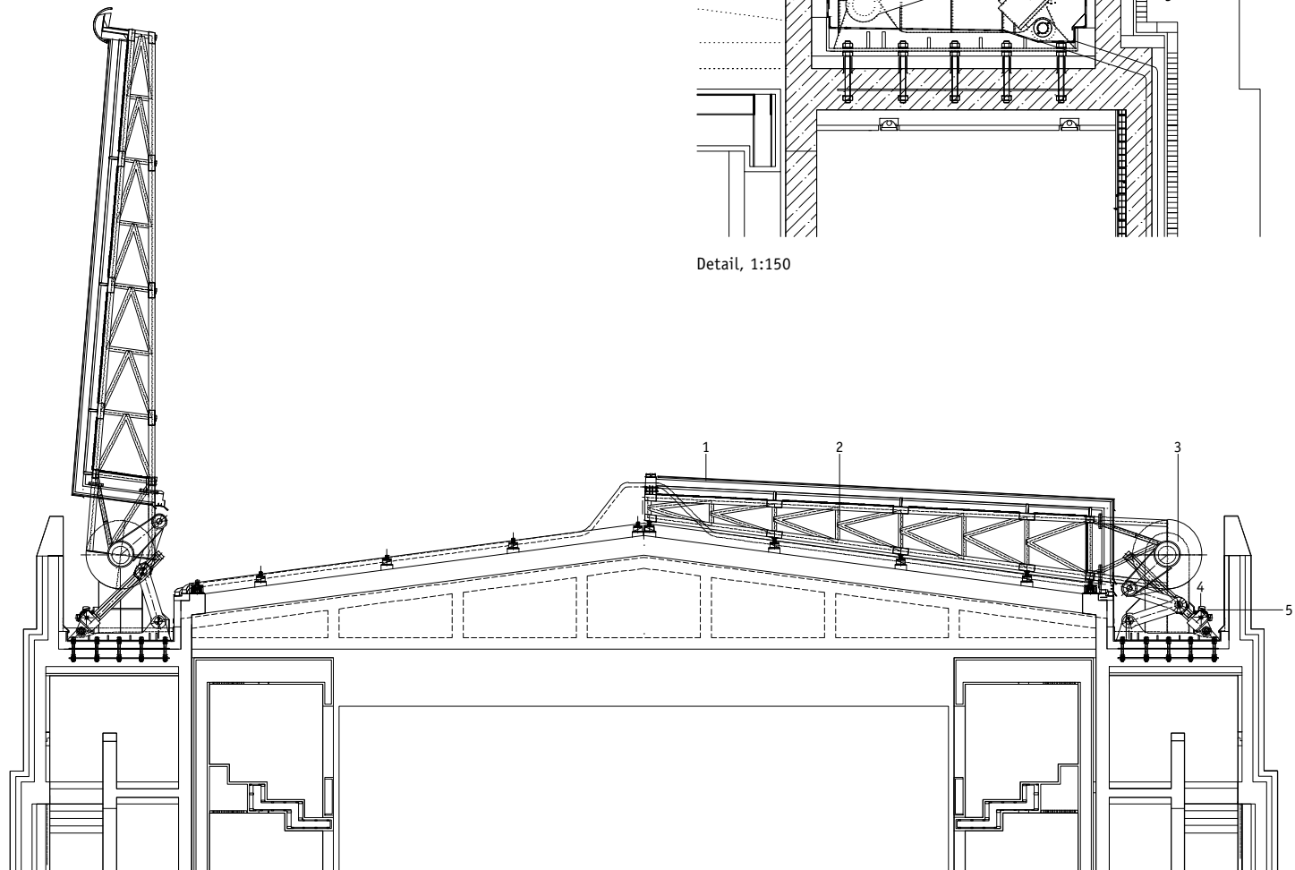
Section, 1:350
