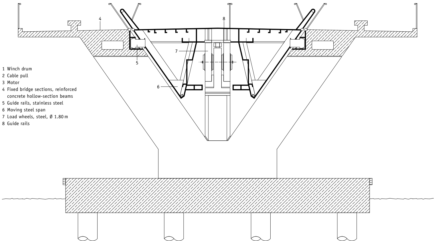
Cross section through bridge, 1:100
