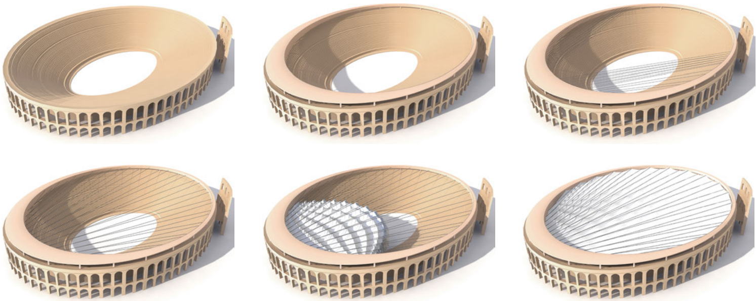
Closing sequence of the proposed roof over the Arena di Verona
