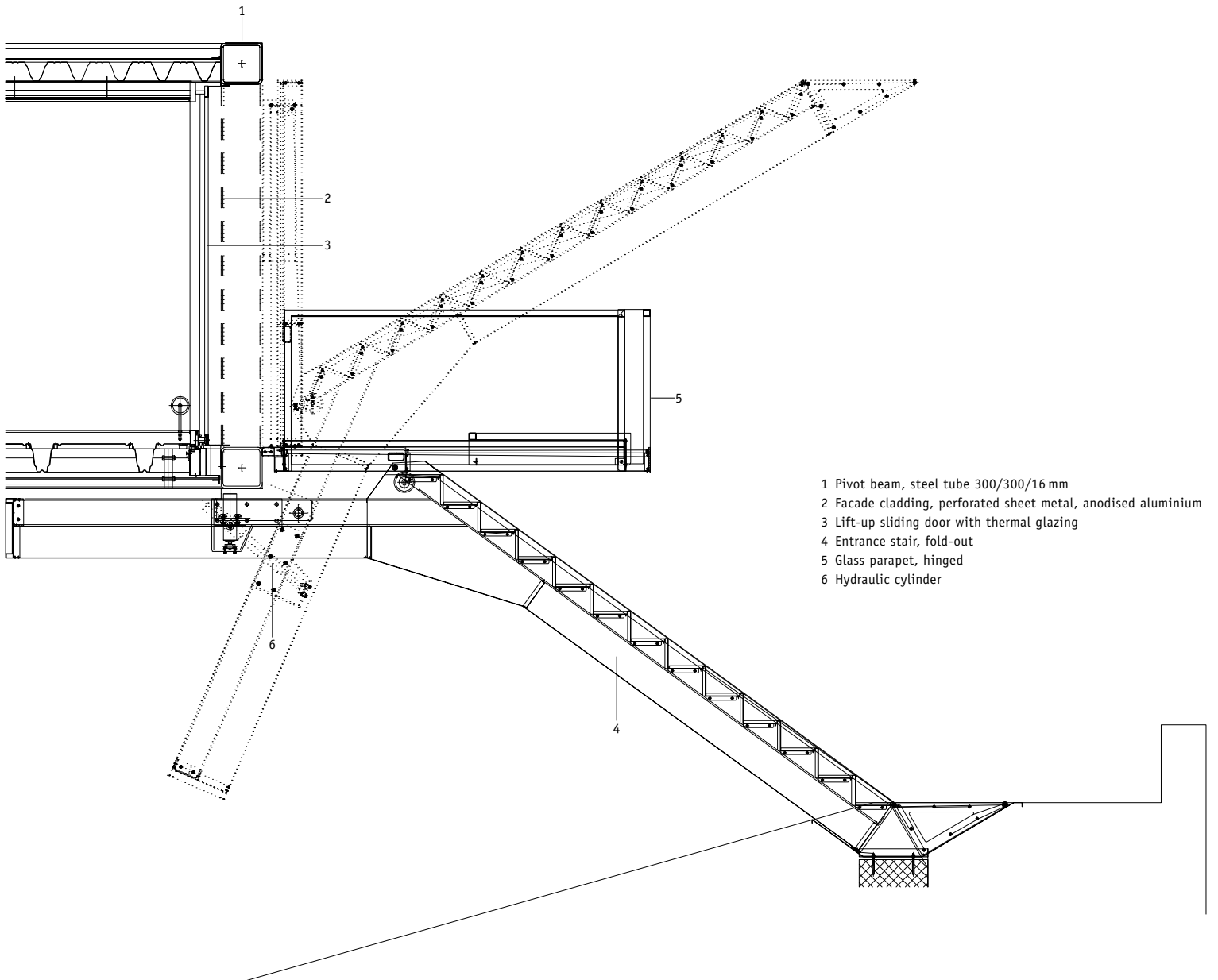
Section, 1:50
