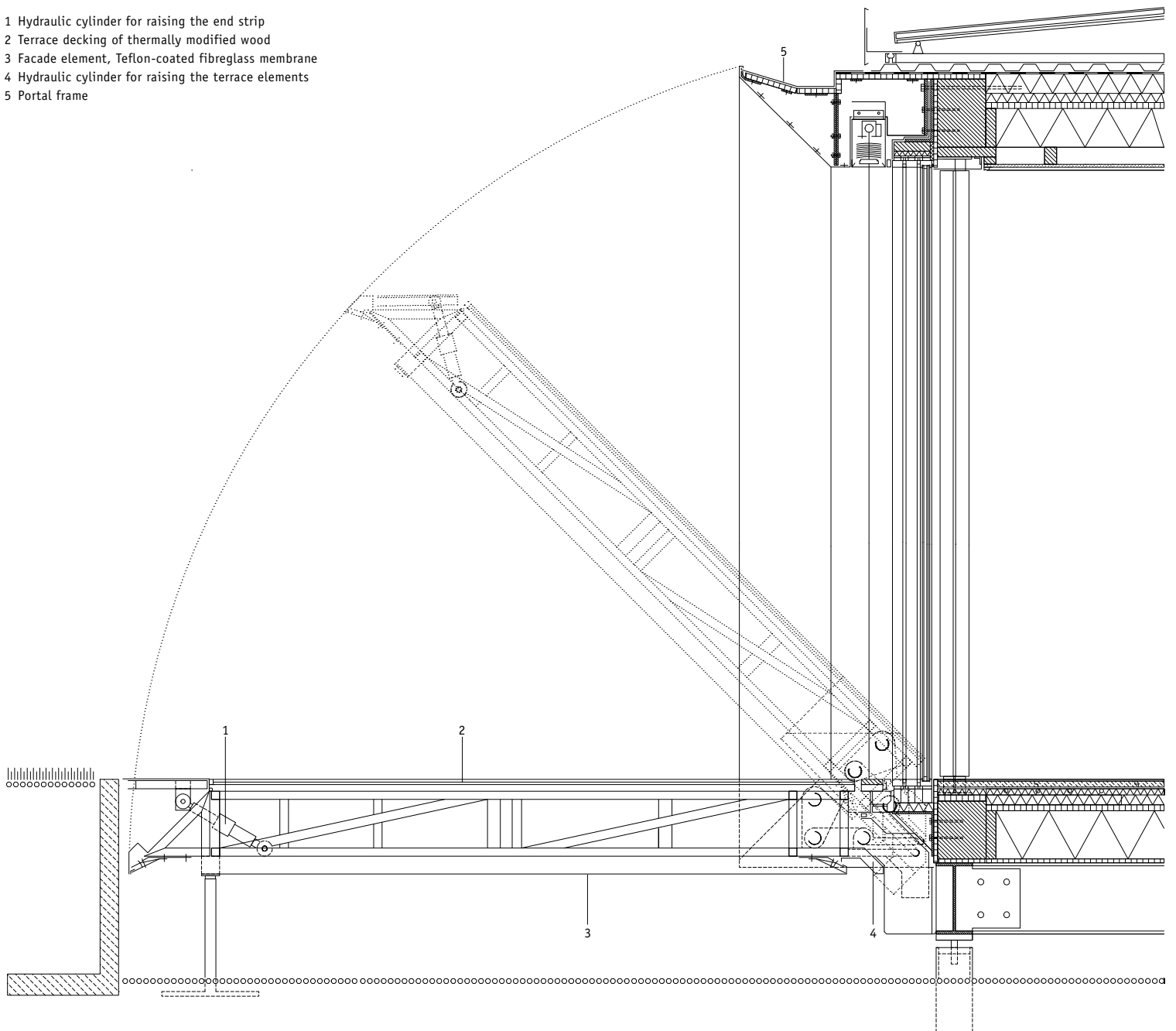
Cross section, 1:25
