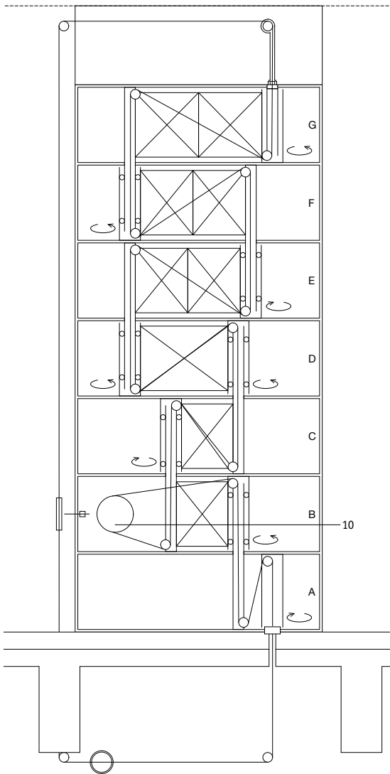
Elevation, 1:50
