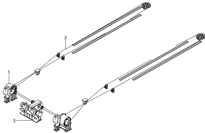
Axonometric projection of the winch drive mechanism
