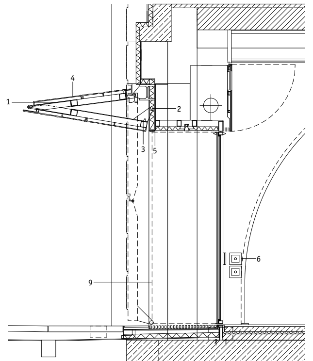
Vertical section, 1:50
