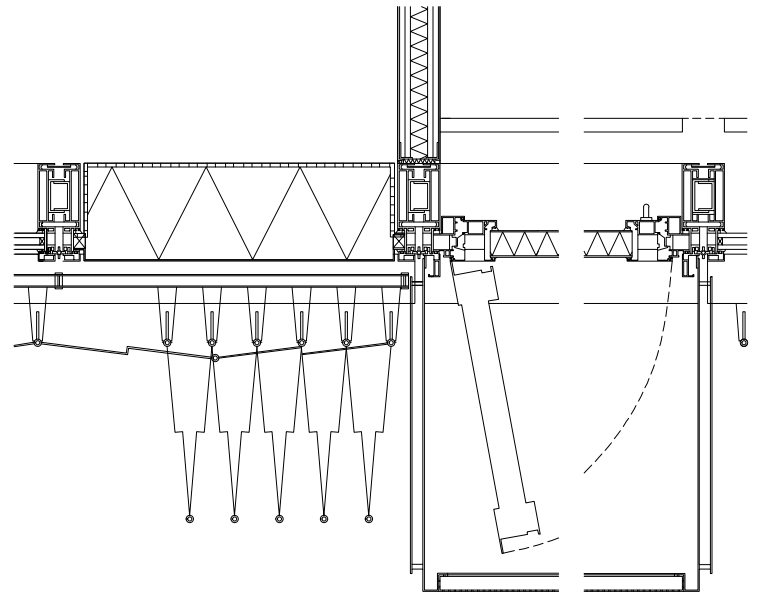
Horizontal section, folding sliding shutter in open position, 1:25
