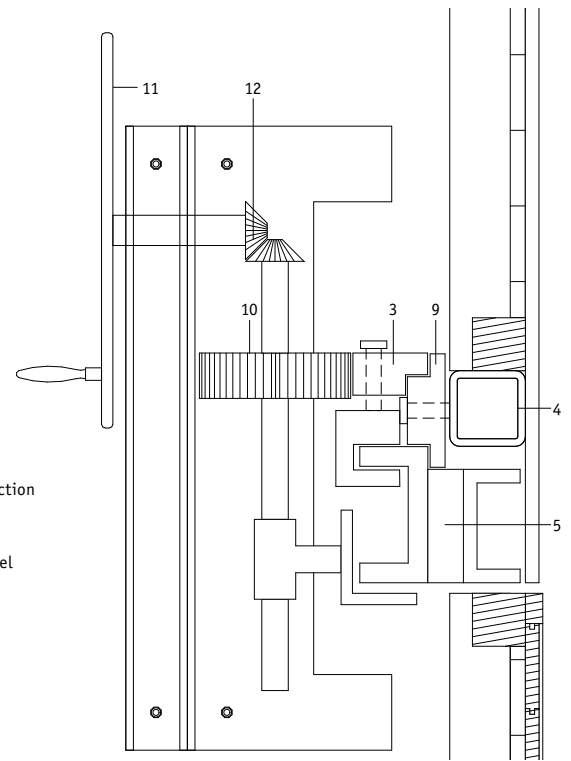
Sectional elevation of drive mechanism, 1:10
