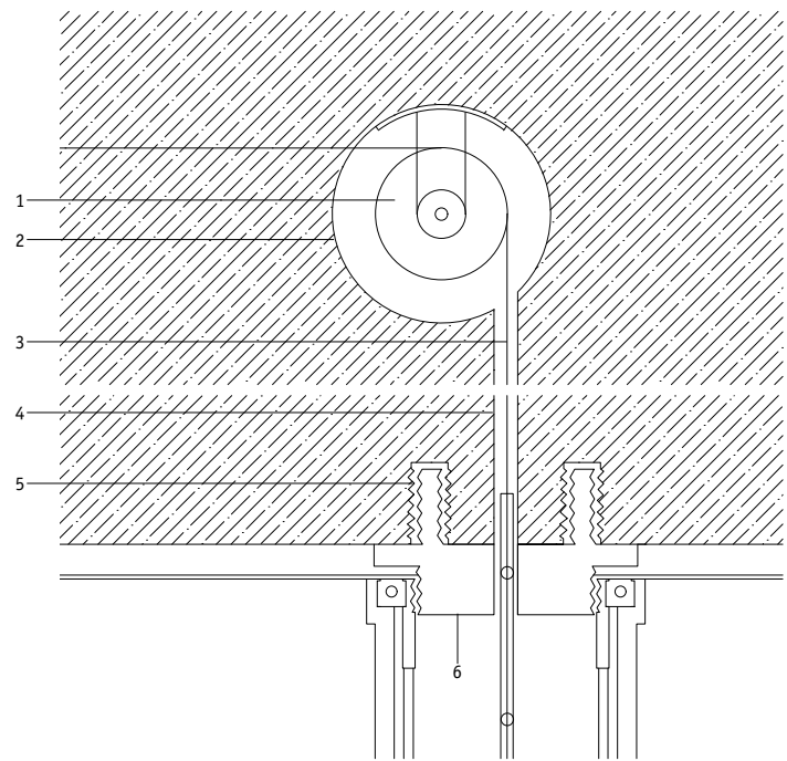
Detail, 1:10
