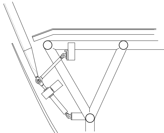
Section of bottom mounting showing drive and lamella anchorage
