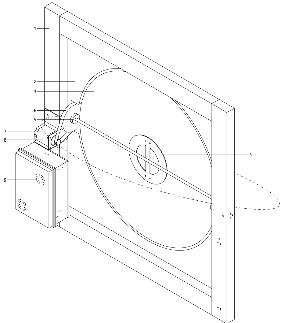
Axonometric projection of an element, 1:10
