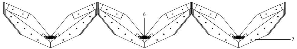
Wooden elements, 1:25
