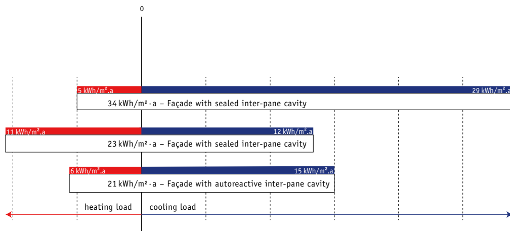
Double-skin glass facades in comparison: energy consumption per year and m 2 surface area
