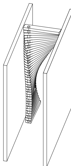
Axonometric projection of door situation and axis of rotation
