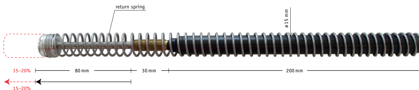
Cylindrical thermal actuator with return spring
