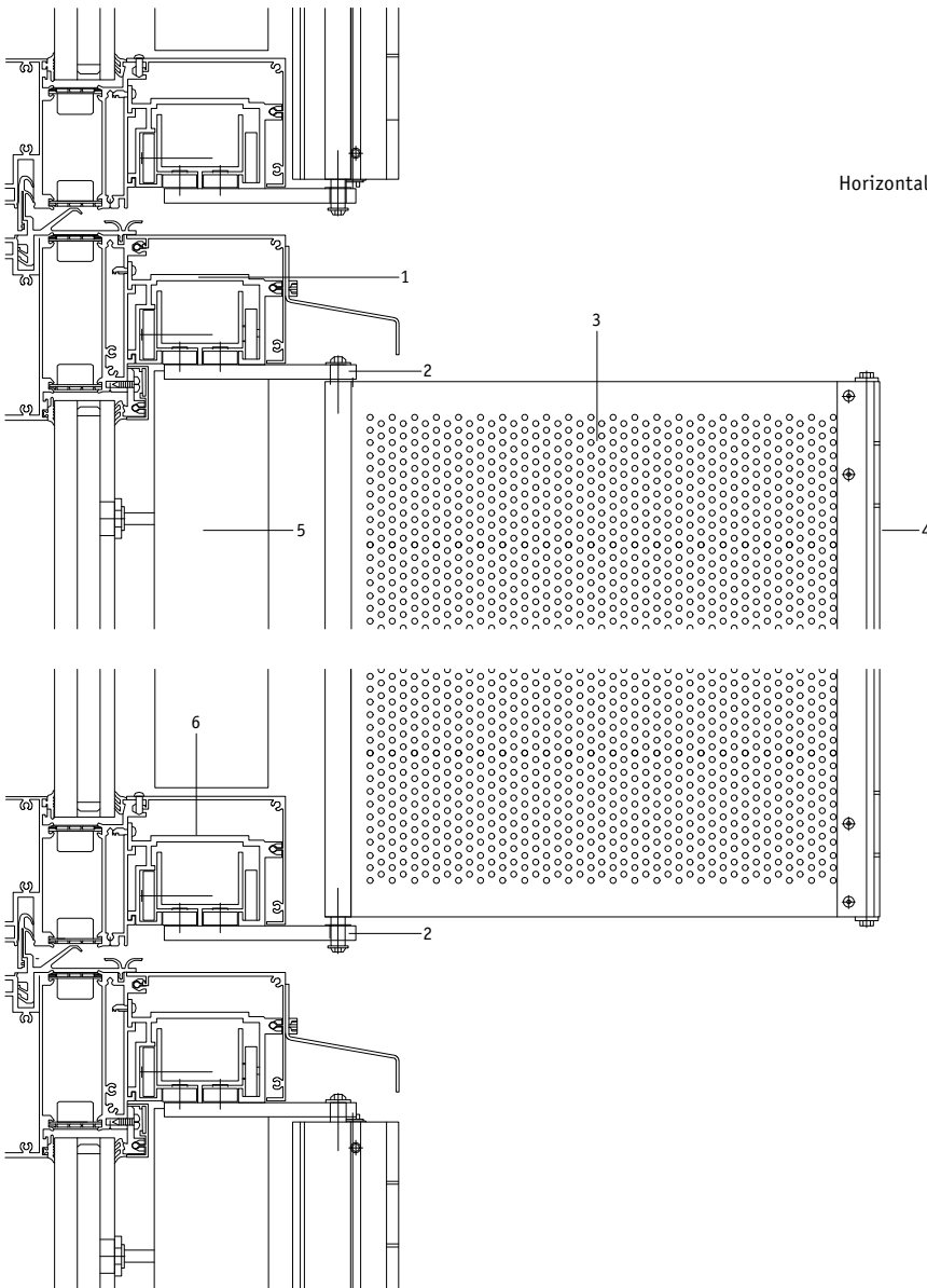
Vertical section, folding sliding shutters in open position, 1:4
