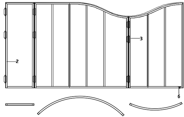
Flattened elevation of folding wall, 1:50
