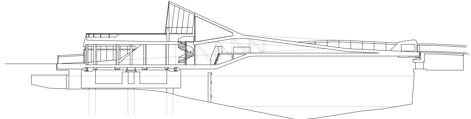
Section, 1:500
