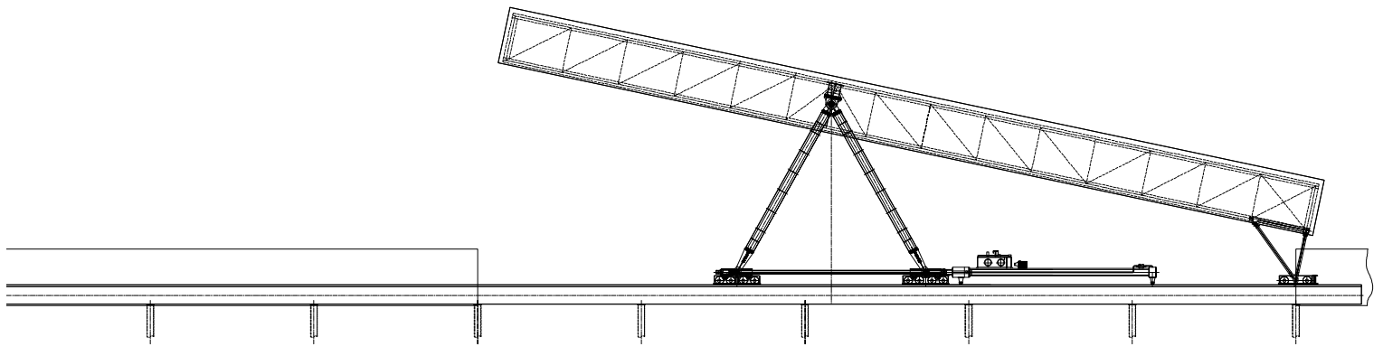
Elevation, 1:600
