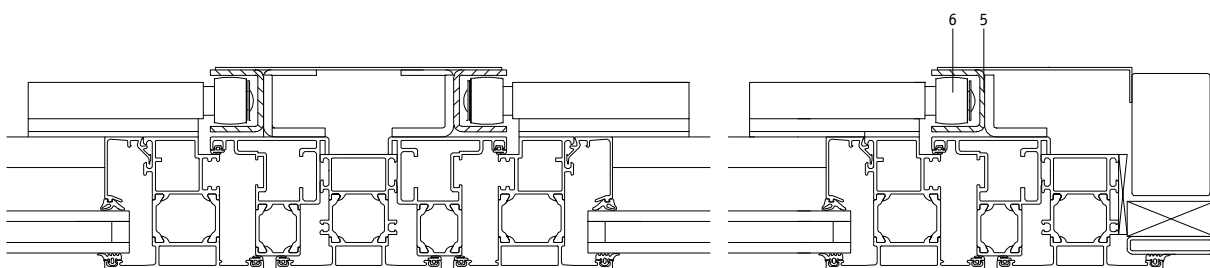
Horizontal section, 1:4
