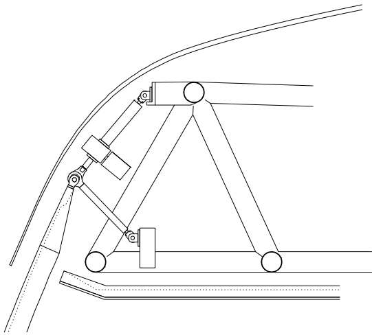
Section of top mounting showing drive and lamella anchorage
