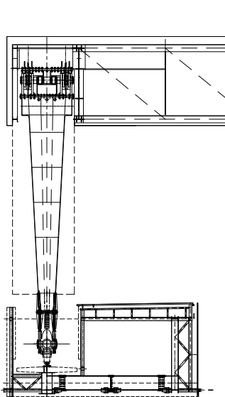
Sections, 1:300
