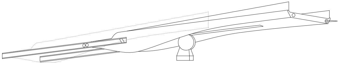
Axonometric projection of lateral guide rails of the bridge deck
