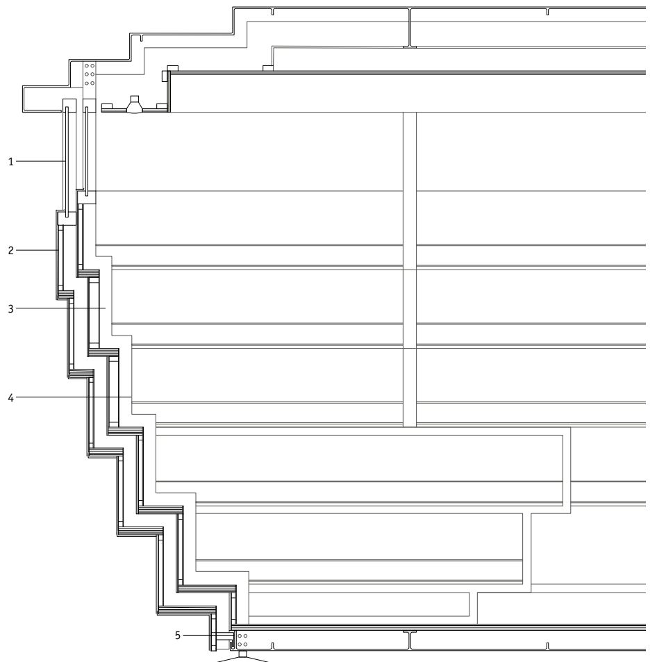
Section, 1:20
