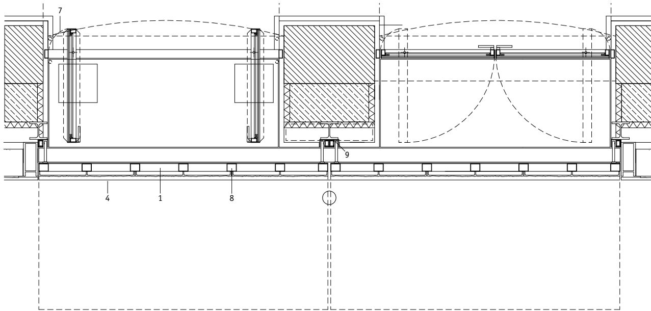
Floor plan (detail), 1:50
