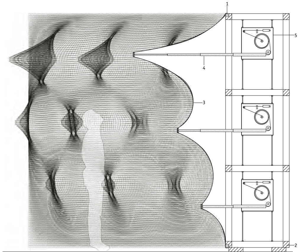
Cross section, 1:33
