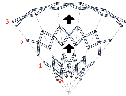
Planar scissor linkage with angulated scissor unit
