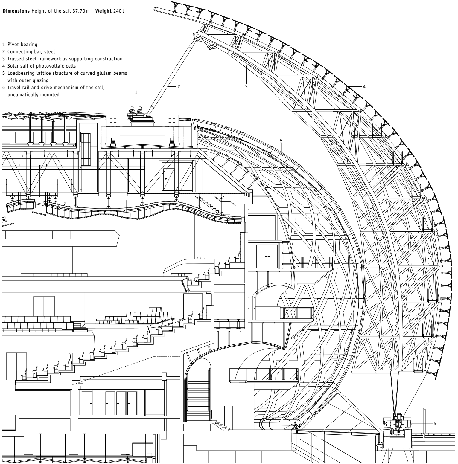
Section through building and rotating element, 1:200
