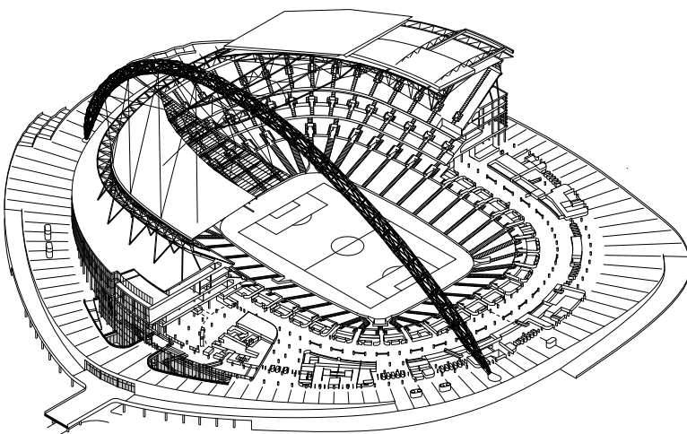
Axonometric projection of the stadium with longitudinal section
