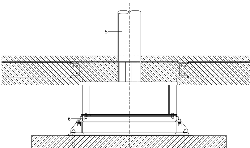
Central spindle, 1:35
