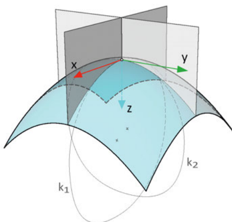
Gaussian curvature
