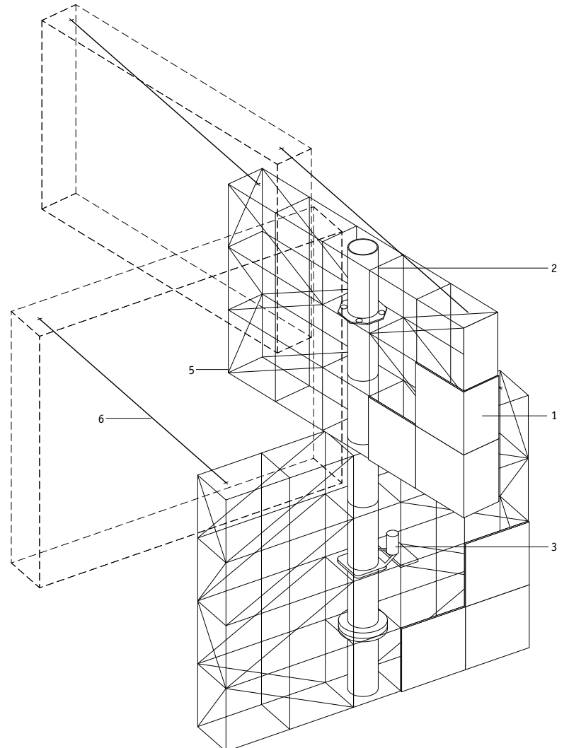
Axonometric projection of an individual element
