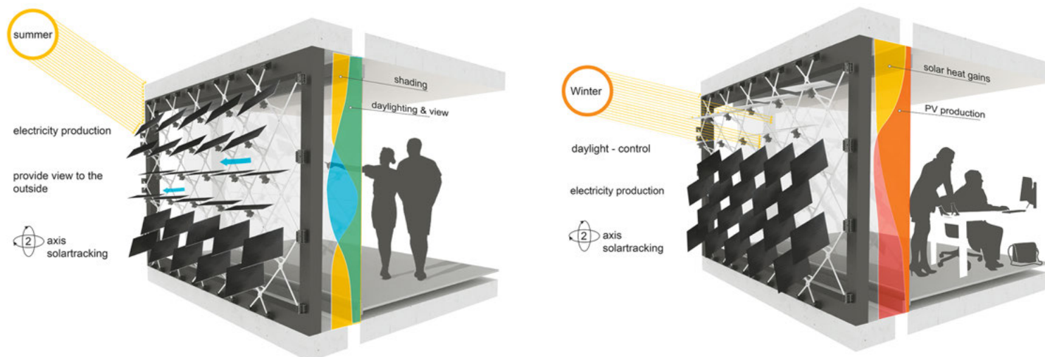
Functions of the different parts of the ASF during the summer and winter months. Image from Svetozarevic et al. 1
