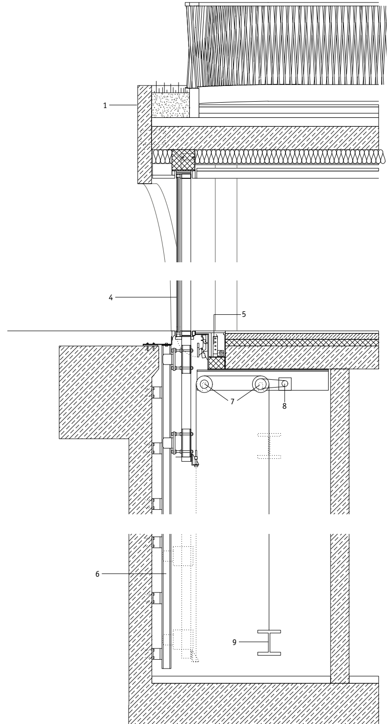
Section through facade, 1:40
