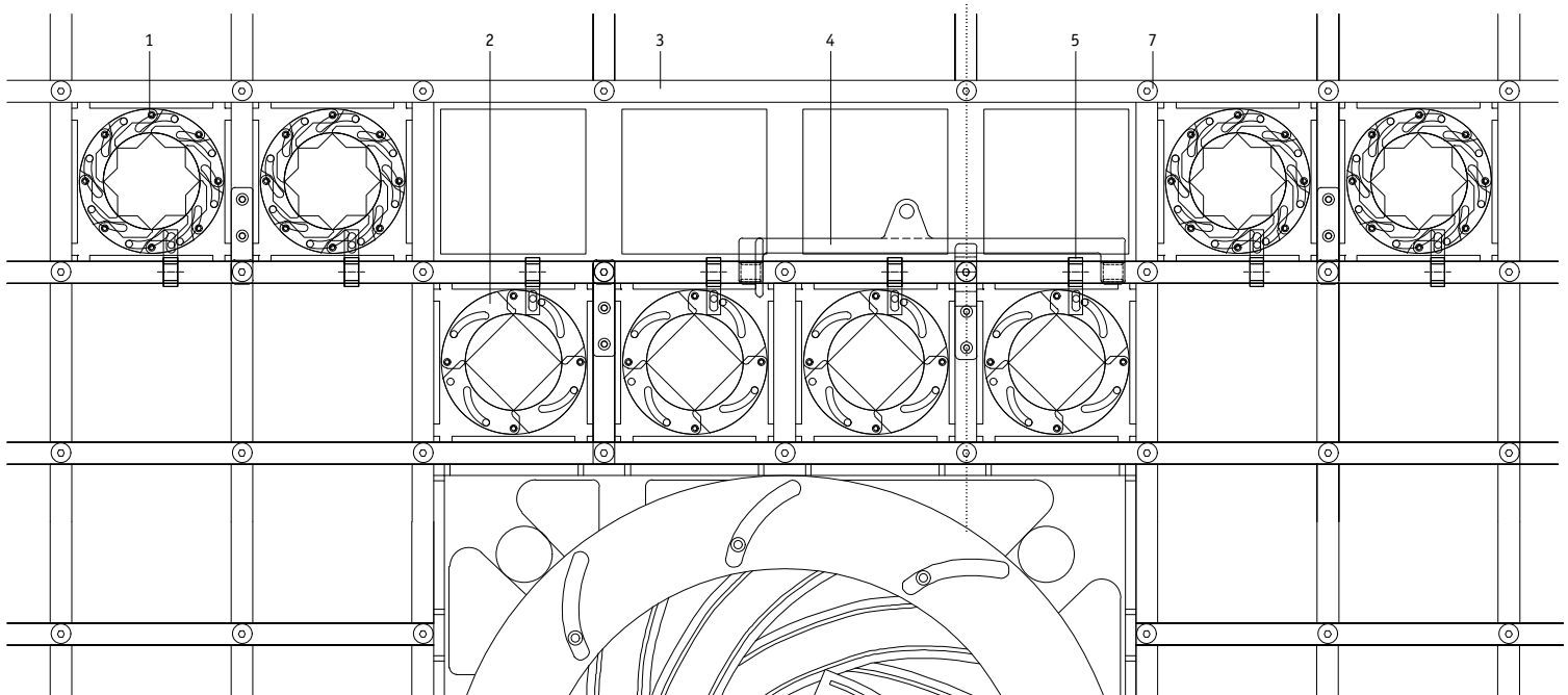
Elevation, 1:65
