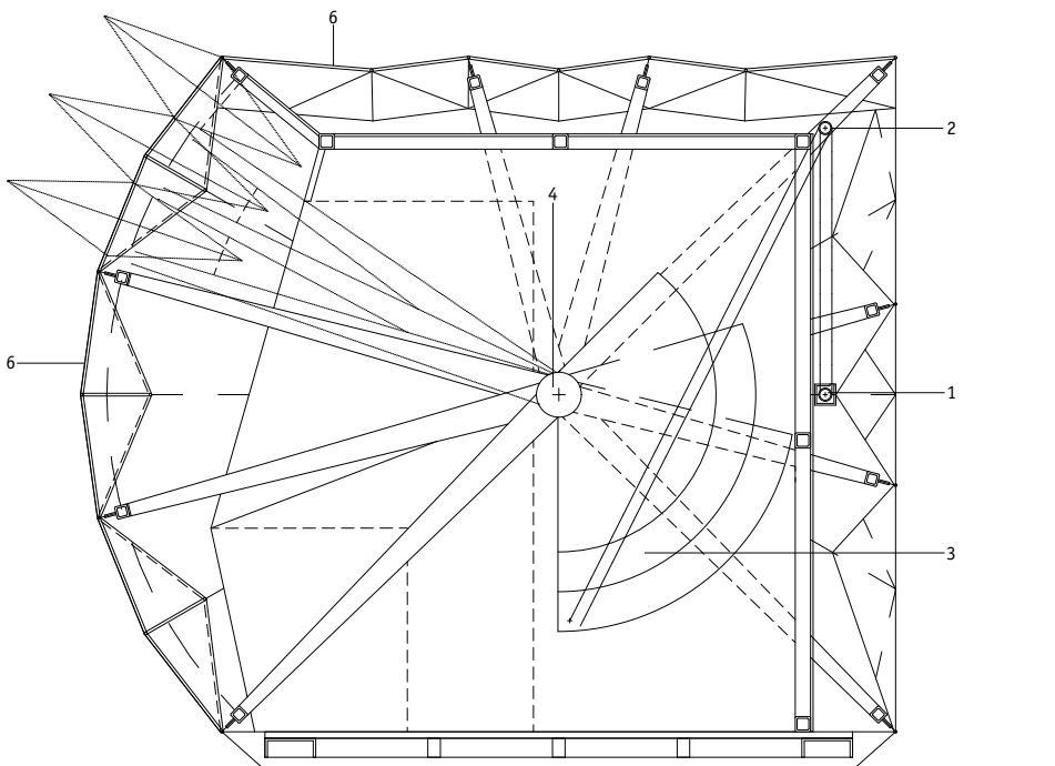
Section, M 1:33
