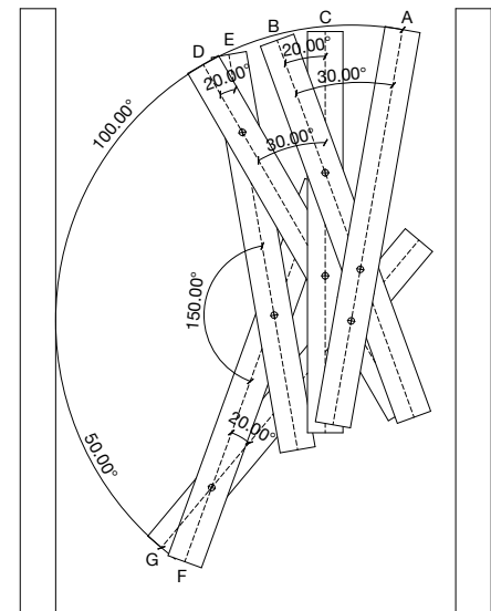
Top view of rotation positions and angles of door segments
