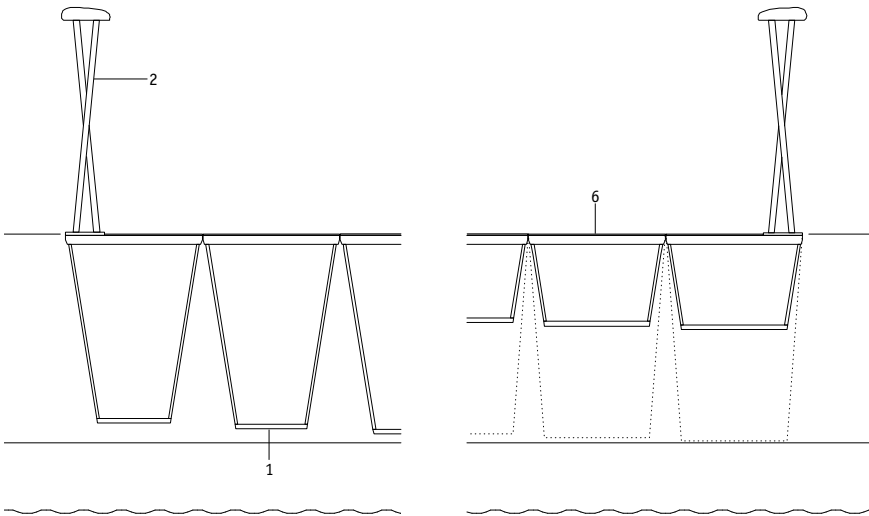
Cross section through the bridge balustrade near the pivot and near the tip, 1:40
