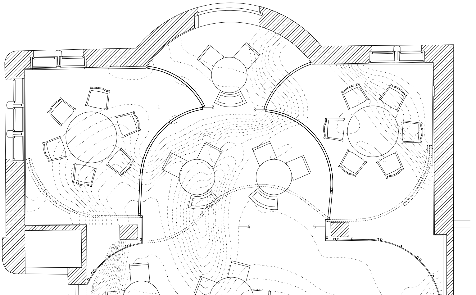
Floor plan of the existing restaurant interior, 1:65
