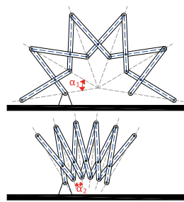
Polar planar scissor linkage
