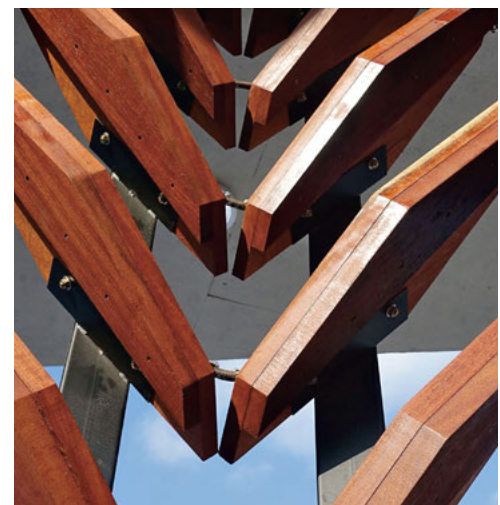
Element anchor and elastic connection
