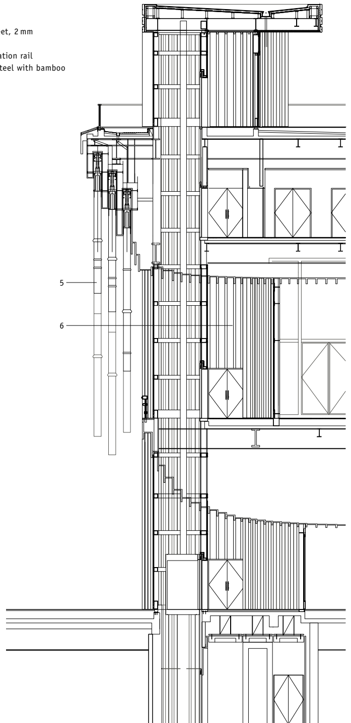
Section through facade, 1:200
