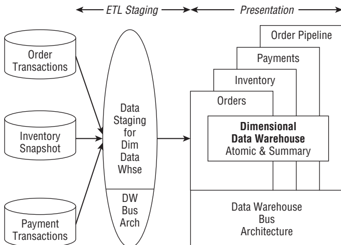
Figure 5-9: Dimensional data warehouse.
