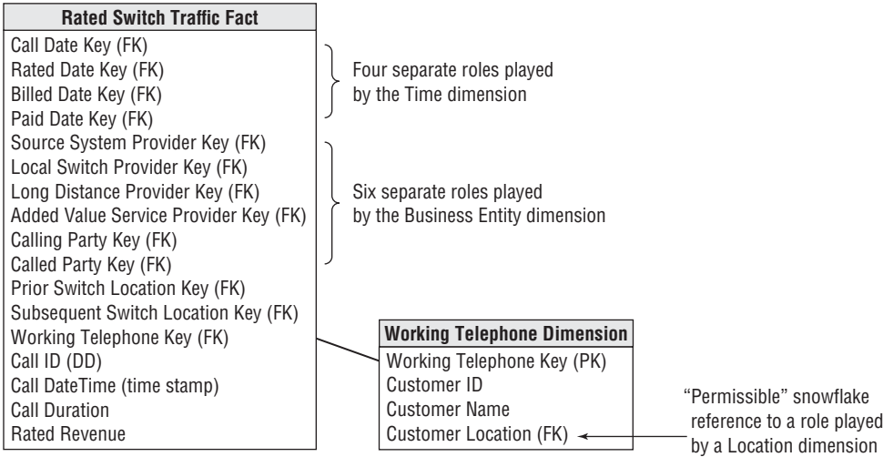
Figure 9-10: Sample schema with extensive role playing.
