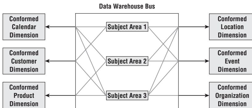
Figure 2-4: The data warehouse bus architecture, showing a series of data marts connecting to the conformed dimensions of the enterprise.
