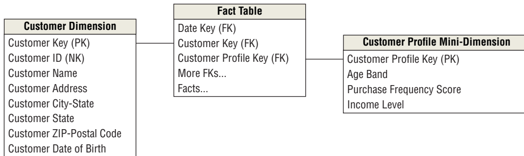
Figure 9-19: Add a mini-dimension to make SCD type 4.
