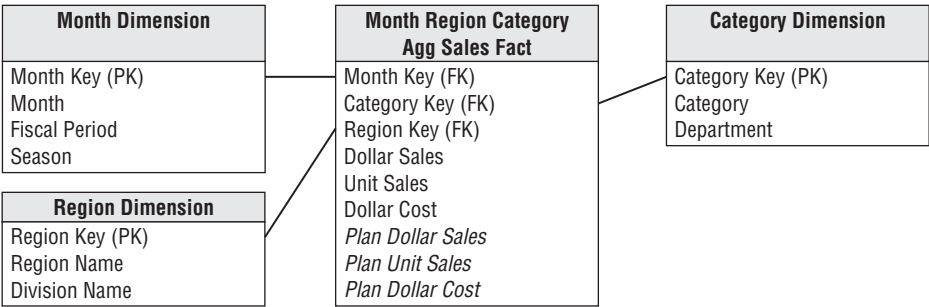
Figure 12-13: The three-way aggregate table formed by aggregating time to month, product to category, and store to region.
