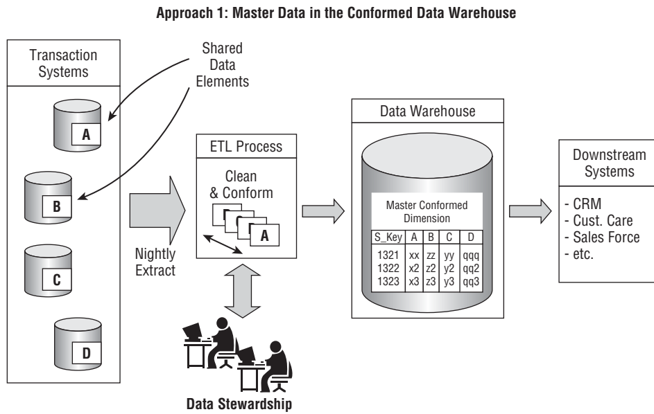
Figure 12-1: Approach 1: Managing master data in the data warehouse ETL.
