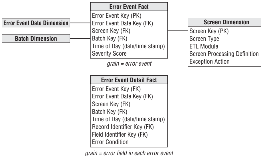
Figure 11-5: The error event schema.
