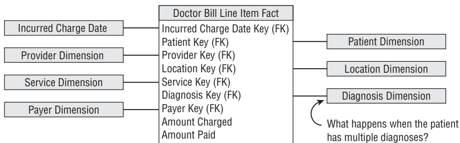
Figure 10-10: A healthcare billing fact table.
