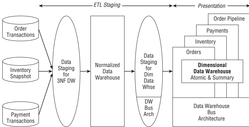
Figure 5-11: Hybrid of normalized data warehouse and dimensional data warehouse.
