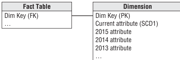
Figure 9-18: A dimension table with a series of type 3 attributes to track predictable changes.
