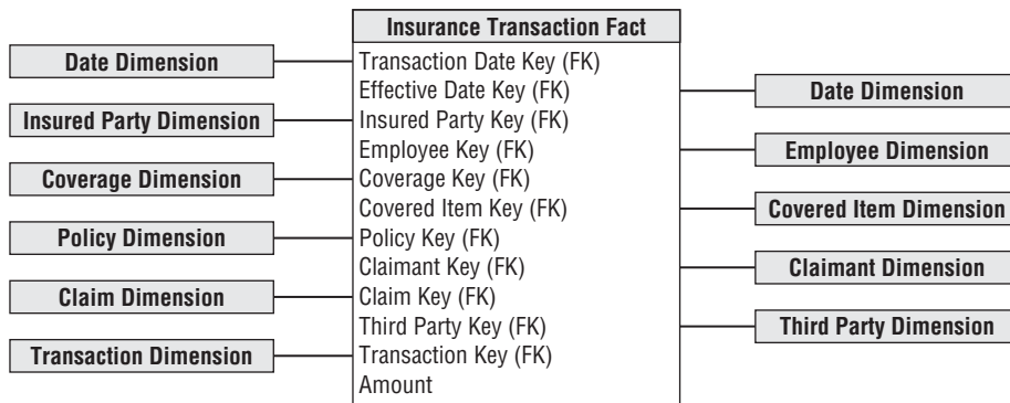
Figure 10-39: A claims transaction dimensional model.
