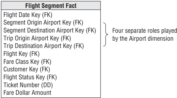
Figure 9-8: Multiple airports on a flight segment fact table.
