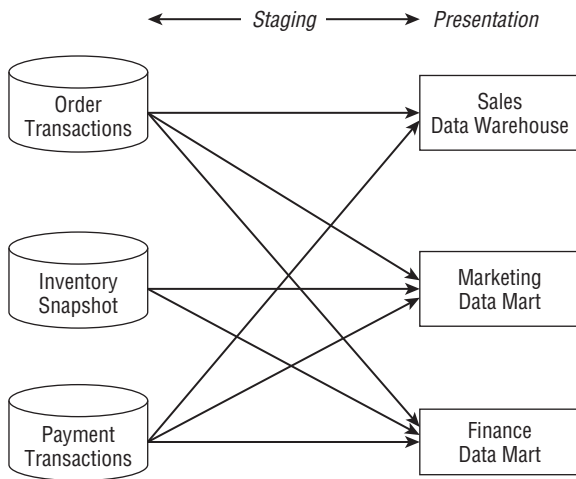
Figure 5-8: Independent data marts/warehouses.
