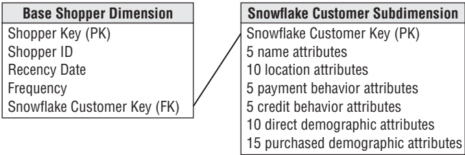
Figure 10-6: A shopper dimension with a snowflake for customer attributes.
