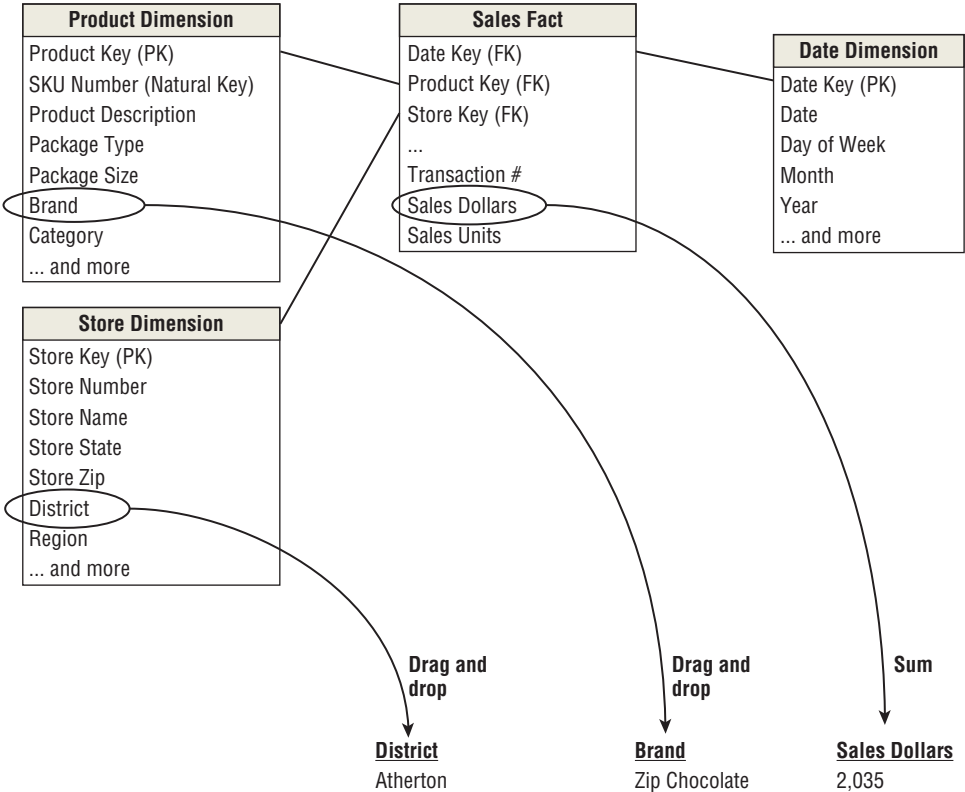
Figure 6-2: Dragging dimension attributes and facts into a report.
