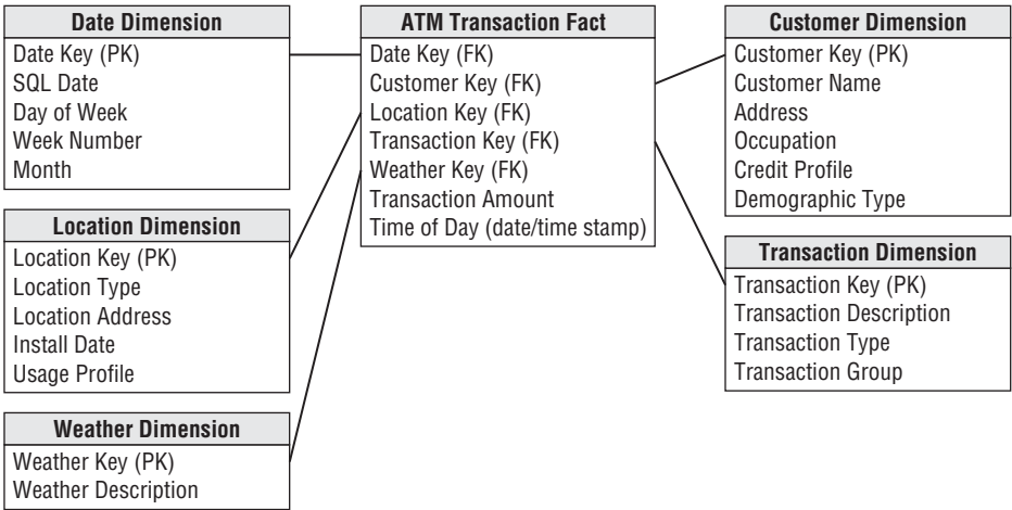
Figure 10-9: A typical dimensional model for ATM transactions.
