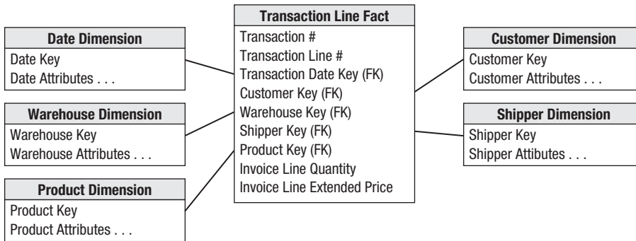
Figure 8-9: Recommended structure for modeling header/line item transactions.
