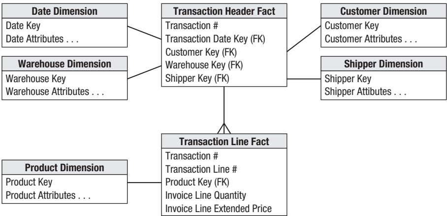
Figure 8-8: Bad idea #2—None of the header dimensionality is directly joined to the line items.
