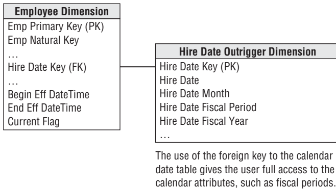
Figure 10-2: A date dimension outrigger joined to the employee dimension.
