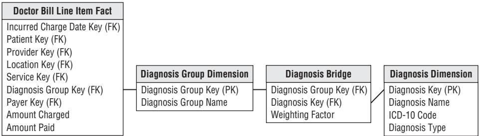
Figure 10-11: A bridge table to handle multiple diagnoses.
