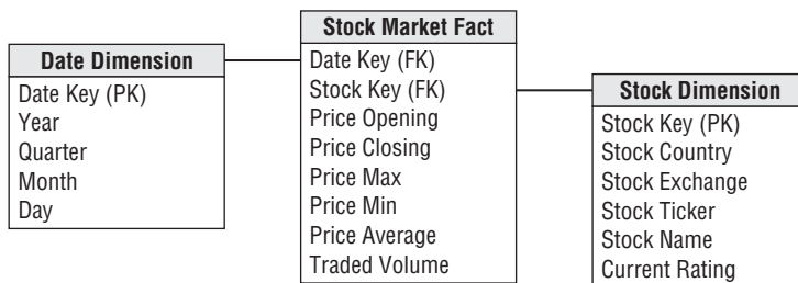
Figure 13-14: A sample schema with stock prices.
