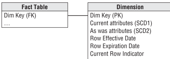
Figure 9-16: Tracking both “as was” and current profile attributes in a single dimension table.
