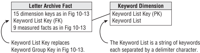
Figure 10-14: The same fact table showing the keyword dimension containing a variable-length text string keyword list.
