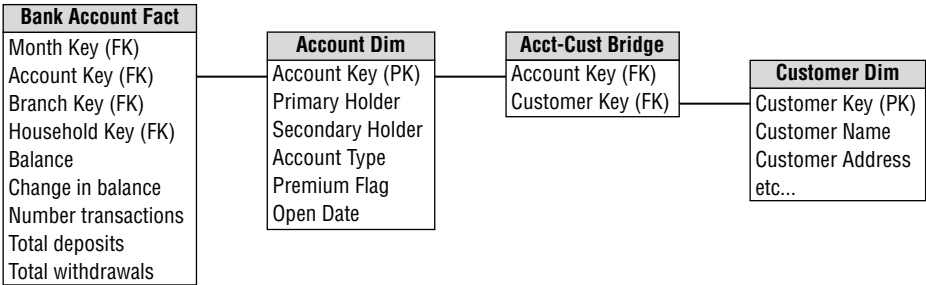
Figure 10-18: The account-to-customer bridge table without the mini-dimension.
