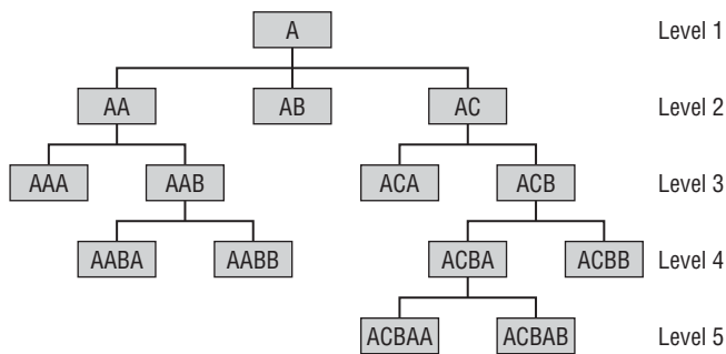
Figure 10-31: Sample org chart with pathstring values.
