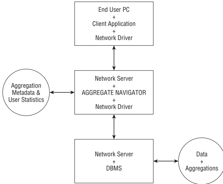
Figure 12-8: The aggregate navigator sits between the user application and DBMS.
