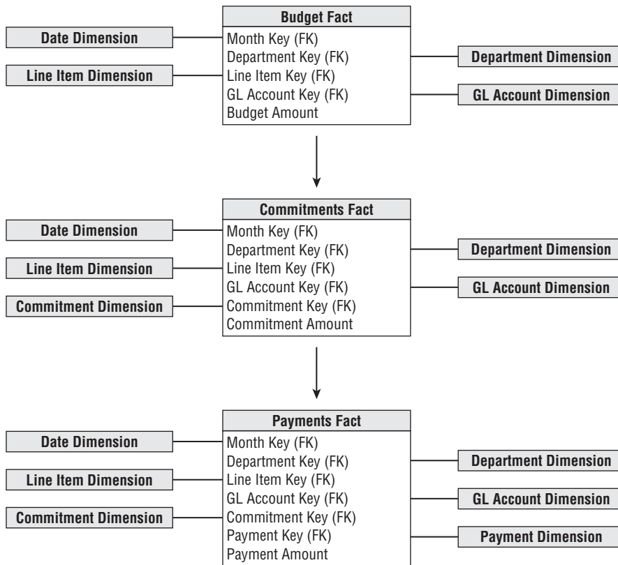
Figure 10-46: The budget chain showing the budget, commitments, and payments fact tables.
