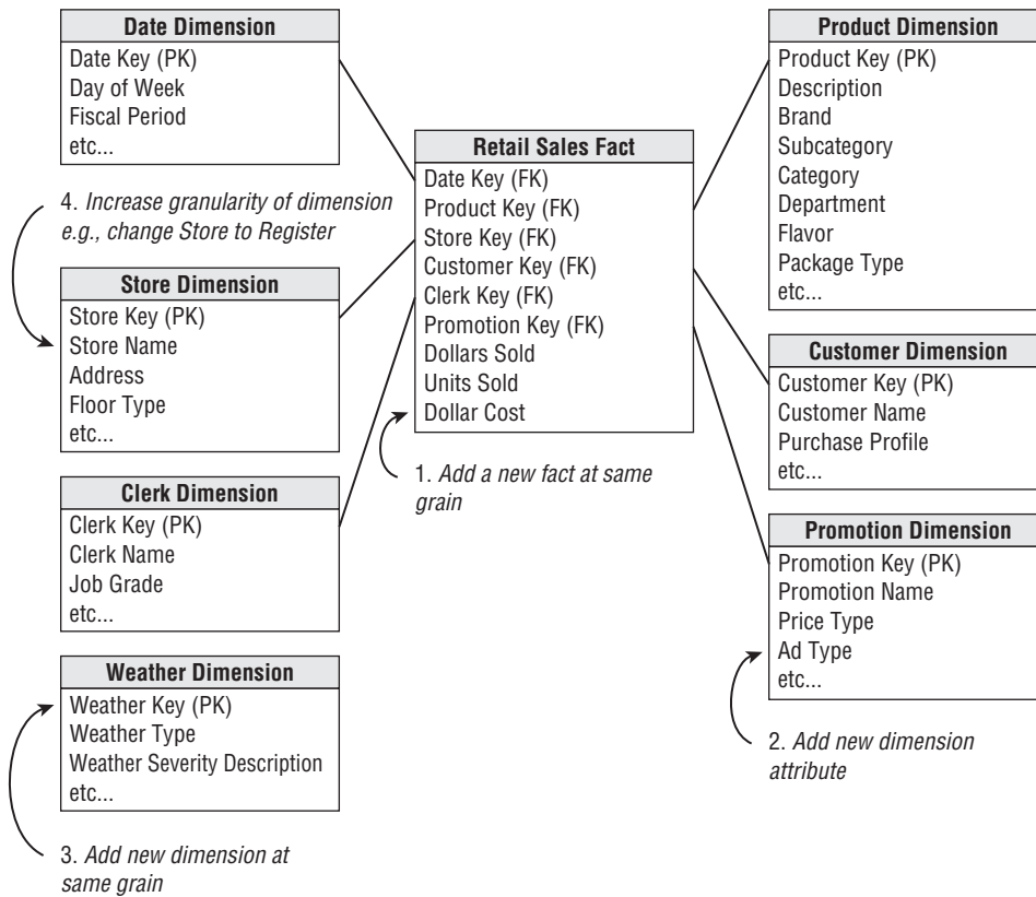
Figure 5-4: A detailed dimensional model for retail point of sales. Numbers 1 through 4 show places where the design may be gracefully extended.
