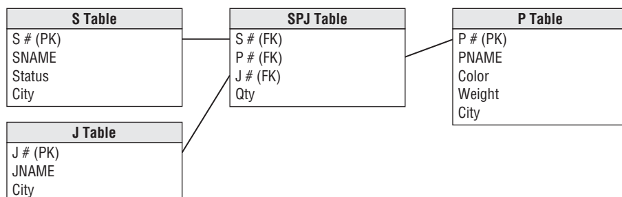
Figure 5-5: The suppliers and parts database.
