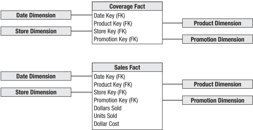
Figure 8-6: Factless coverage fact table for promotion events.
