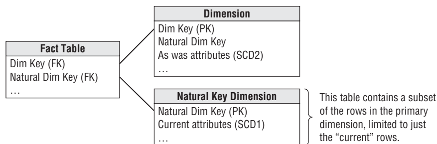
Figure 9-17: One foreign key in the fact table joins to a SCD2 dimension table, while the natural/durable key joins to only the most current version of the dimension.
