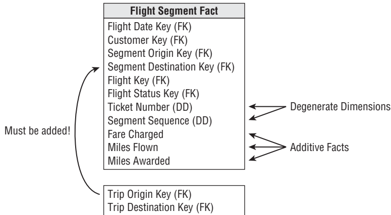
Figure 10-43: The flight segment dimensional model.
