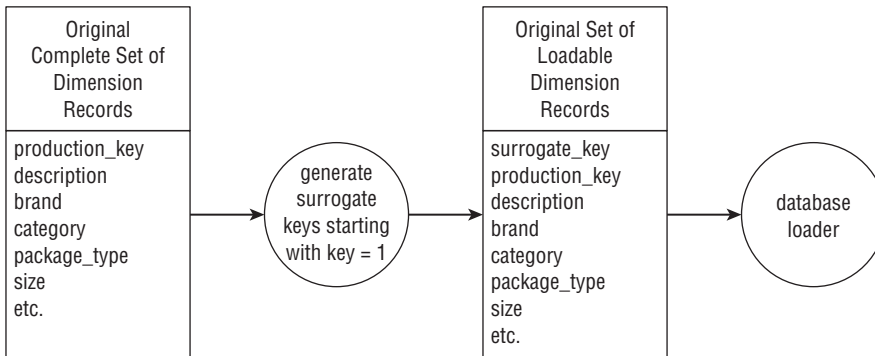
Figure 11-13: The original loading of a dimension where surrogate keys are assigned sequentially to every input record and the natural key becomes an ordinary attribute.
