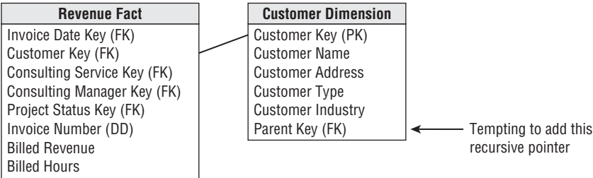
Figure 10-23: A fact table whose grain is the individual invoice line item.
