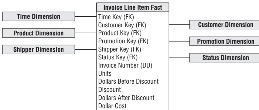
Figure 7-1: Customer invoice line item fact table.
