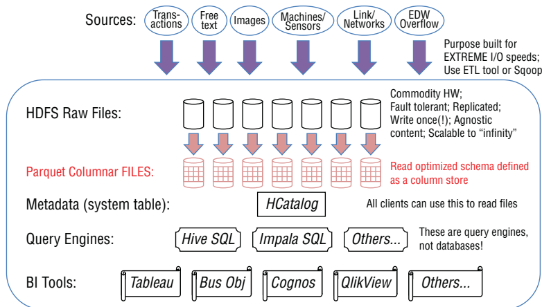
Figure 12-6: HDFS viewed as a data warehouse environment.
