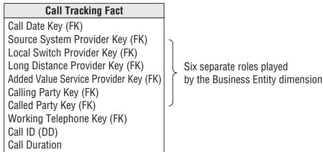
Figure 9-9: Multiple business entities associated with a phone call.
