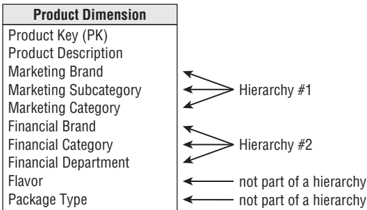
Figure 6-3: A product dimension table with both marketing and finance attributes.
