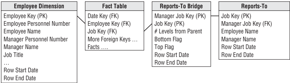
Figure 10-28: Separate employee and reports-to (or job) dimensions.
