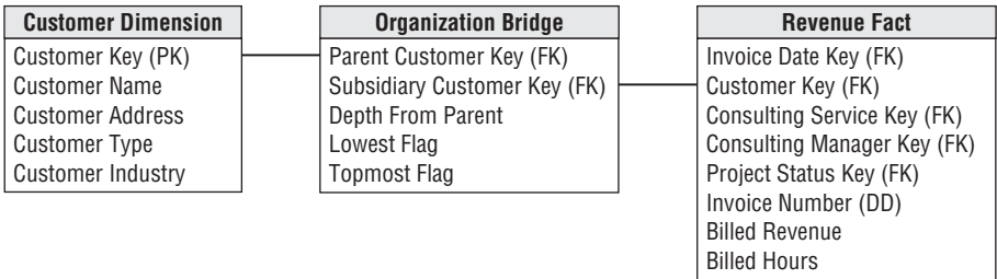
Figure 10-25: A bridge table between the fact and dimension table to navigate the organizational hierarchy.
