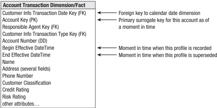
Figure 8-10: Fact table to capture customer information changes.
