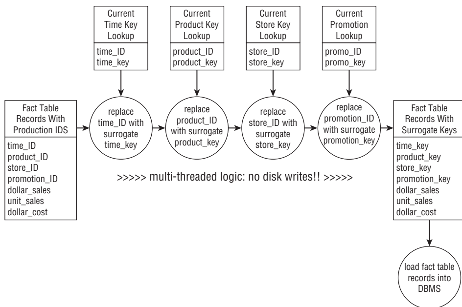
Figure 11-16: The pipelined fact table processing logic for replacing all natural keys (designated as IDs) with surrogate keys.
