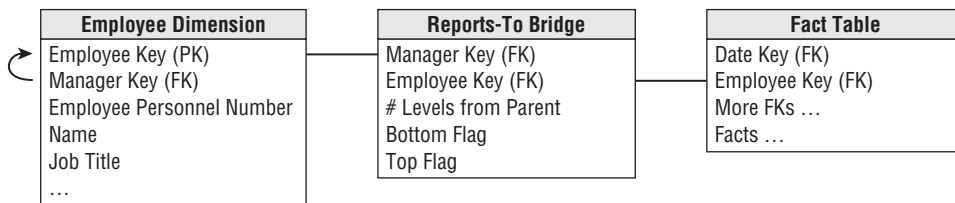
Figure 10-27: Classic relational structure for a reports-to hierarchy.
