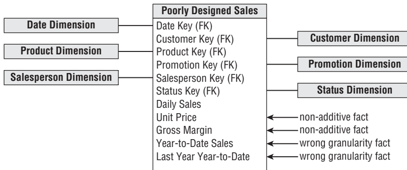
Figure 7-3: An example of a “bad” fact table.
