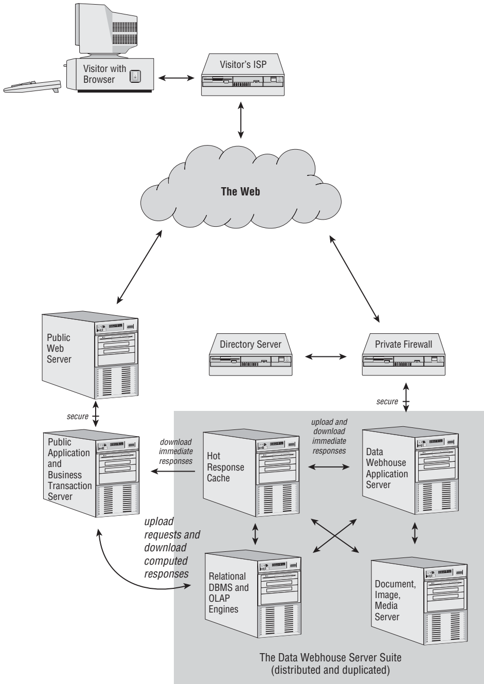
Figure 11-21: The web-intensive data warehouse architecture, showing the hot response cache and the application server that creates its contents.
