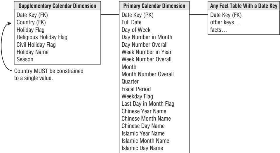
Figure 10-37: Primary and supplementary calendar dimensions for organizations that must track multiple national calendars.
