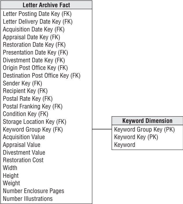
Figure 10-13: The fact table for a letter archive data warehouse showing the keyword bridge dimension table.
