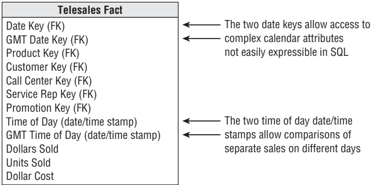
Figure 10-36: A typical fact table recording sales made in different time zones, with GMT as the absolute time stamp.
