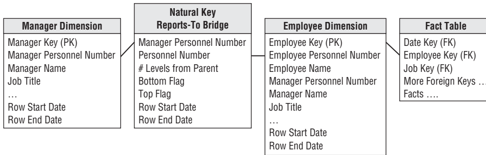
Figure 10-29: Tracking history in the reports-to relationship with a natural key bridge table.
