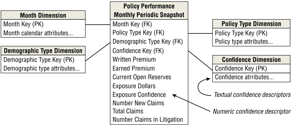
Figure 11-8: An insurance fact table augmented with an exposure confidence fact and uncertainty dimension.
