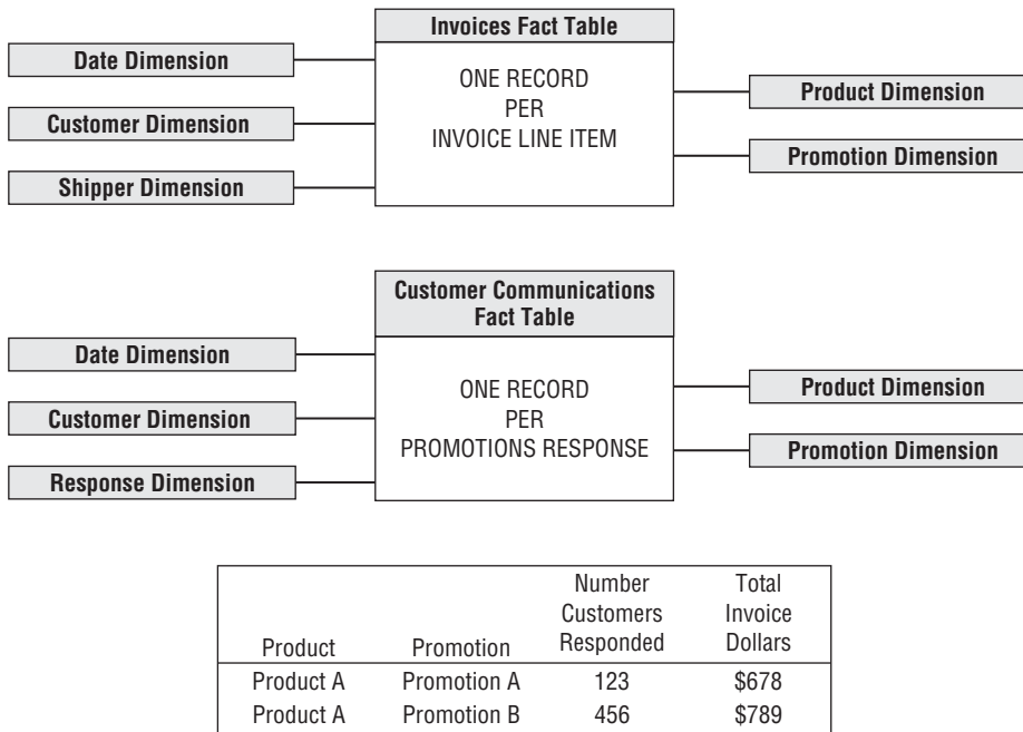
Figure 7-2: Two subject areas with conformed dimensions.
