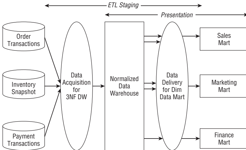
Figure 5-10: Normalized data warehouse with departmental data marts.
