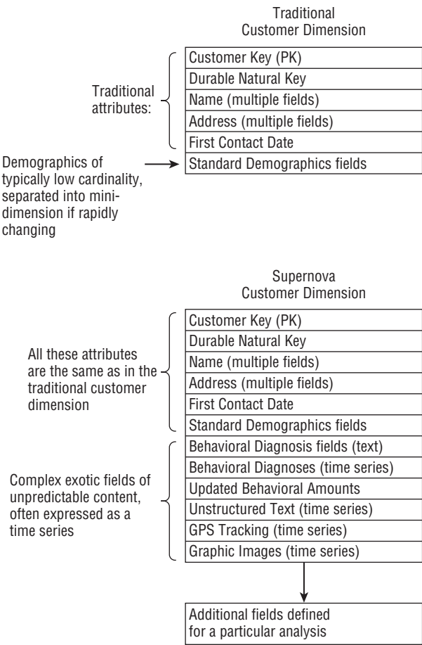
Figure 15-1: Traditional and Supernova Customer Dimensions.
