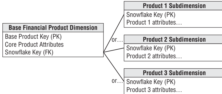
Figure 10-7: A financial product dimension with a subdimension for each product type.
