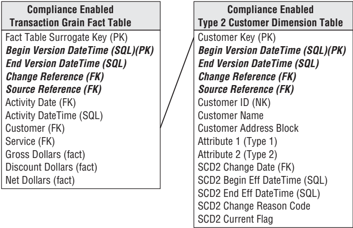
Figure 10-47: Compliance-enabled fact and dimension tables.
