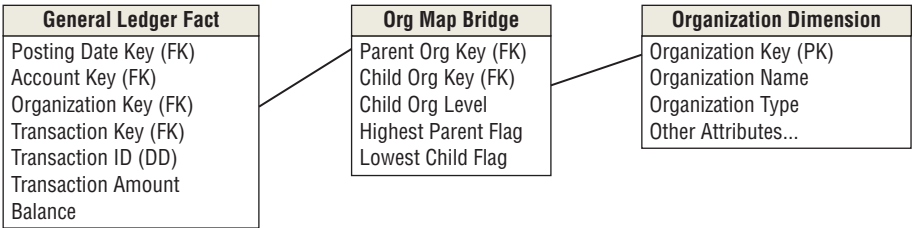
Figure 10-4: A bridge table models a hierarchical variable-depth relationship.
