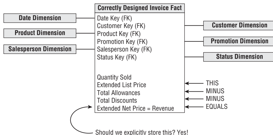
Figure 7-5: A customer billing fact table.
