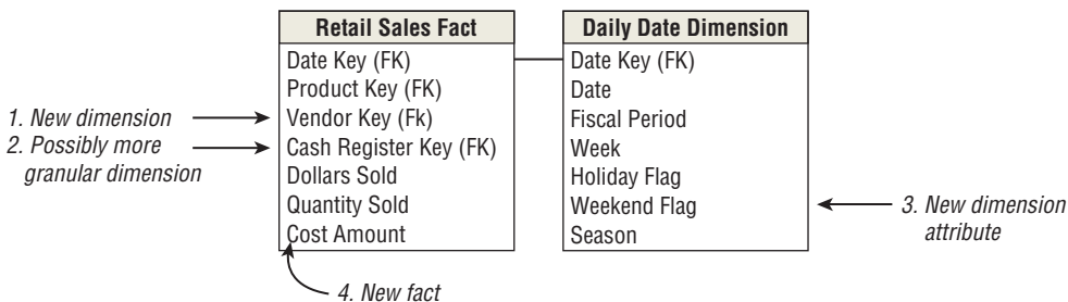
Figure 6-6: Potential changes to an existing dimensional model.
