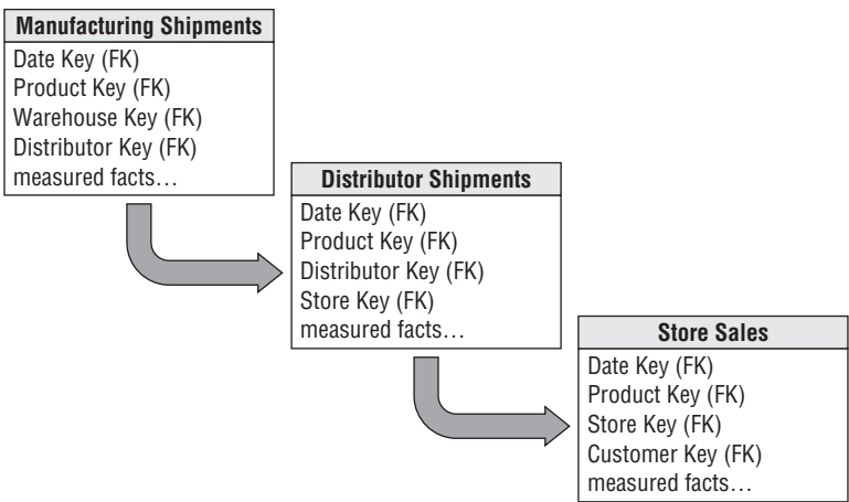
Figure 10-45: This value chain represents a product flow where each process is a fact table.
