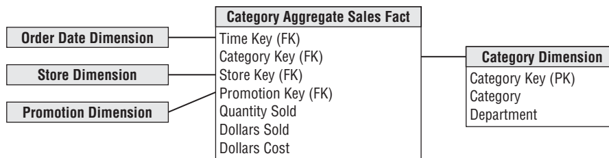
Figure 12-10: Aggregate records stored in separate fact and shrunken dimension tables is recommended.
