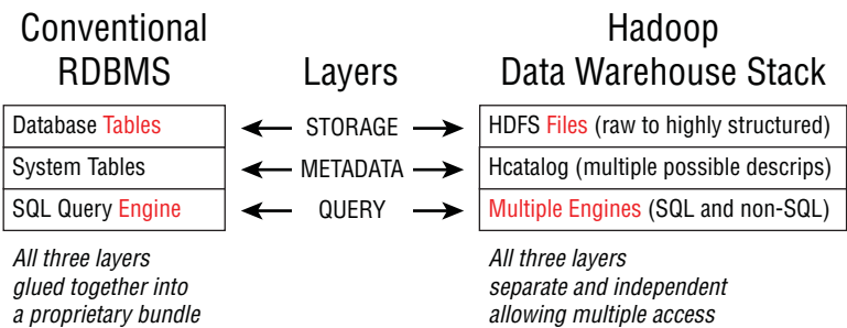
Figure 12-5: Comparison of the storage, metadata, and query layers between conventional RDBMSs and the Hadoop data warehouse stack.
