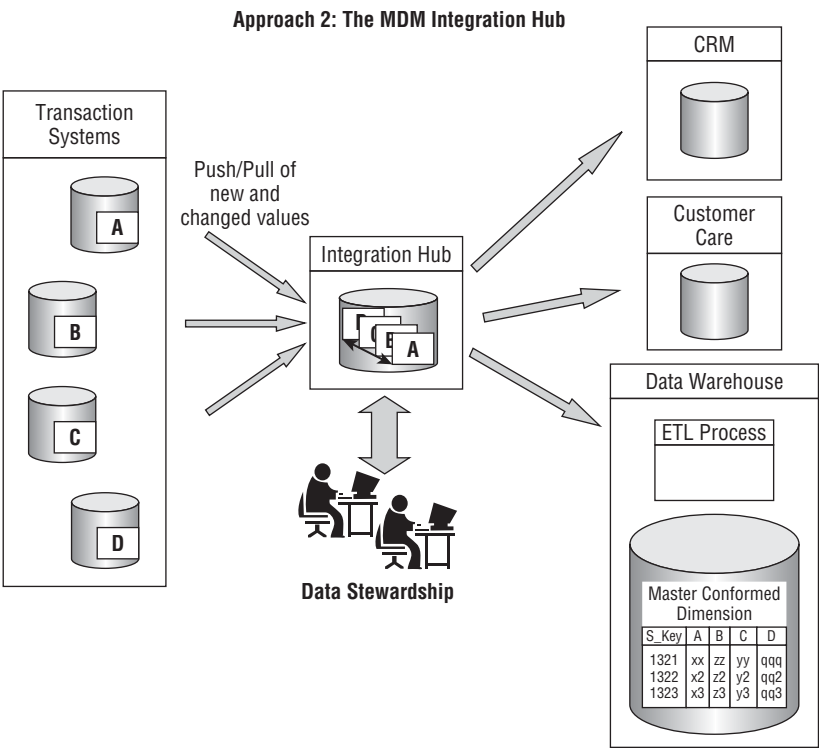
Figure 12-2: Approach 2: Implementing MDM via an integration hub.
