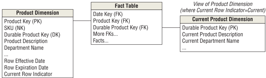
Figure 9-22: Add dual type 1 and type 2 dimensions to make SCD type 7.
