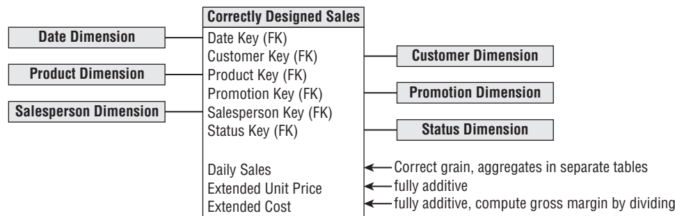
Figure 7-4: An example of a “good” fact table addressing the issues in Figure 7-3.
