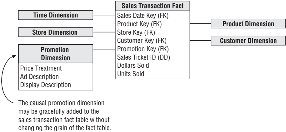
Figure 9-12: A typical dimensional schema for a set of retail sales transactions with a “causal” promotion dimension.
