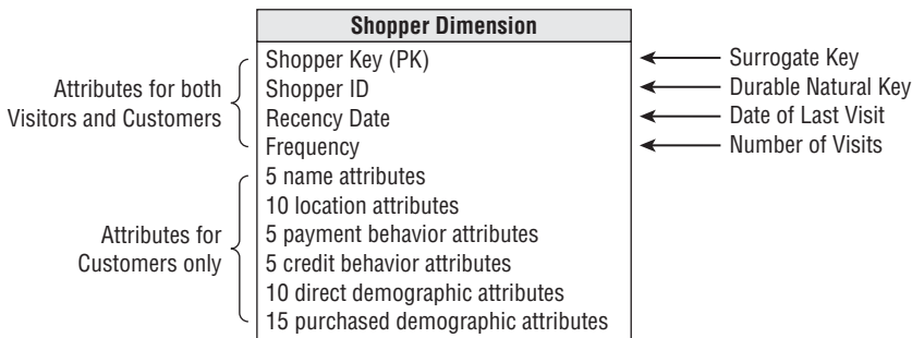
Figure 10-5: Shopper dimension with both visitor and customer attributes.
