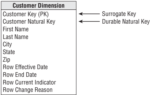
Figure 9-24: Customer dimension table with type 2 administration control columns.
