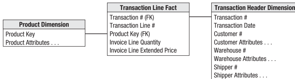
Figure 8-7: Bad idea #1—The transaction header is a dimension table.
