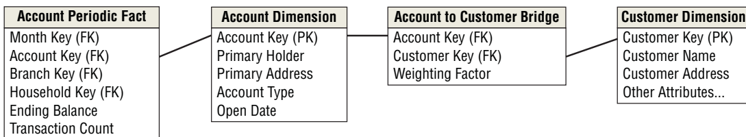
Figure 10-3: A bridge table resolves a many-valued dimension attribute.
