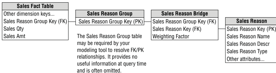
Figure 10-16: A sales fact table capturing multiple sales reasons.
