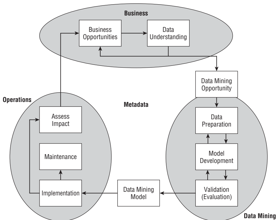
Figure 13-4: The overall data mining process.
