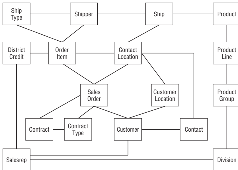
Figure 5-3: A high level 3NF model.
