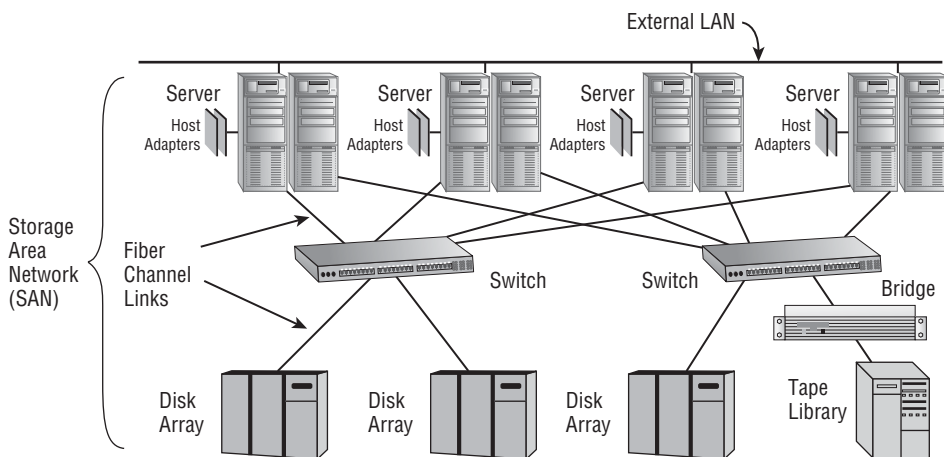
Figure 12-14: A typical storage area network configuration.
