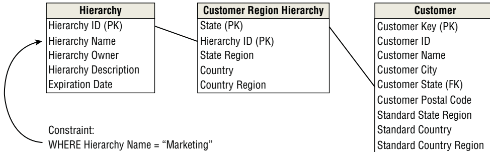
Figure 10-32: Using a bridge table to support multiple alternate hierarchies.
