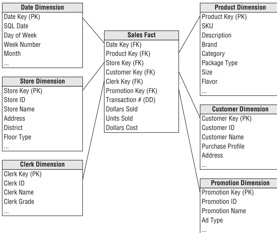
Figure 9-1: A sample data warehouse schema.
