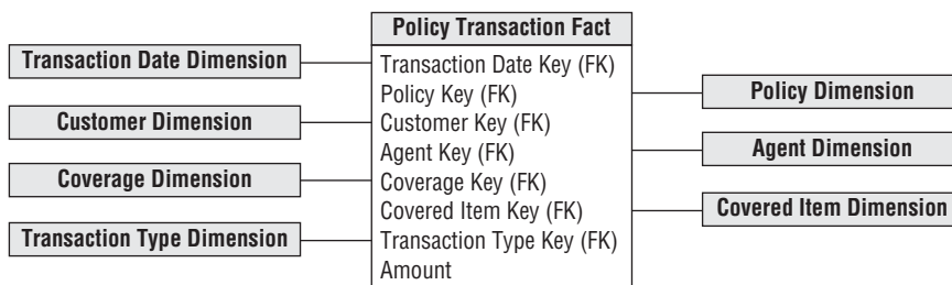
Figure 8-2: A transaction-grained insurance fact table.
