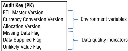
Figure 11-9: A simple audit dimension.
