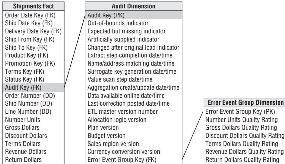
Figure 11-6: A sample audit dimension attached to a shipments invoice fact table.
