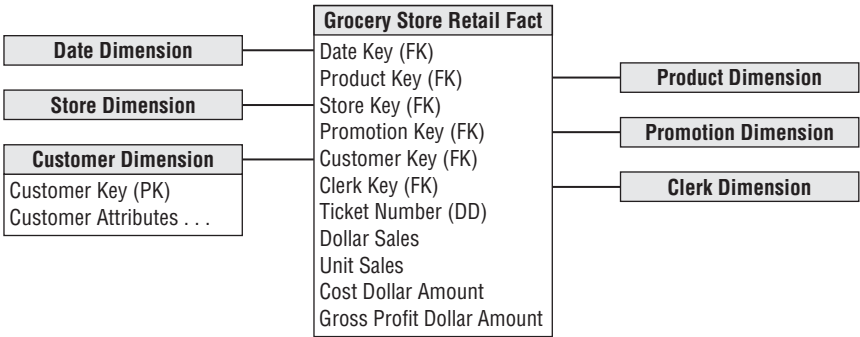
Figure 6-1: A dimensional model for grocery store sales.
