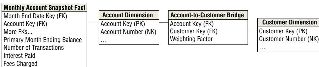
Figure 10-15: A banking example showing an account-to-customer bridge table.
