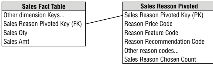
Figure 10-17: Multiple sales reasons modeled as a pivoted sales reason dimension.
