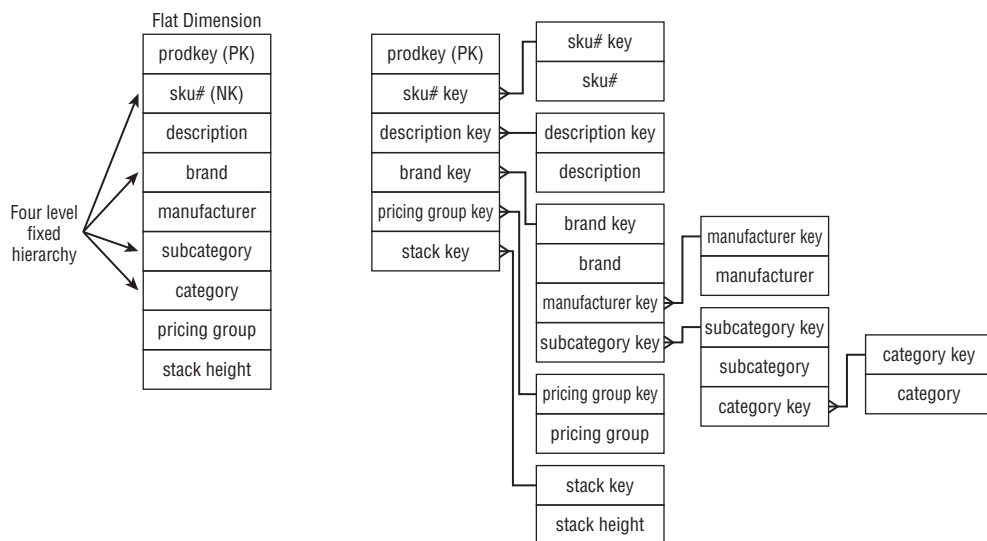
Figure 10-1: Denormalized and snowflaked versions of the same dimension table.
