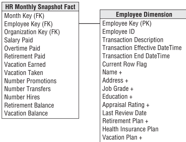
Figure 10-44: A human resources monthly snapshot with a type 2 slowly changing employee dimension table.
