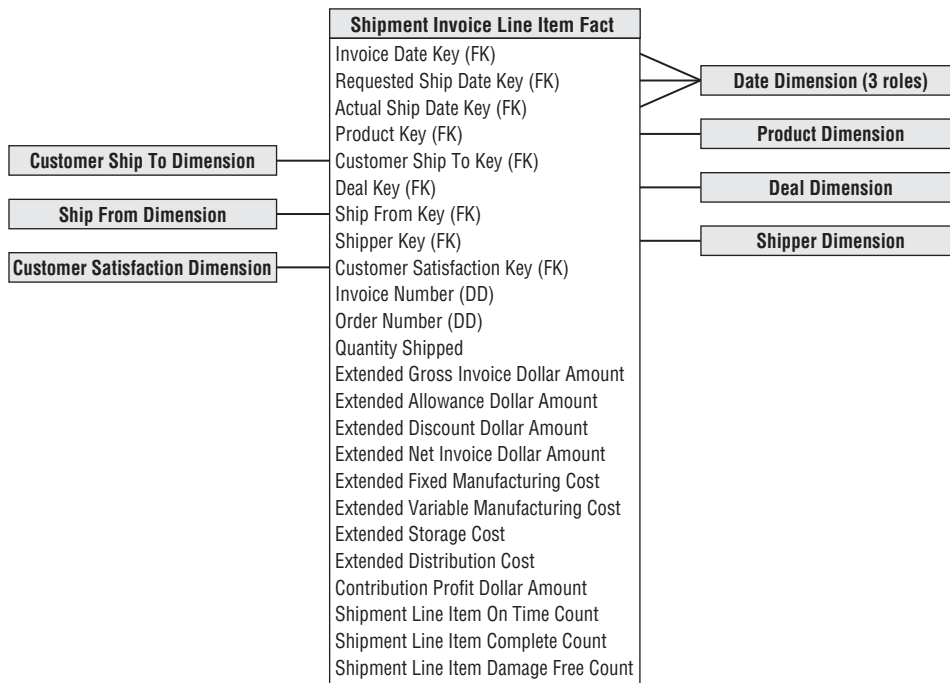
Figure 10-33: Treating satisfaction metrics as facts.
