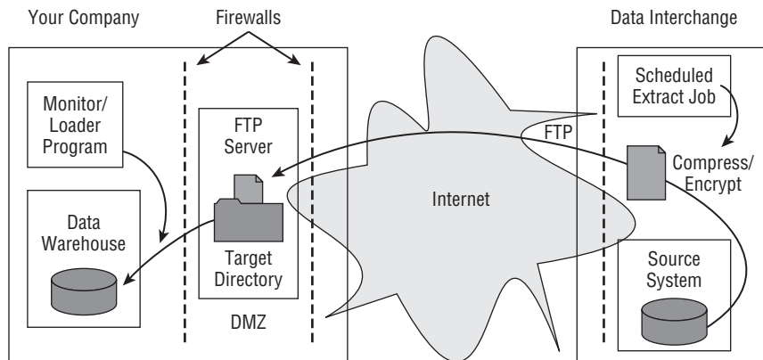
Figure 11-4: Typical architecture to support FTP-based integration.
