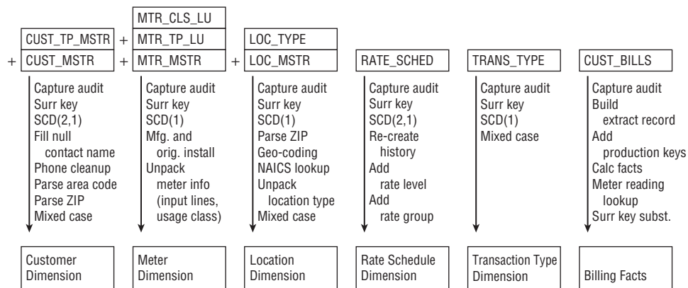
Figure 11-1: Simplified conceptual ETL plan.
