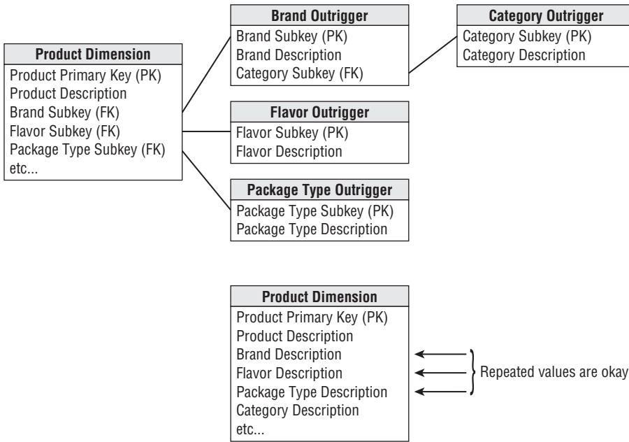
Figure 5-2: Two representations of a product dimension—the top snowflaked version is normalized to 3NF, and the bottom is denormalized into a flat dimension.
