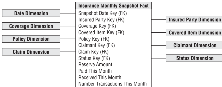
Figure 10-40: A claims monthly snapshot dimensional model.
