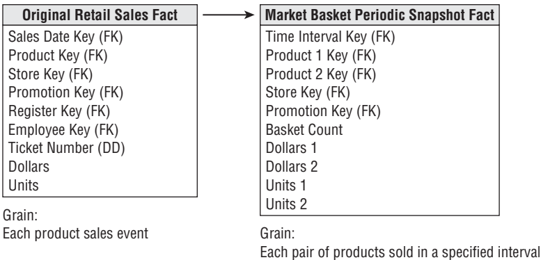
Figure 10-49: A market basket fact table based on atomic retail sales data.
