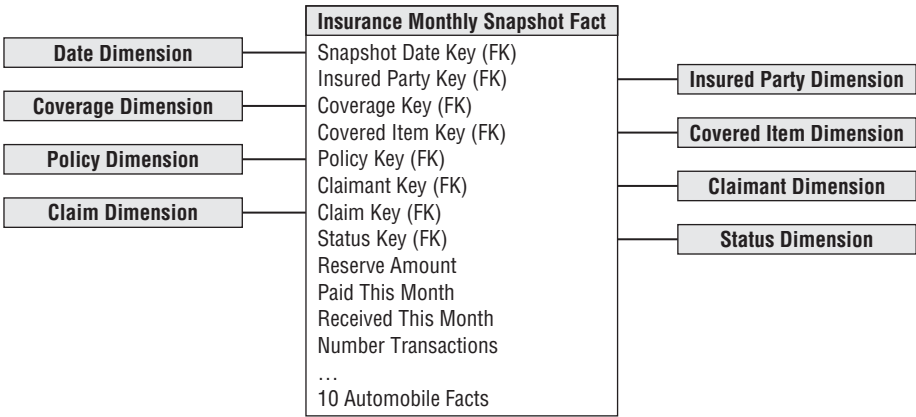
Figure 10-42: Monthly snapshot for automobile coverages.
