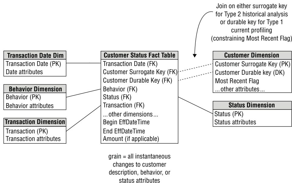
Figure 10-35: Design for real-time customer status tracking with historical and current perspectives.
