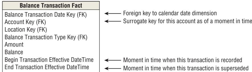
Figure 8-11: Balance transactions that reference the account surrogate key.
