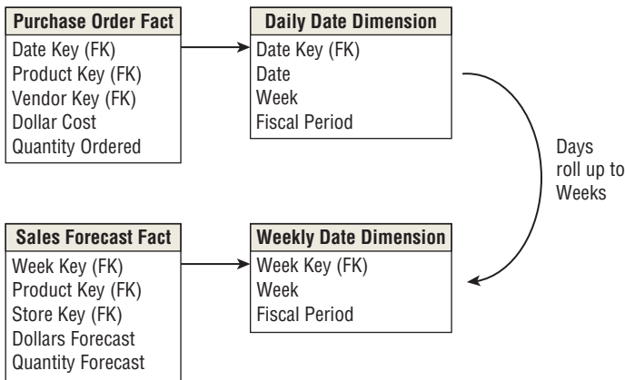
Figure 6-5: Two fact tables with conformed dimensions.
