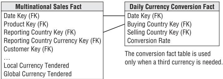
Figure 10-38: A fact table simultaneously recording sales in many different currencies. The currency conversion table is only used when converting to a third currency.
