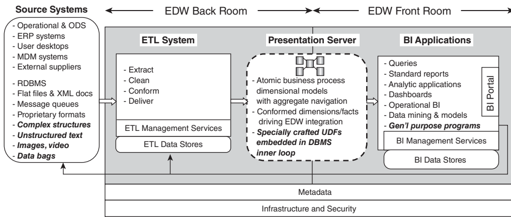
Figure 12-4: The extended RDBMS-based architecture for an enterprise data warehouse.
