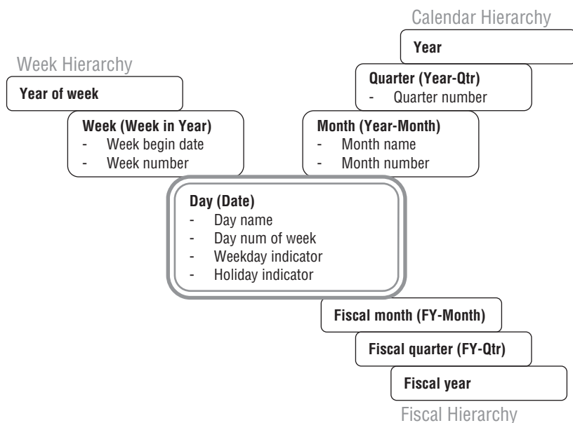
Figure 10-20: Graphical representation of multiple date hierarchies.
