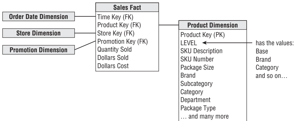
Figure 12-9: Aggregate records identified by the level attributes, which is not recommended.
