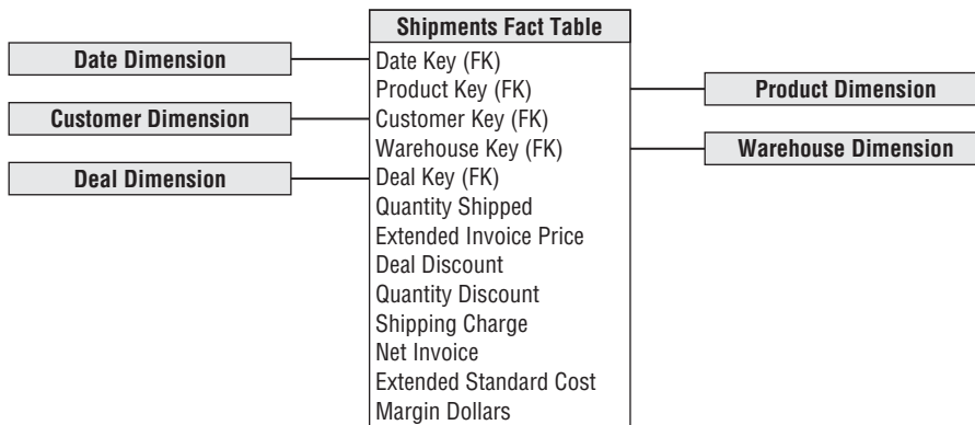
Figure 2-1: Dimensional schema example.
