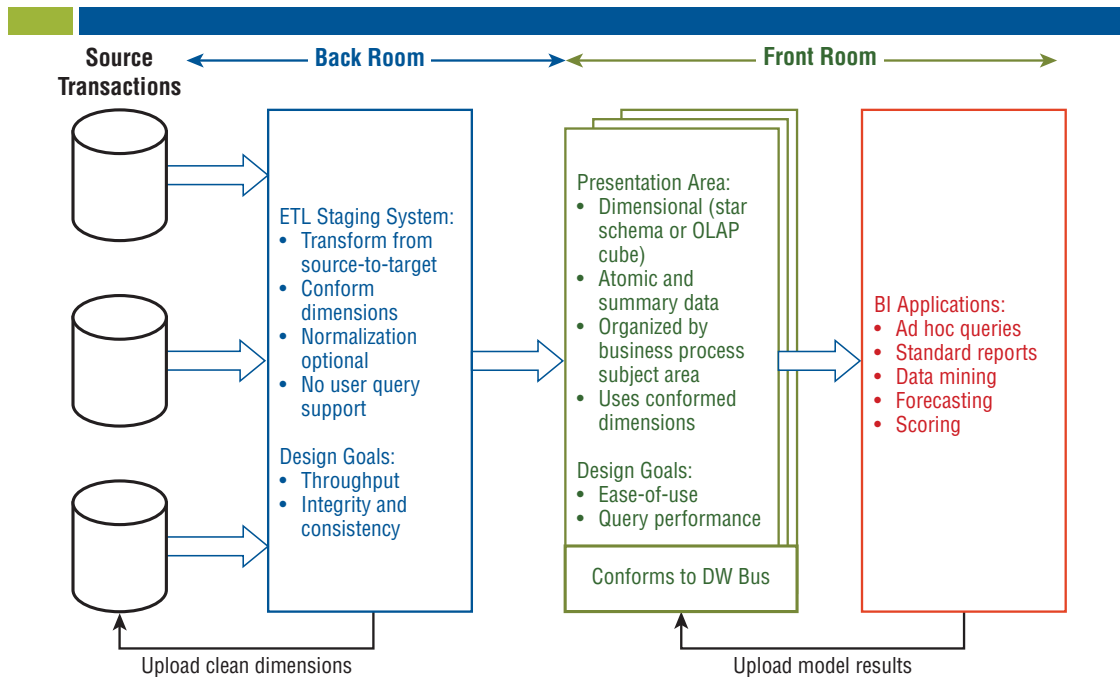
Figure 2-3: The enterprise data warehouse, showing the back room ETL staging area and the front room presentation area.
