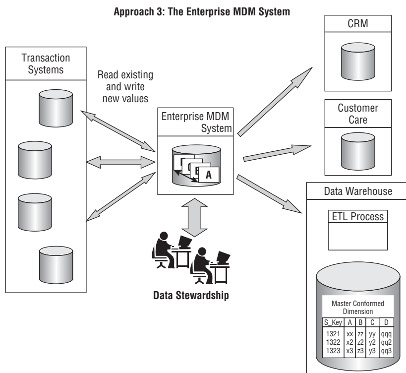
Figure 12-3: Approach 3: The enterprise MDM system.
