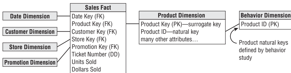
Figure 13-13: A special behavior dimension is added to a normal dimensional model to restrict the schema to the context of a behaviorally defined group of products.
