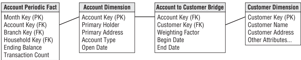
Figure 10-12: Resolving the relationship of multiple customers associated with an account using a bridge table.
