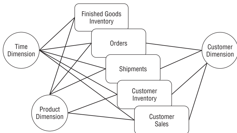
Figure 6-4: Separate fact tables for each business process share common dimensions.
