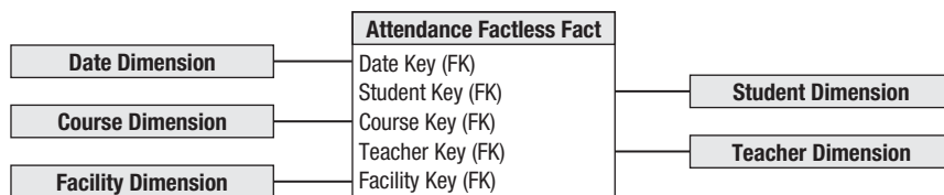
Figure 8-5: Daily student attendance is recorded in a factless fact table.
