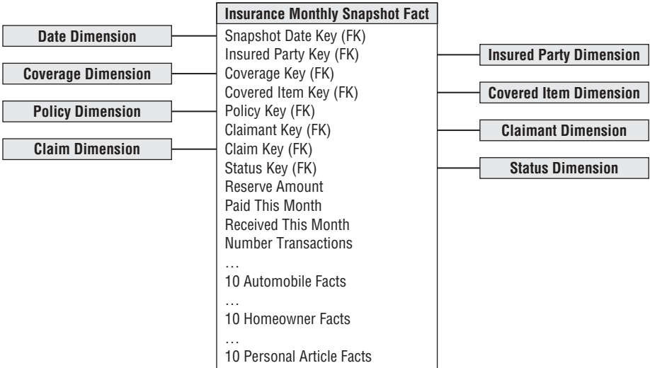
Figure 10-41: Inappropriate way to handle the facts unique to each line of business.
