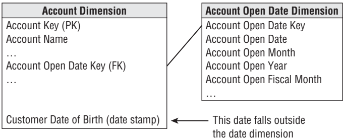
Figure 9-6: A dimension table with a date foreign key, as well as a date stamp attribute.
