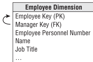
Figure 10-26: Basic structure of the employee dimension and reports-to hierarchy.
