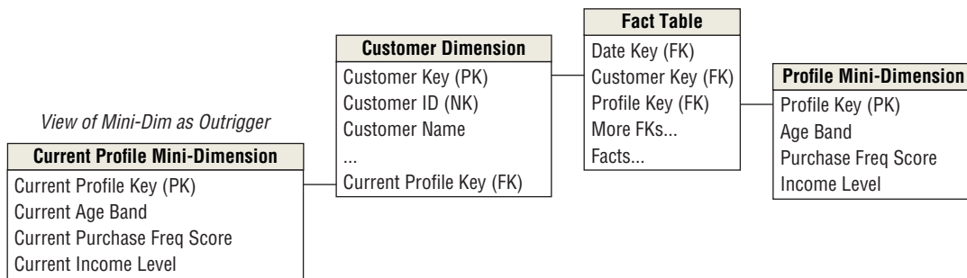
Figure 9-20: Add a mini-dimension and type 1 outrigger to make SCD type 5.
