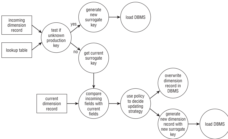
Figure 11-15: Dimension processing logic for all refreshes of a dimension table after the original load.
