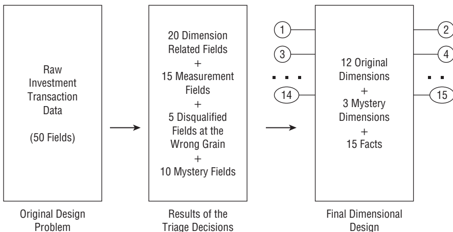
Figure 9-11: The logical progression of transforming complex source data into its corresponding dimensional model.
