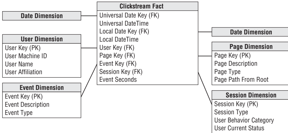
Figure 10-48: The dimensional model for clickstream events.
