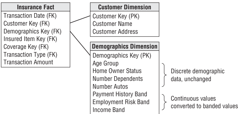
Figure 9-14: Separating frequently changing customer attributes in a demographics mini-dimension.
