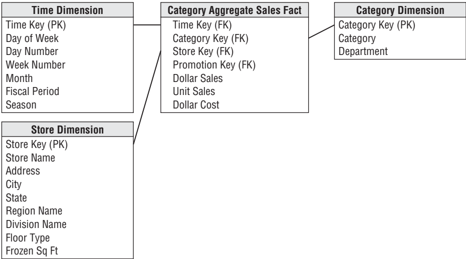
Figure 12-12: An aggregated dimensional schema derived from Figure 12-11 by aggregating to the category level.
