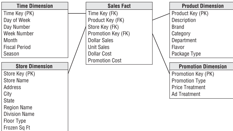
Figure 12-11: A base-level dimensional model.
