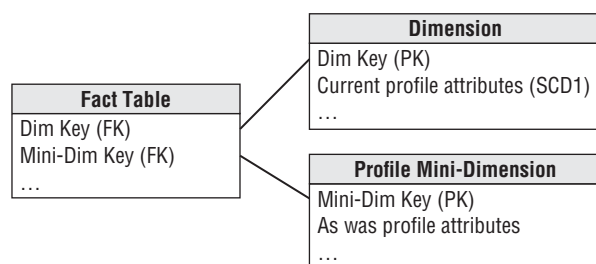
Figure 9-15: A mini-dimension for capturing profile changes with type 1 overwrite in the primary dimension table.
