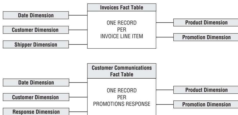
Figure 2-2: Conformed dimensions used by multiple fact tables.
