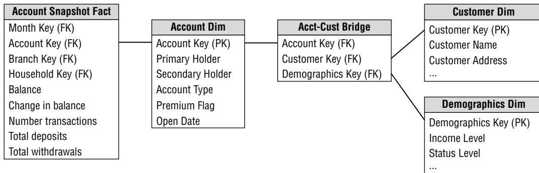
Figure 10-19: The account-to-customer bridge table with the demographics mini-dimension.
