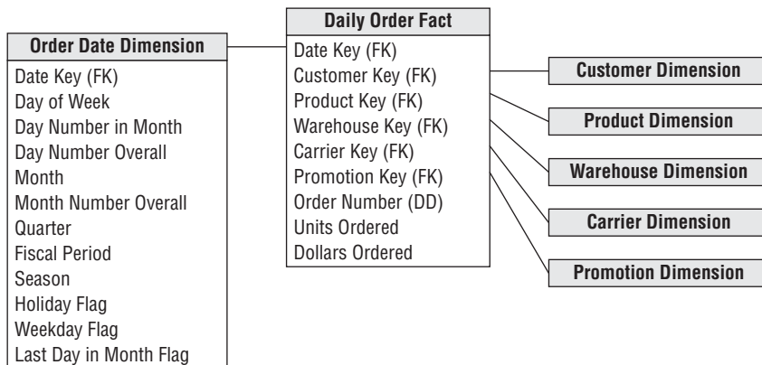
Figure 9-4: A basic dimensional design for order tracking.
