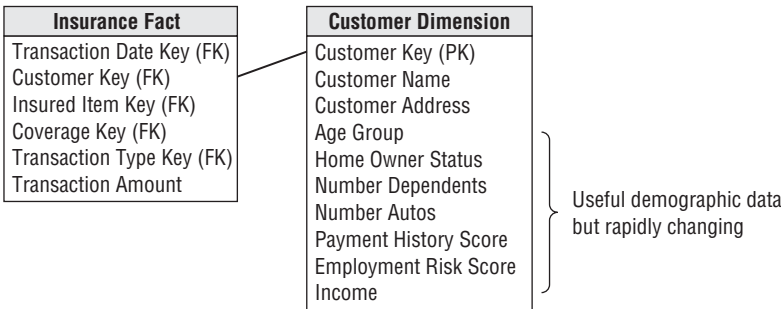
Figure 9-13: Customer dimension with rapidly changing demographic attributes.
