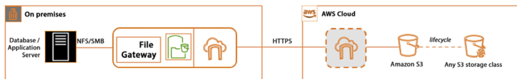
Figure 5.10: Amazon S3 File Gateway
