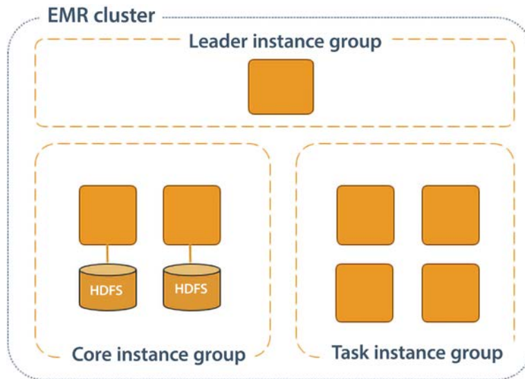
Figure 10.1: Amazon EMR node types
