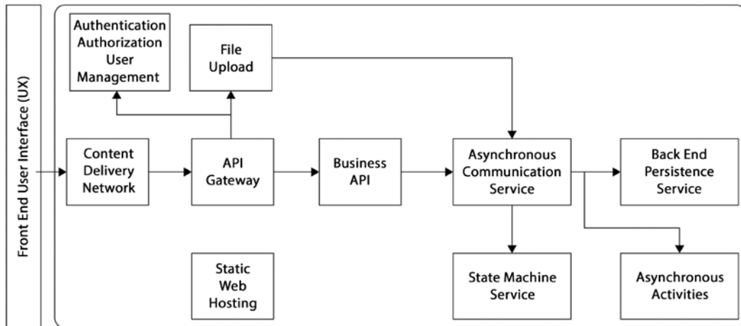
Figure 16.2: Serverless web-application architecture
