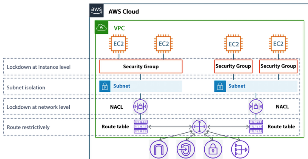
Figure 4.15: SGs and NACLs in network defense
