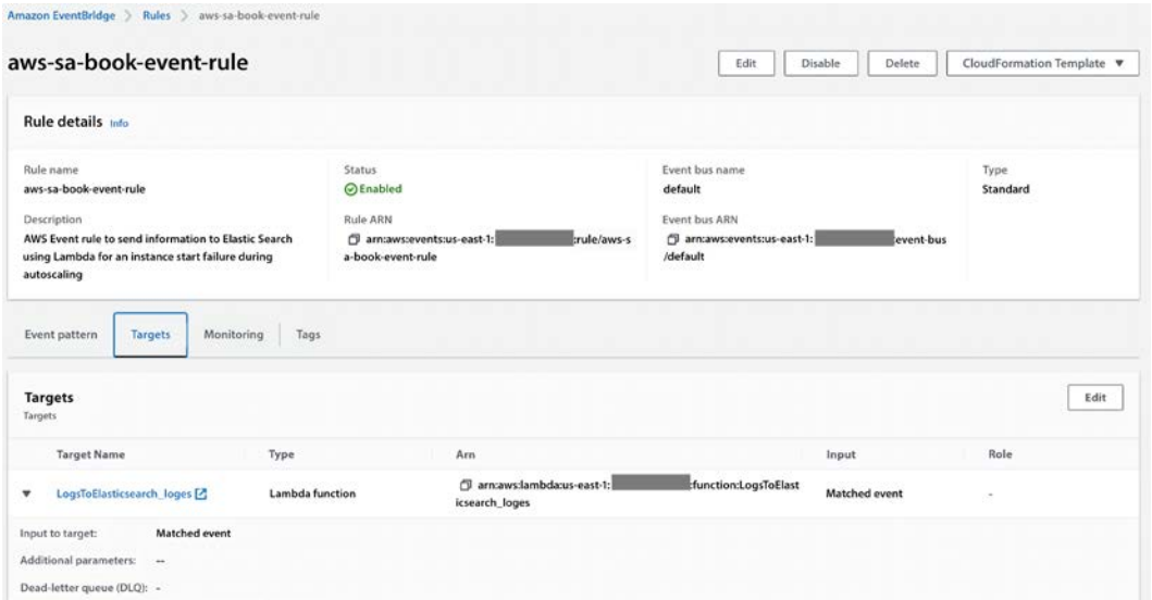
Figure 9.2: An AWS EventBridge rule for an autoscaling failure
