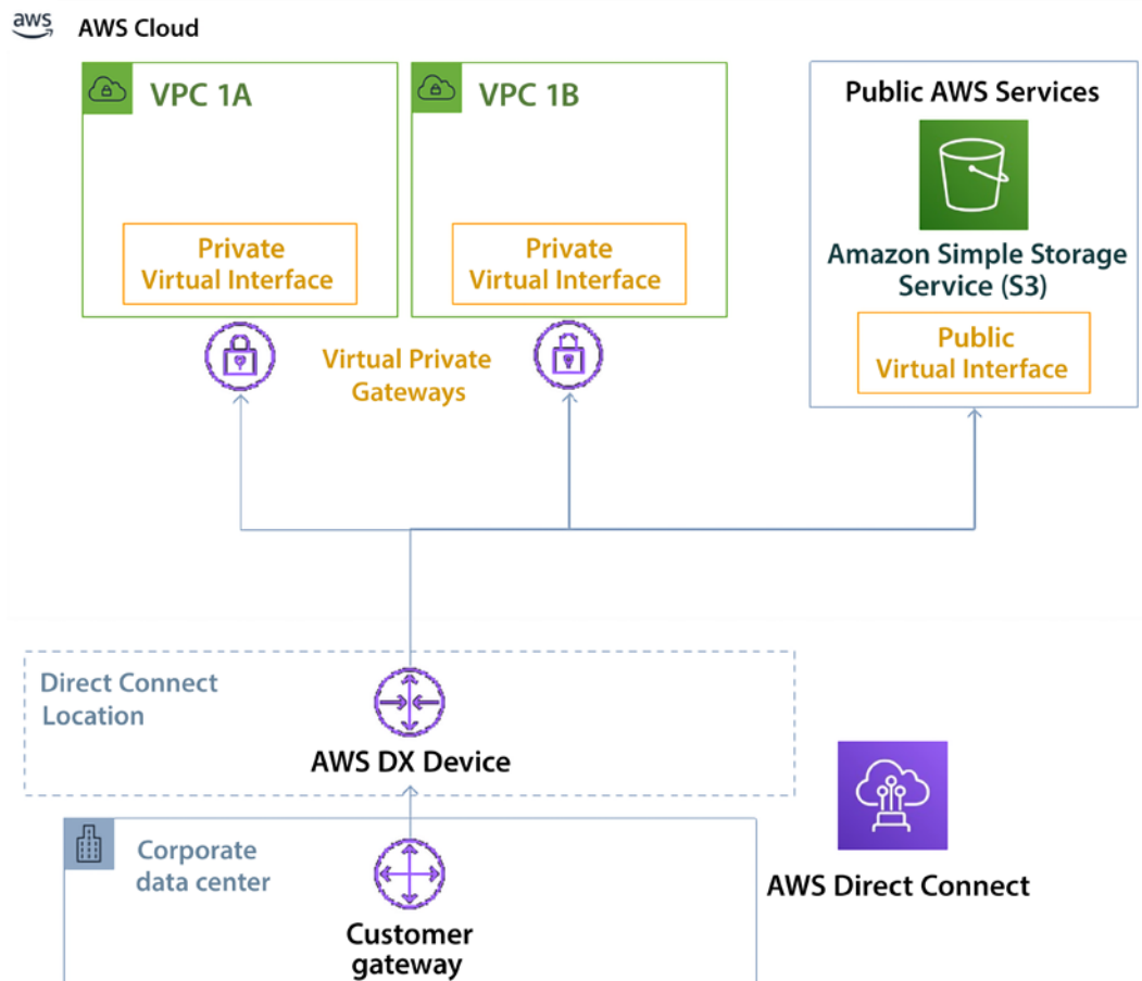
Figure 4.13: AWS Direct Connect interface types
