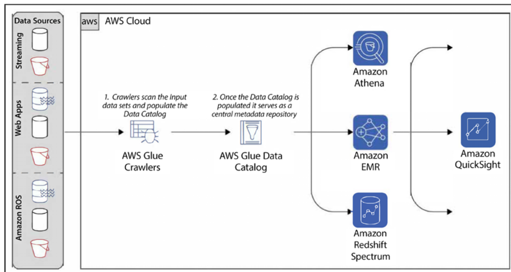
Figure 10.2: AWS Glue typical workflow steps
