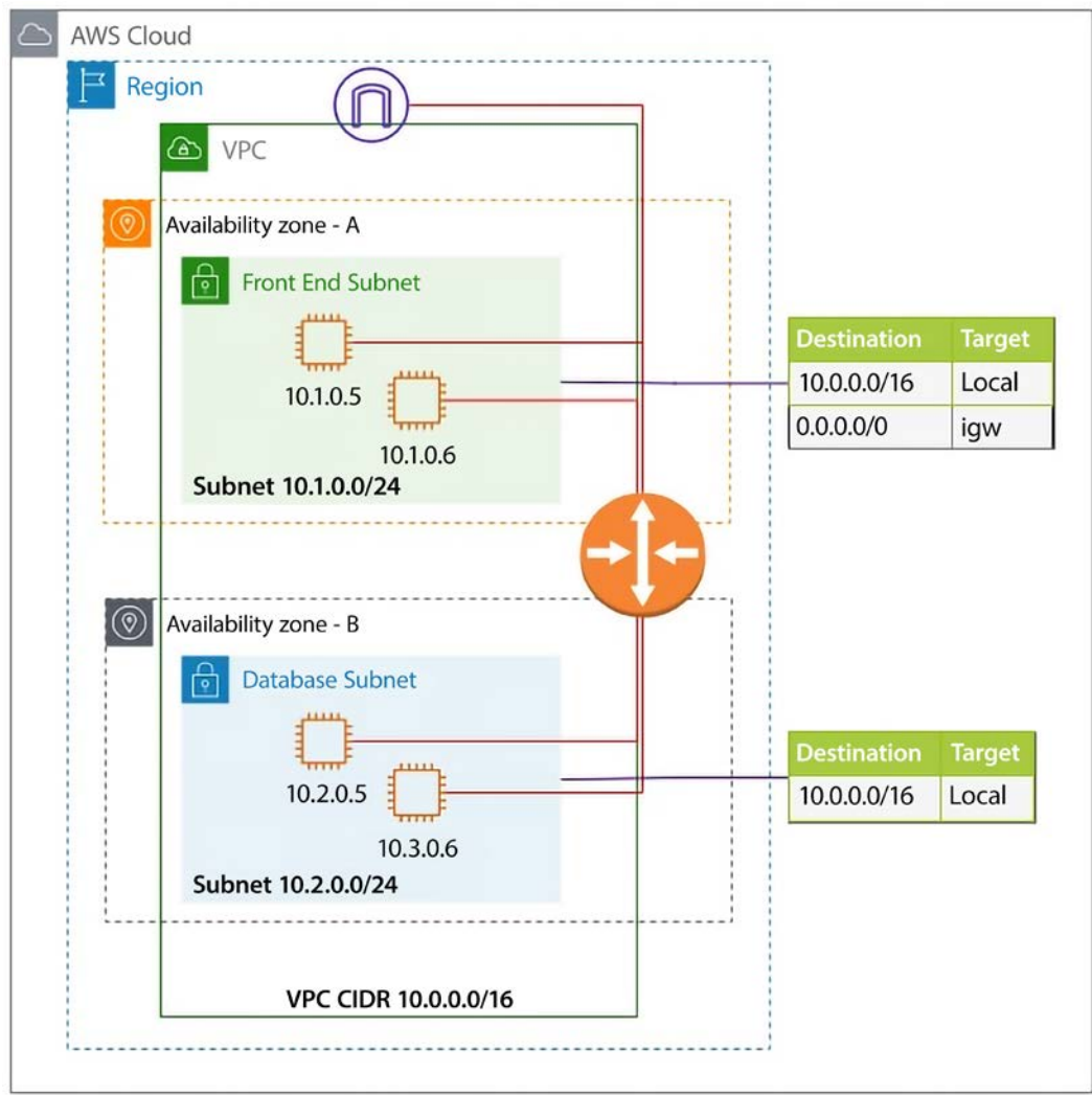
Figure 4.3: AWS VPC network architecture
