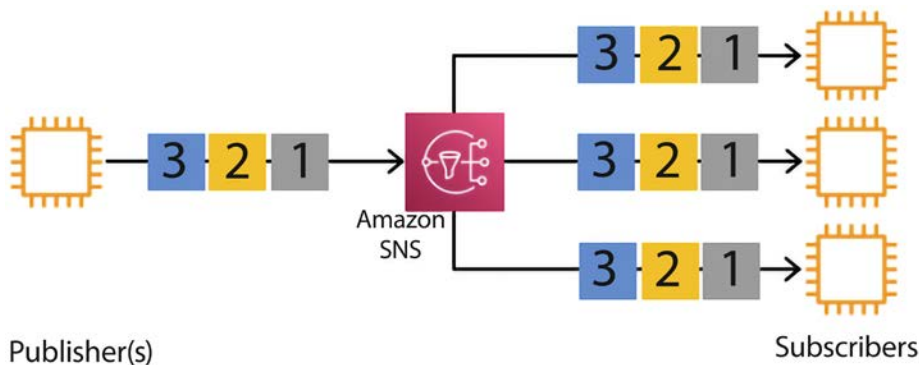
Figure 14.7: Event-driven pub/sub model in AWS
