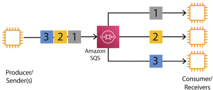
Figure 14.5: Event-driven message queuing model in AWS
