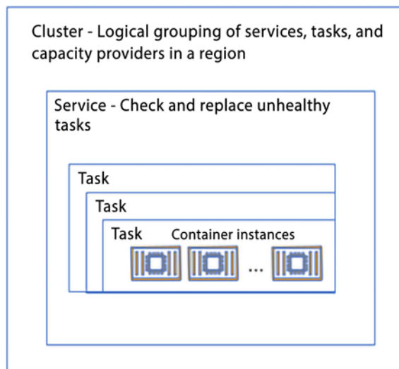
Figure 13.4: Amazon ECS architecture
