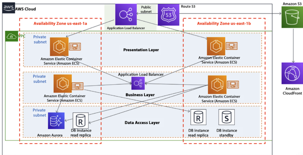
Figure 14.3: Three-layer microservice architecture in AWS
