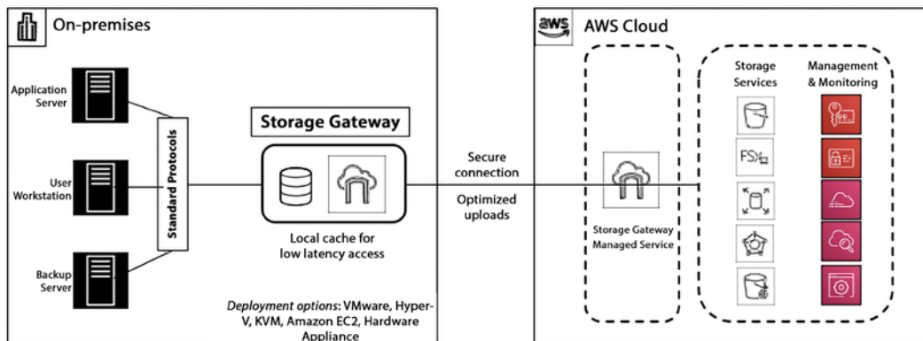
Figure 5.9: AWS Storage Gateway
