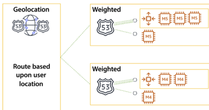
Figure 4.9: Route 53 nested routing policy
