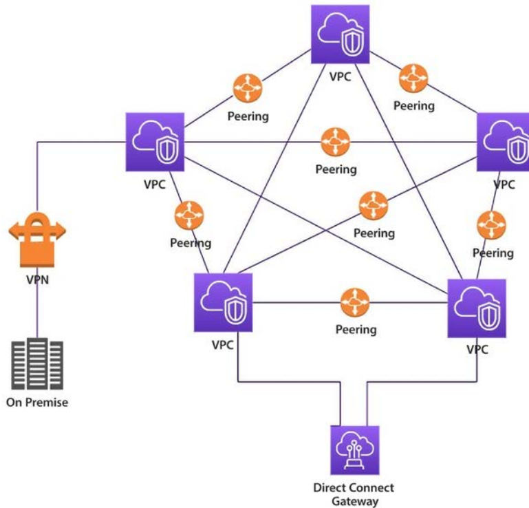
Figure 4.4: VPC connectivity using VPC peering without TGW
