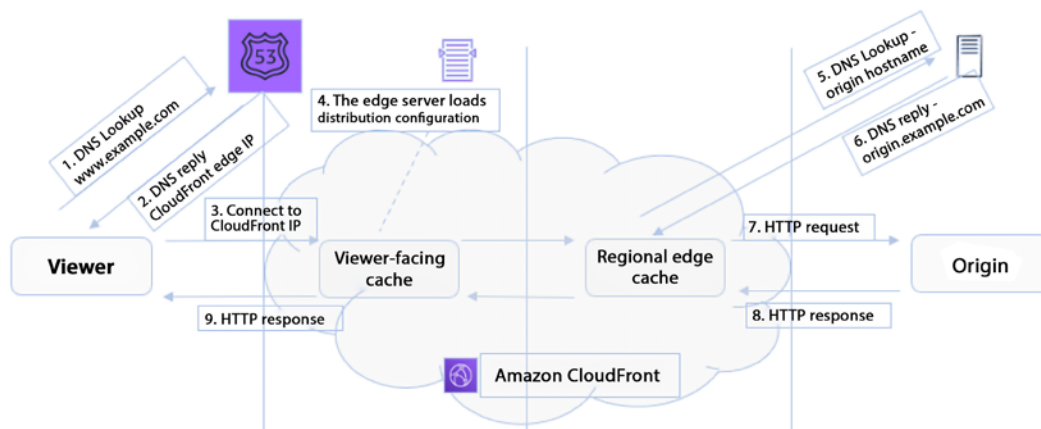
Figure 4.10: HTTP request flow with Amazon CloudFront
