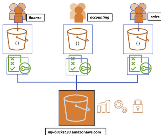
Figure 5.4: Amazon S3 Access Points
