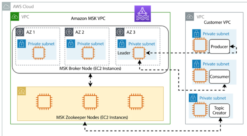
Figure 10.3: Amazon MSK architecture
