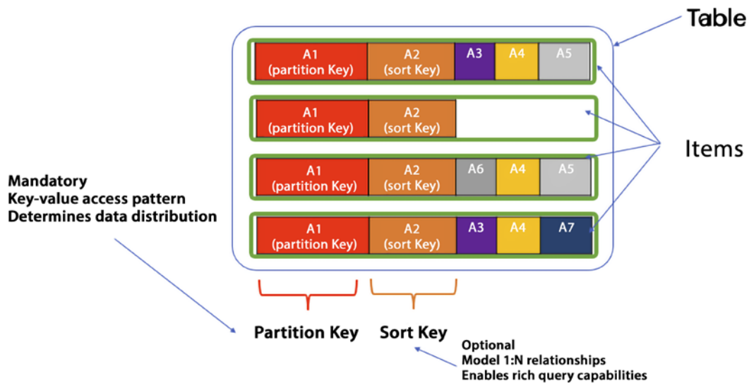
Figure 7.3: DynamoDB table with partition and sort key
