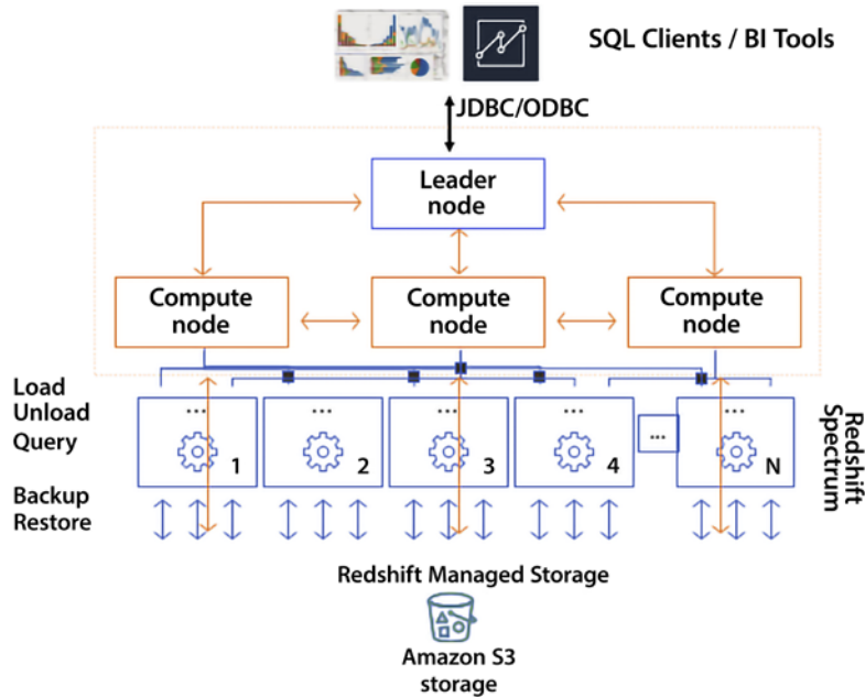
Figure 11.1: Redshift cluster architecture
