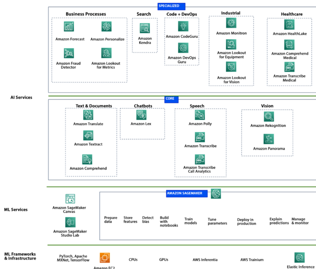
Figure 12.1: AWS ML Services Stack
