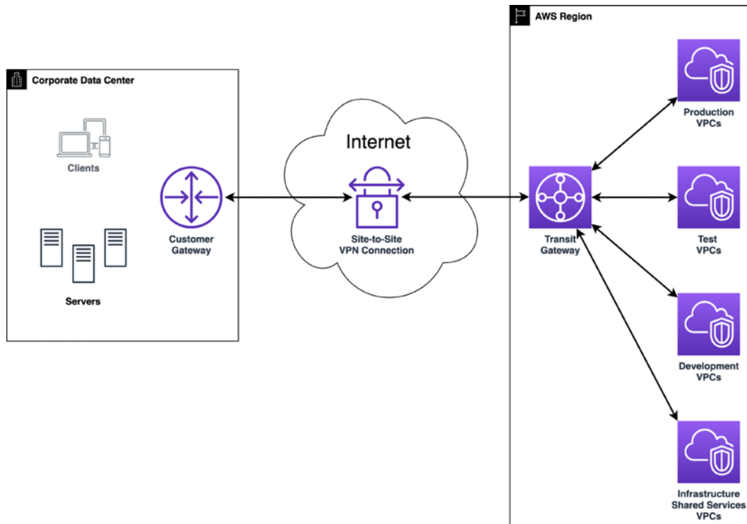
Figure 4.11: AWS Site-to-Site VPN with TGW
