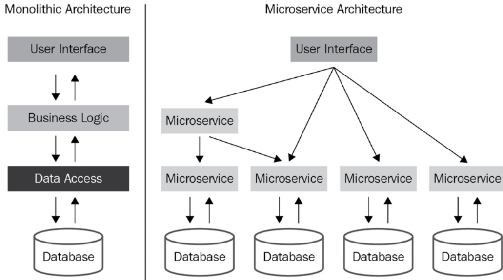
Figure 14.1: Monolithic versus microservice architectures
