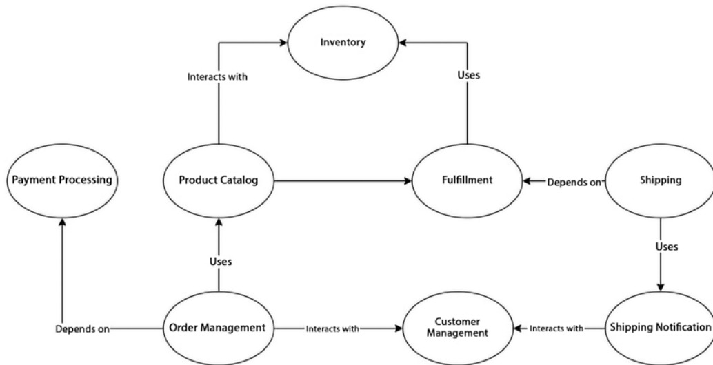
Figure 16.1: Domain-driven design context map diagram for AWSome Store
