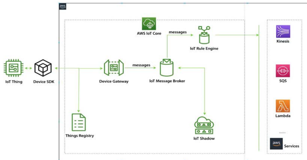
Figure 12.4: AWS IoT Services
