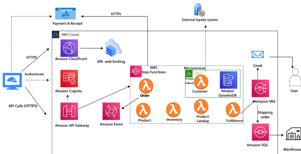
Figure 16.3: AWS cloud-native architecture to build AWSome Store
