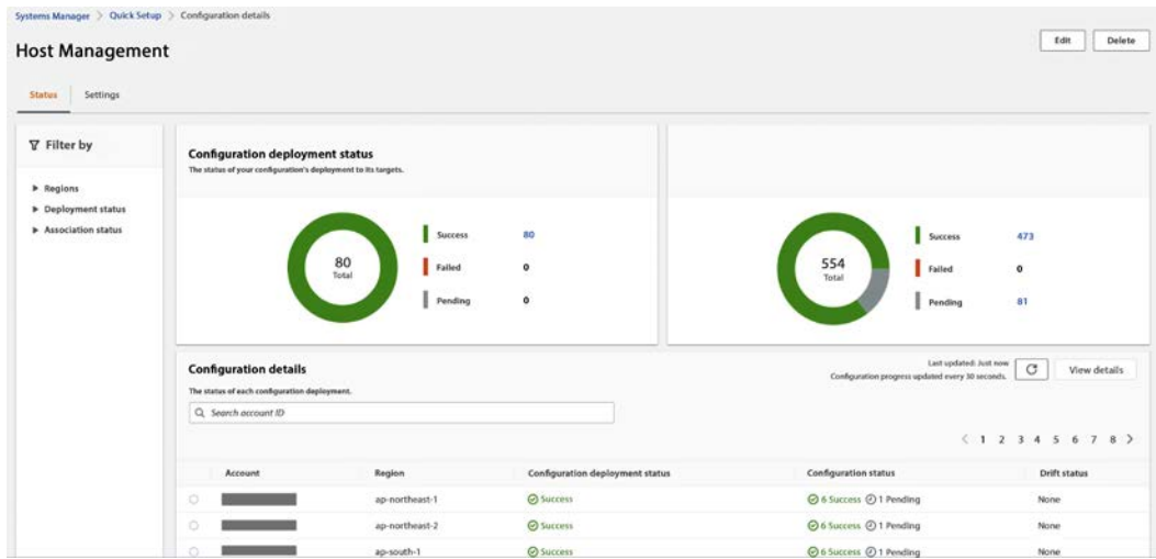
Figure 9.4: AWS Systems Manager host management
