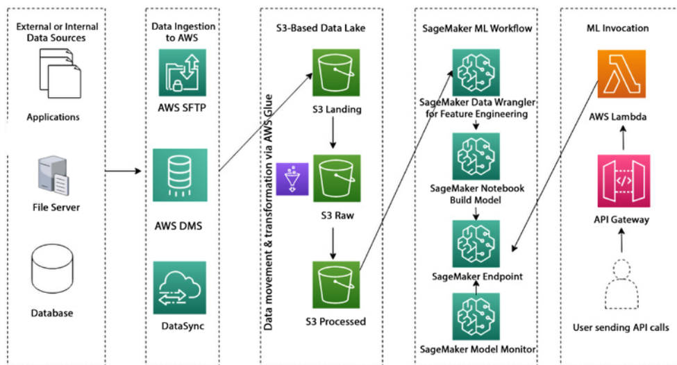
Figure 12.3: End-to-end ML Pipeline in AWS
