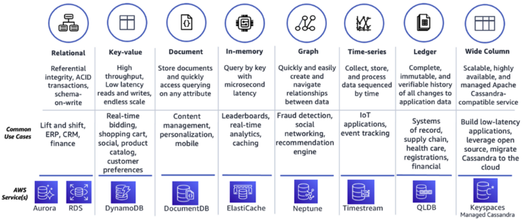
Figure 7.8: AWS database services in a nutshell
