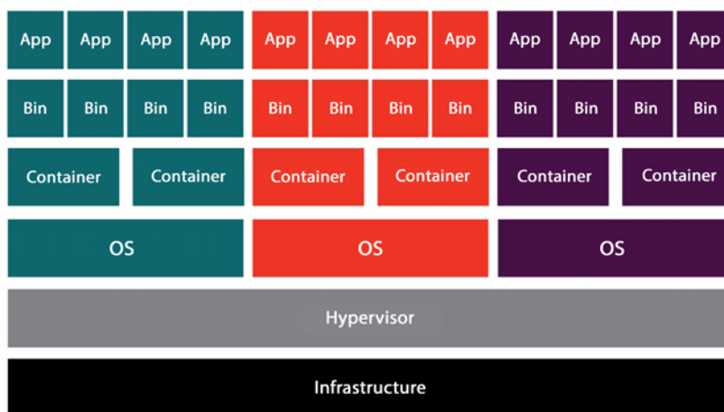
Figure 13.2: Architecture for container virtualization
