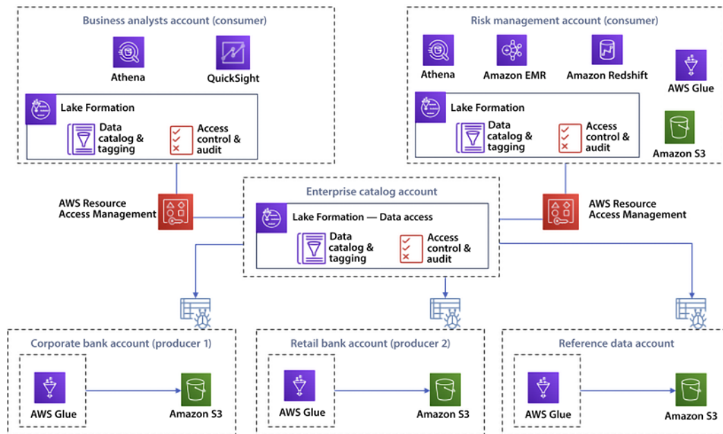
Figure 15.4: Data mesh architecture in AWS
