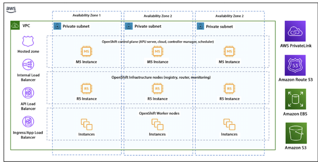
Figure 13.7: ROSA private cluster architecture
