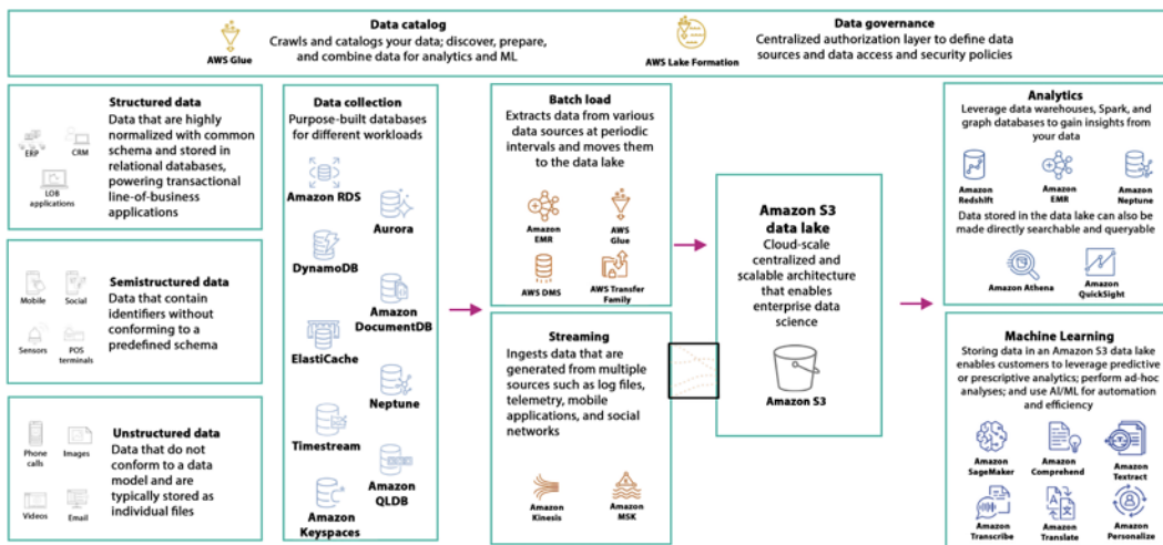
Figure 15.3: AWS data lake components
