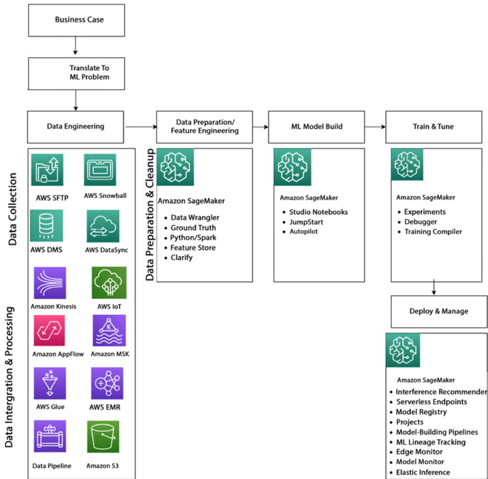
Figure 12.2: AI/ML Pipeline and Amazon SageMaker
