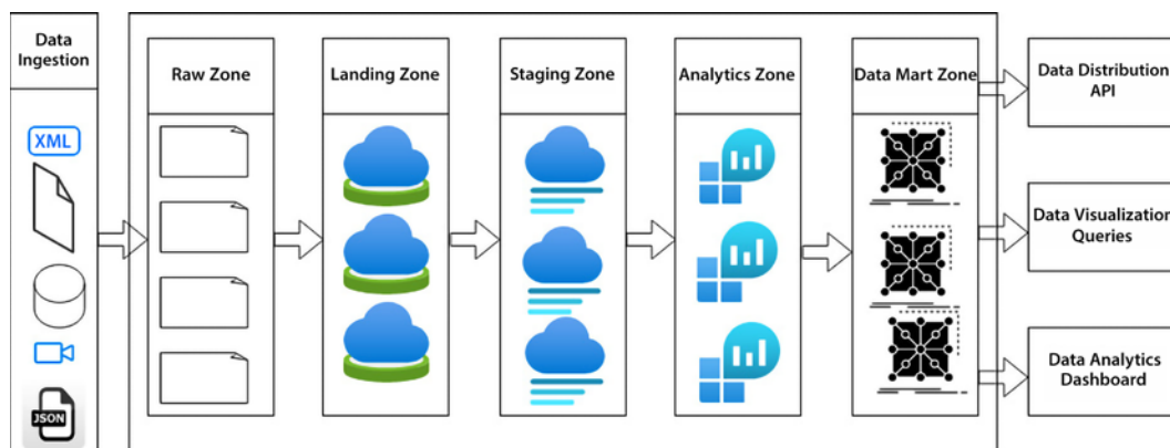
Figure 15.2: The different zones of a data lake
