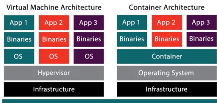
Figure 13.1: VMs versus containers
