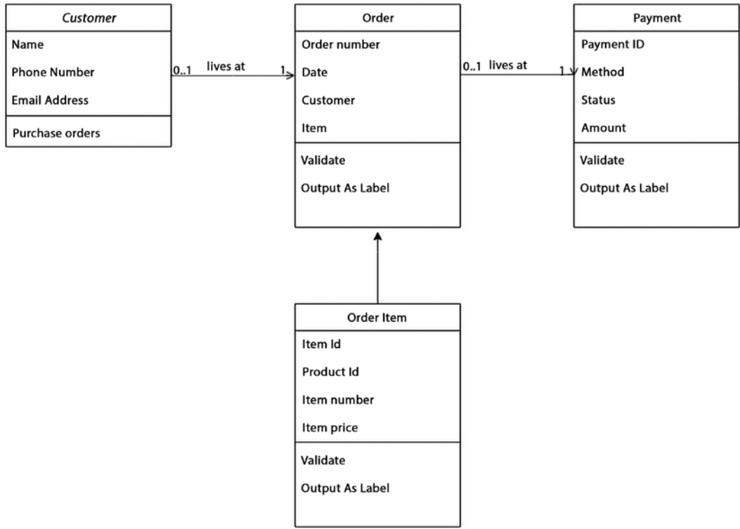
Figure 16.7: Order context class diagram
