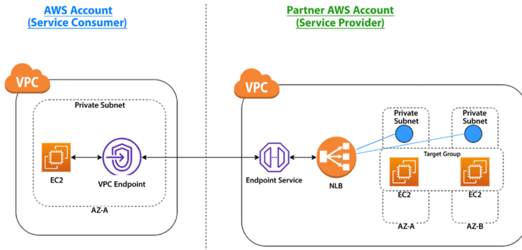
Figure 4.6: PrivateLink between partner Service Provider and Service Consumer accounts
