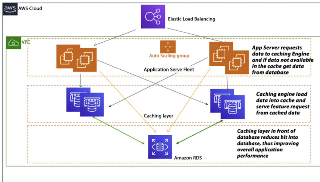
Figure 7.4: Application caching pattern architecture
