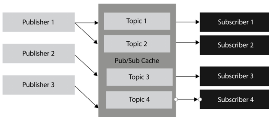
Figure 14.6: The pub/sub model
