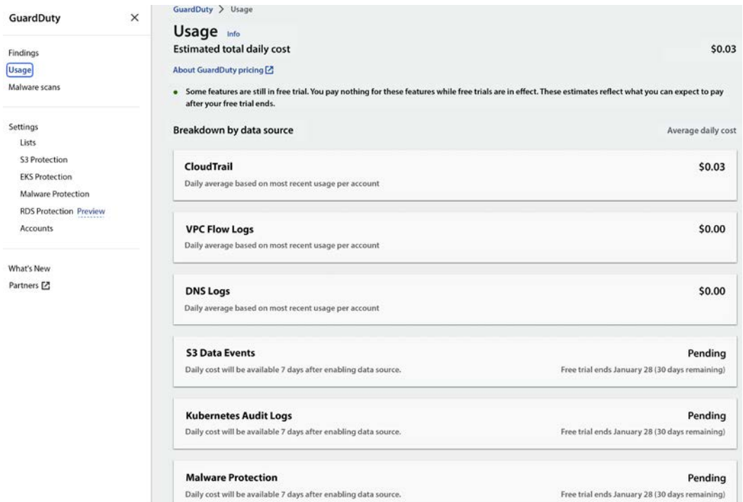
Figure 8.8: Amazon GuardDuty data source list
