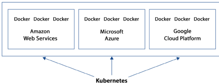
Figure 13.5: Sample architecture for a multi-cloud Kubernetes deployment
