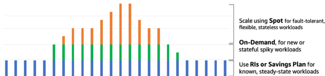
Figure 6.1: EC2 pricing model to optimize cost
