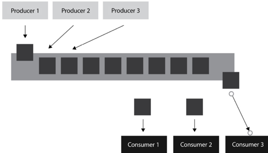
Figure 14.4: Event streaming model
