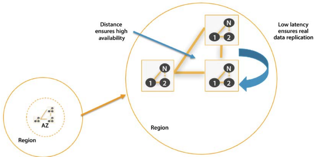
Figure 4.1: AWS Regions and AZs
