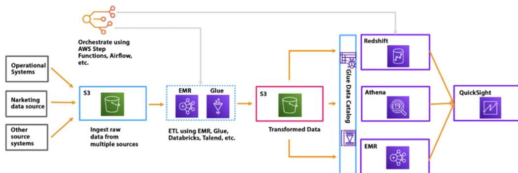
Figure 11.6: Data analytic architecture in AWS
