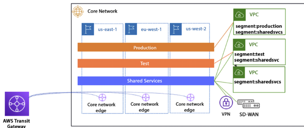
Figure 4.14: AWS Cloud WAN architecture
