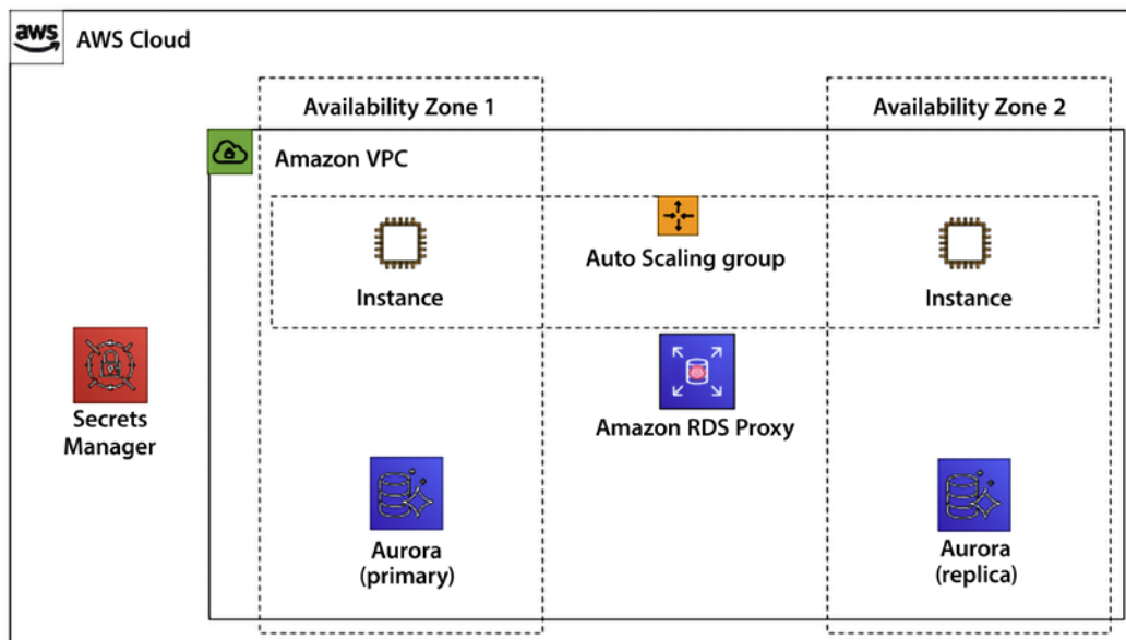
Figure 7.2: Amazon Aurora's high availability with RDS proxy
