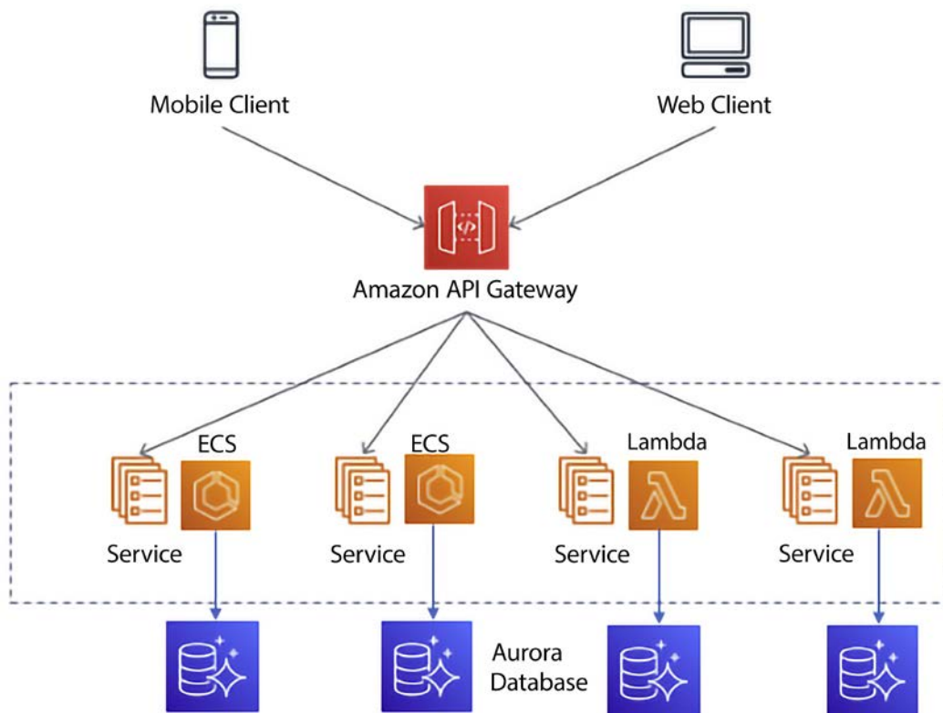
Figure 14.2: Microservice architectures in AWS
