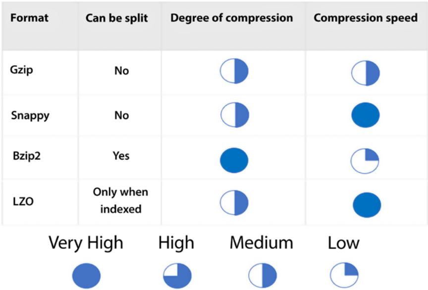
Figure 11.3: Compression formats
