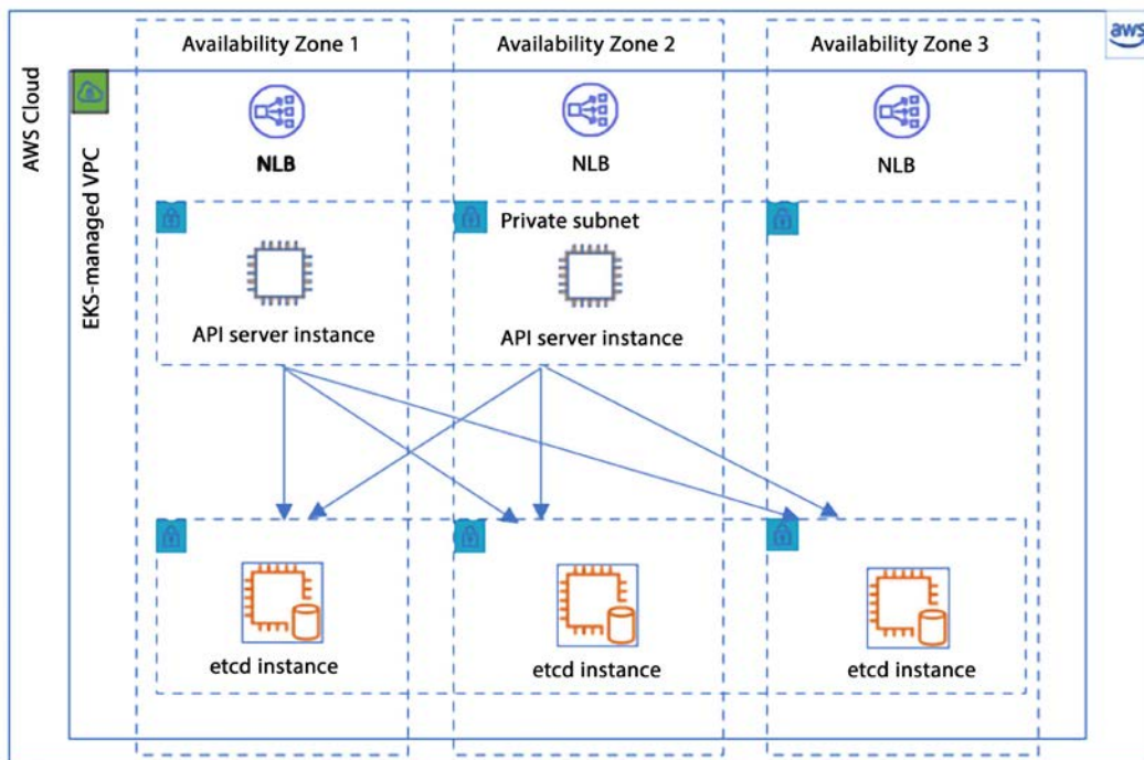
Figure 13.6: Amazon EKS control plane architecture
