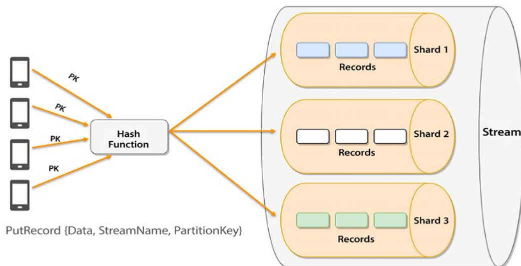
Figure 10.5: Amazon Kinesis architecture
