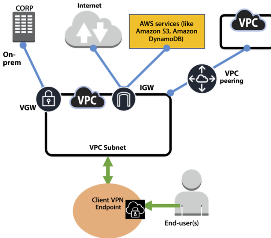
Figure 4.12: AWS Client VPN
