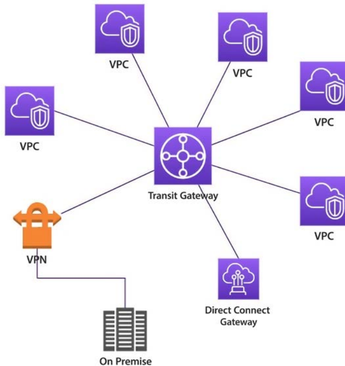
Figure 4.5: VPC connectivity with TGW
