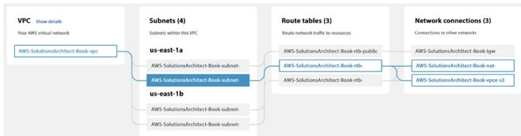
Figure 4.2: AWS VPC configuration with a private subnet flow
