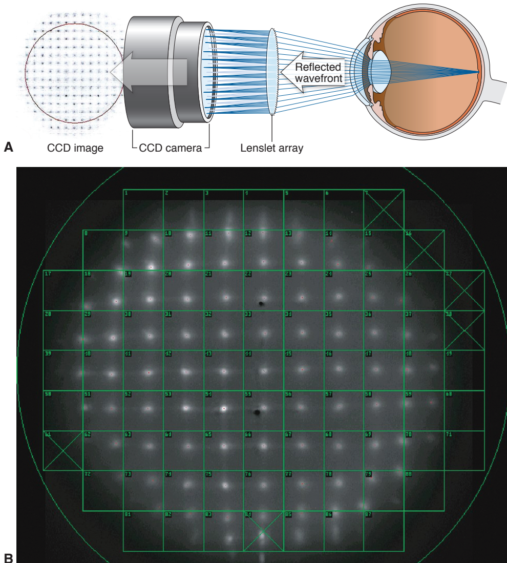
Figure 1-2 Schematic of a Hartmann-Shack wavefront sensor. A , The reflected wavefront passes through a grid of small lenses (the lenslet array ), and the images formed are focused onto a charge-coupled device (CCD) chip. The degree of deviation from the expected focal points determines the aberration and thus the wavefront error. B , Example of the images formed after the wavefront passes through the lenslet array. The green overlay lattice is registered to correspond to each lenslet in the array. (Part A illustration by Mark Miller.)
