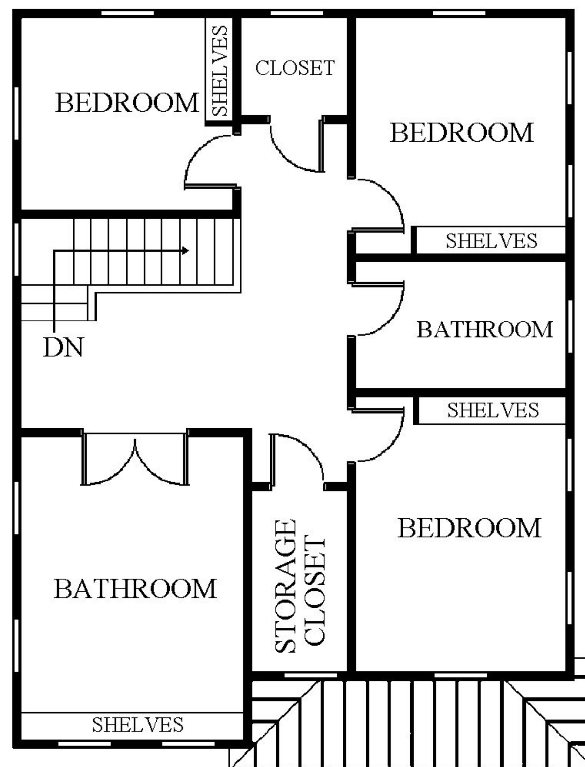
SECOND FLOOR
