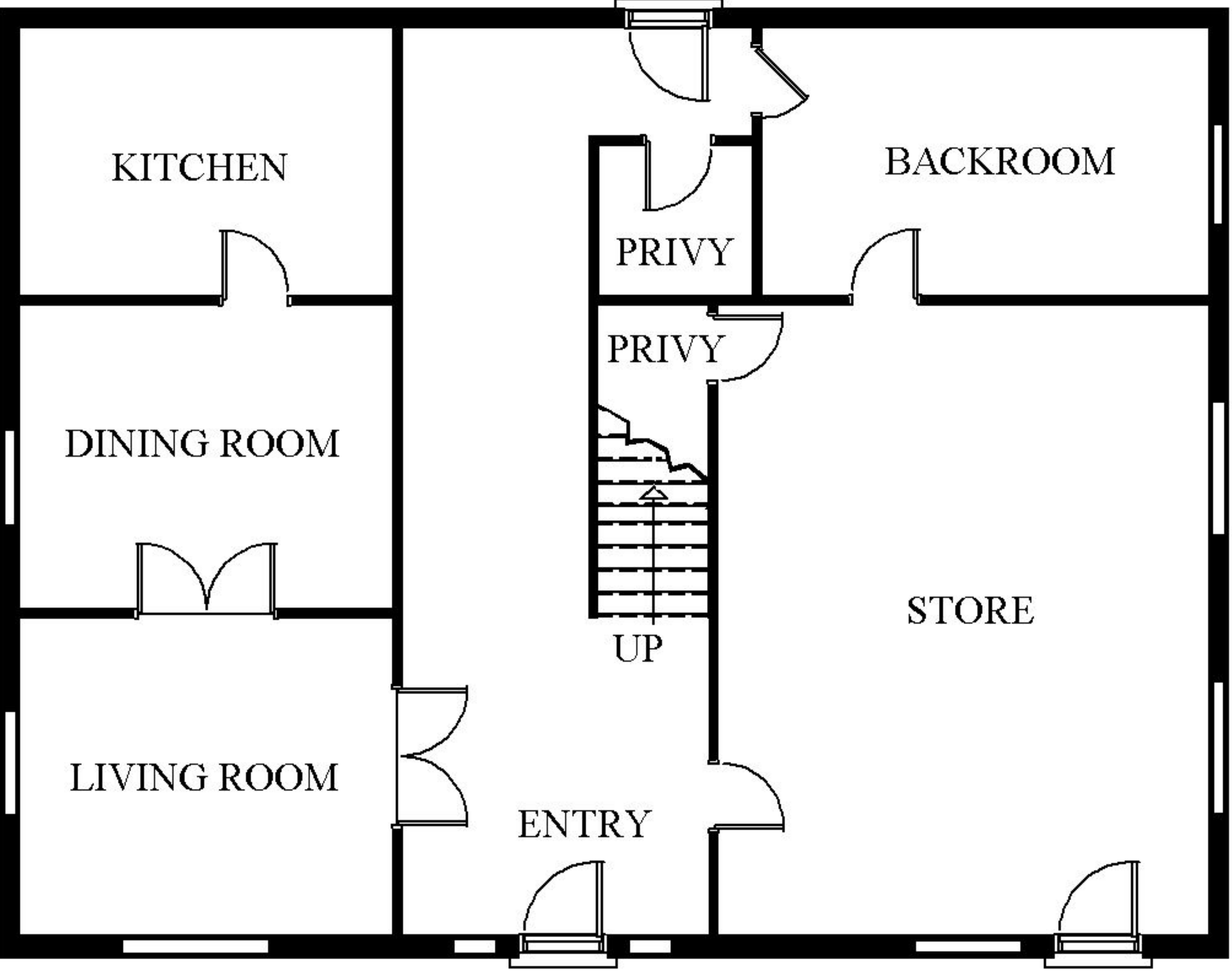
FIRST FLOOR
