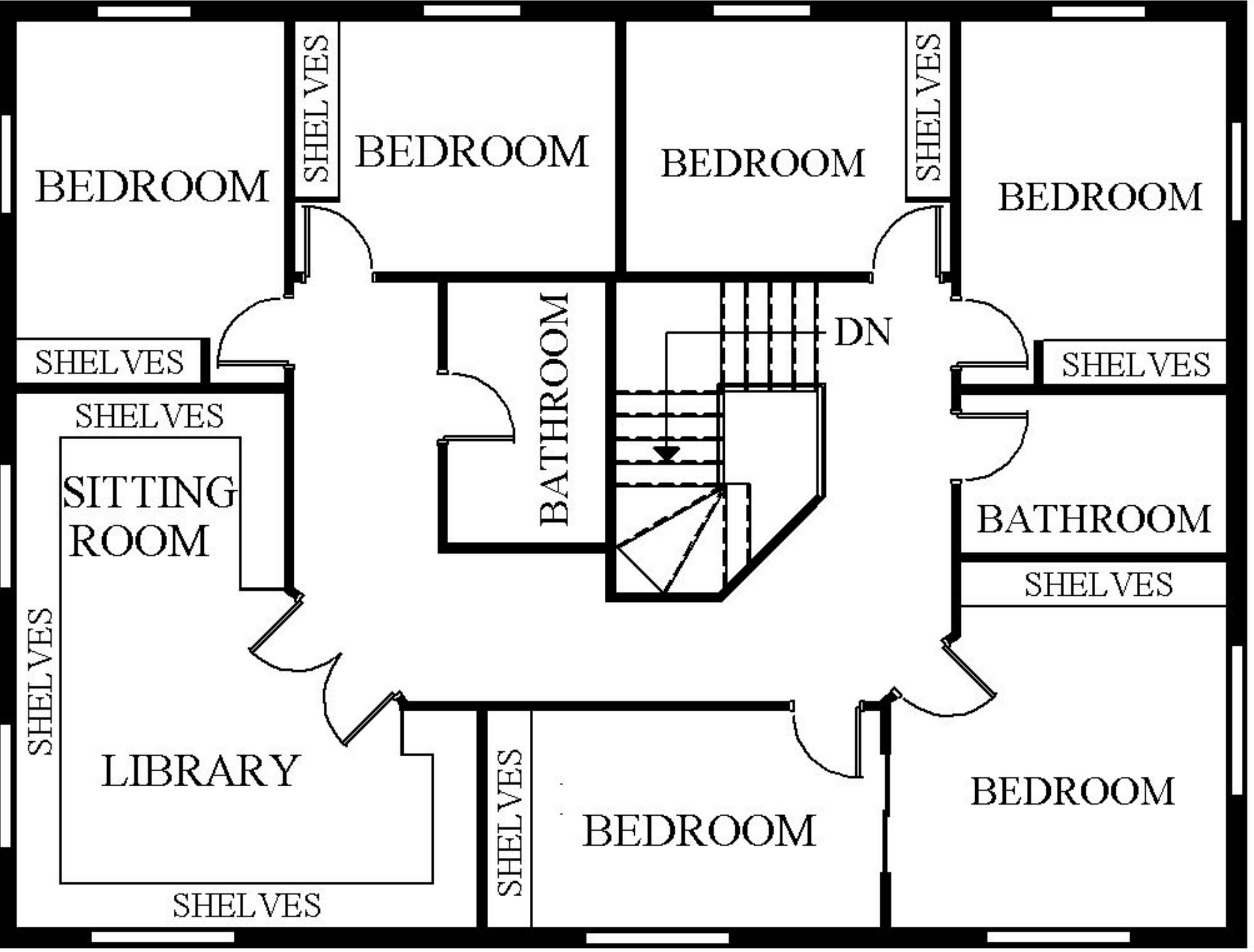
SECOND FLOOR
