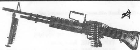
M60 with bipod extended and ammunition belt inserted
