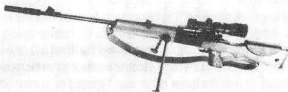
FR-F1 with bipod extended
