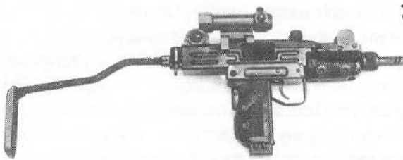
Mini UZI fitted with the Armson OEG sight, with 20 rd magazine
