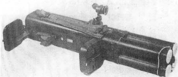
M202A1 Flash with 4 rd rocket clip fitted
