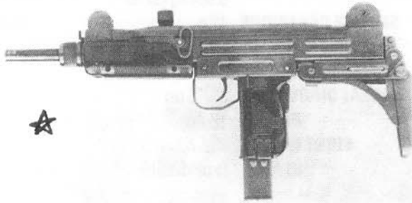
UZI with Hebrew markings, fitted with a 25 rd magazine and metal stock (folded)
