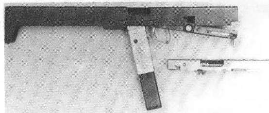
FMG partially field stripped showing the bolt/barrel assembly separate from the weapon, the hinged trigger guard and magazine well are unlocked and partially folded
