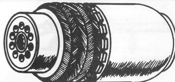
HE (short) showing pre-engraved rotating band and propellant chamber
