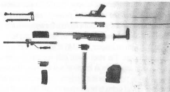
LMG field stripped with both belt feed with ammunition and magazine feed magazine
