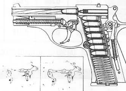
Beretta M84 cross section
