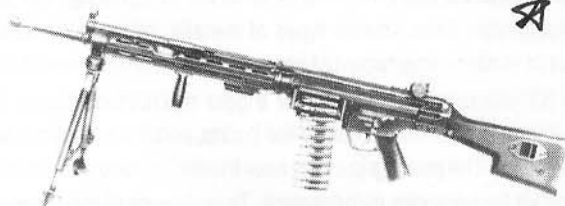
HK21E with ammunition belt inserted and selector set on safe
