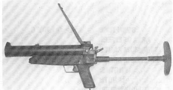
Granatepistole with stock extended and rear sight raised for long range fire
