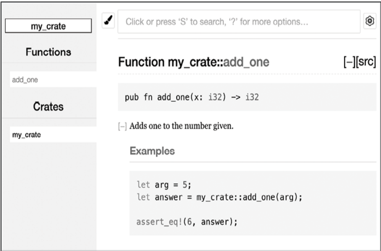
Figure 14-1: HTML documentation for the add_one function
