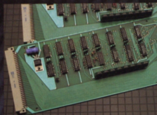
Memory Expansion Board
