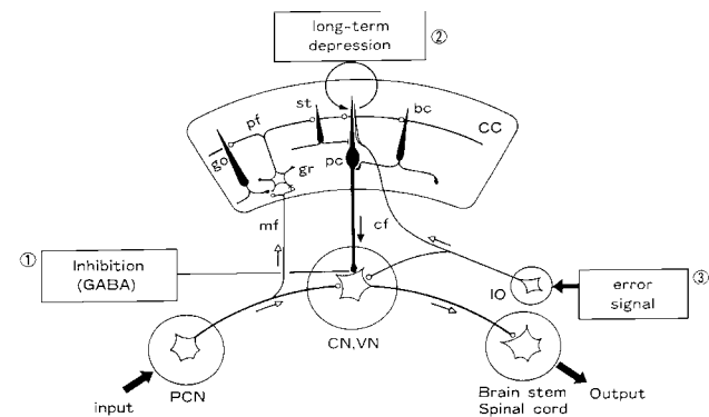
Figure 1. Neuronal circuitry of the cerebellum. CC, cerebellar cortex; pc, Purkinje cell; bc, basket cell; st, stellate cell; pf, parallel fiber; gr, granule cell; go, Golgi cell; mf, mossy fiber; cf, climbing fiber; IO, inferior olive; PCN, precerebellar nuclei; CN, cerebellar nuclei; VN, vestibular nuclei.
