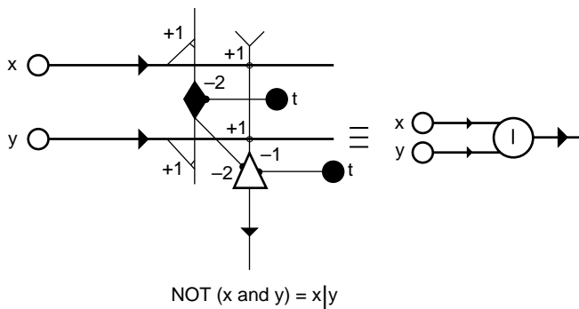
Figure 2. NAND logic function implemented by a McCulloch-Pitts net comprising two units.
