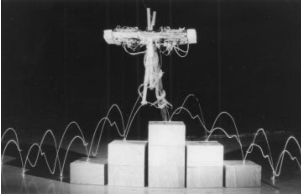
Figure 2. The planar biped running right to left, up and down a short flight of stairs. Photograph reprinted by permission of the MIT Leg Laboratory.
