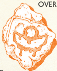
MAJOR CREST OF OVERFLOWING CHALK
