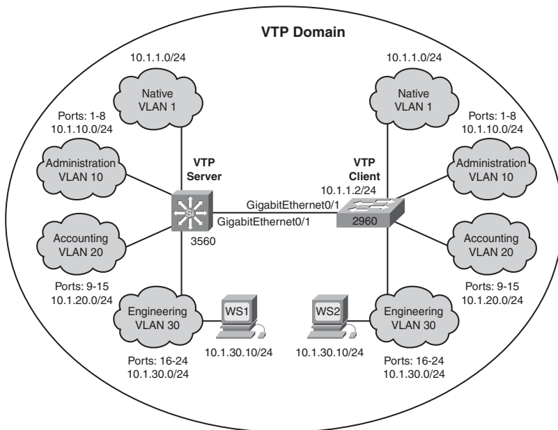
Figure 2-1 Network Topology for VLAN Configuration Example
