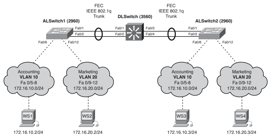
Figure 2-3 Network Topology for EtherChannel Configuration
