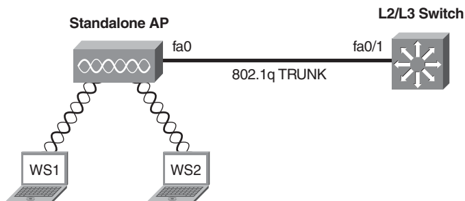
Figure 9-2 Switch Configuration for Standalone APs and HREAPS
