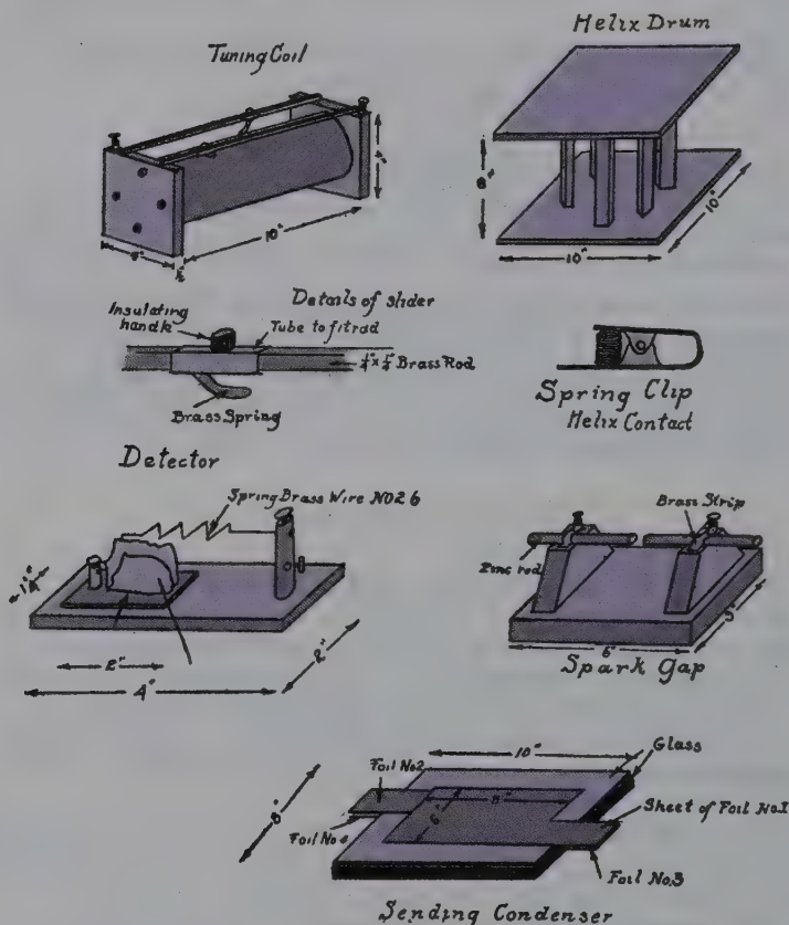
Details of instruments for field use.
