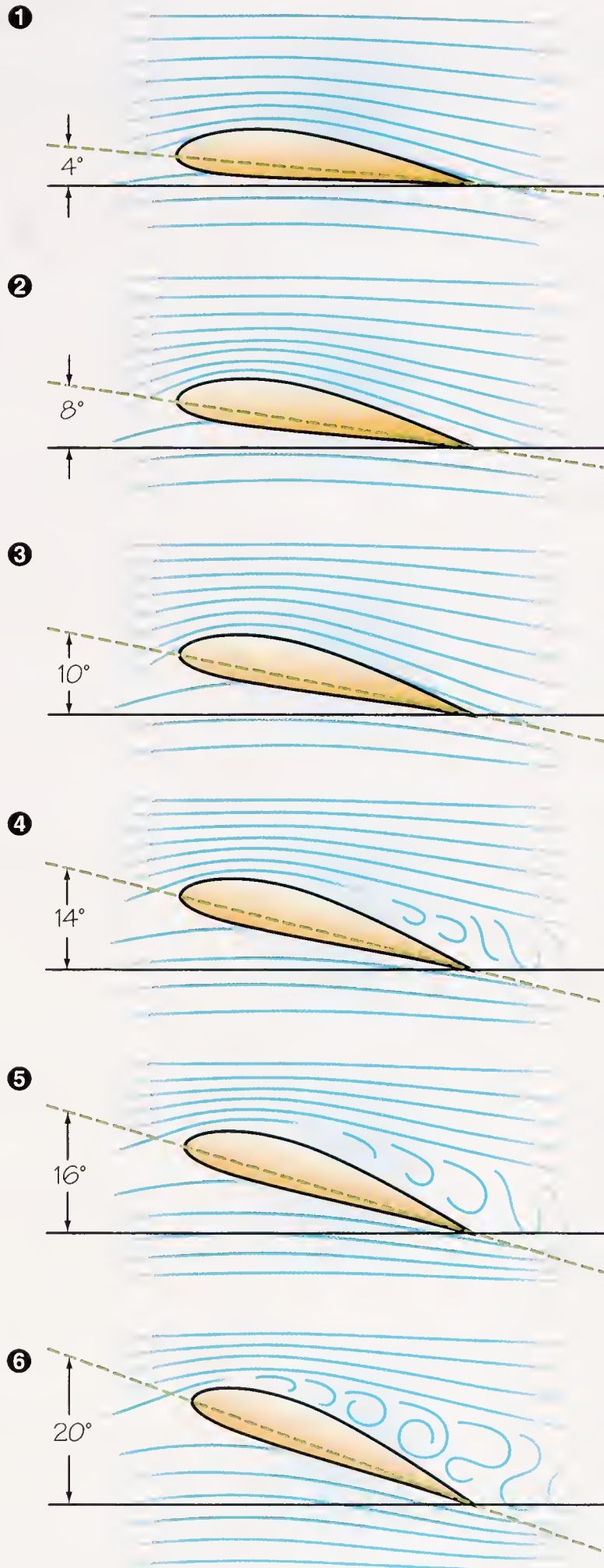
How airfoils work
