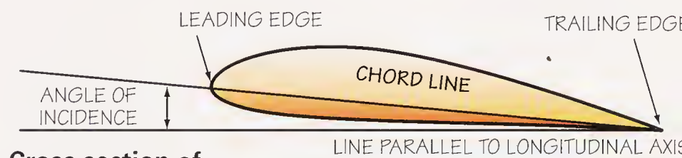
Cross section of an airfoil
