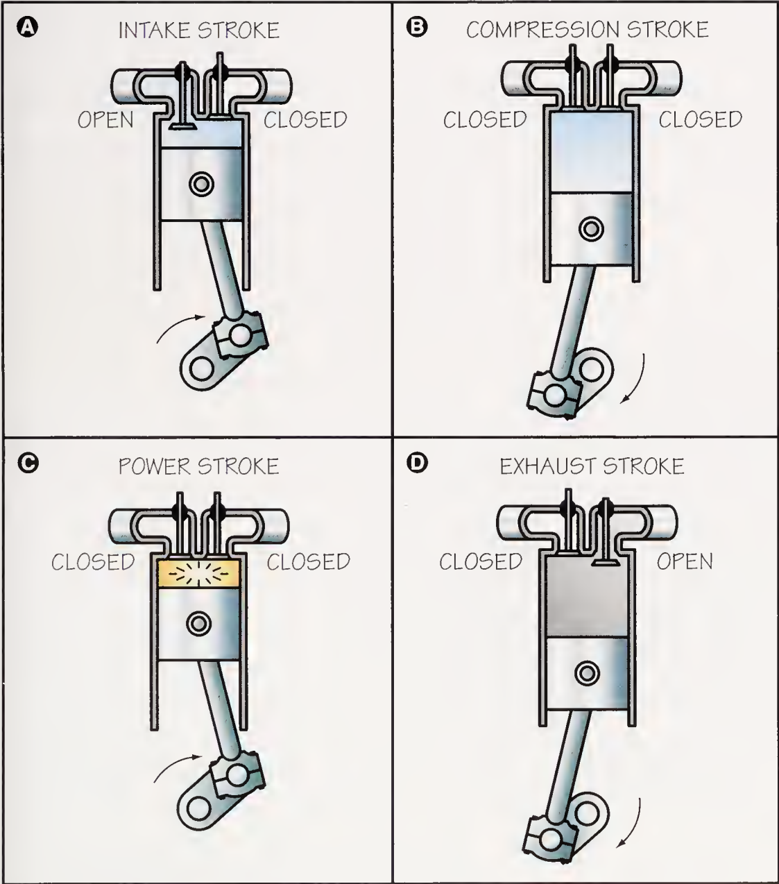
How a piston engine develops power
