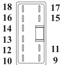
Internal Transmission Harness "Male" Coupler Connector Number "JB10"
