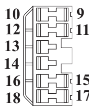
Internal Transmission Harness "Female" Coupler Connector Number "JB10a"
