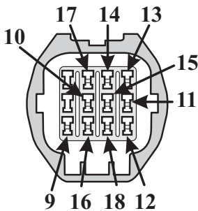
External Transaxle Harness Connector Number "H2-03"
