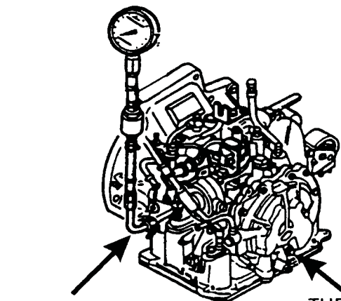
LINE PRESSURE
