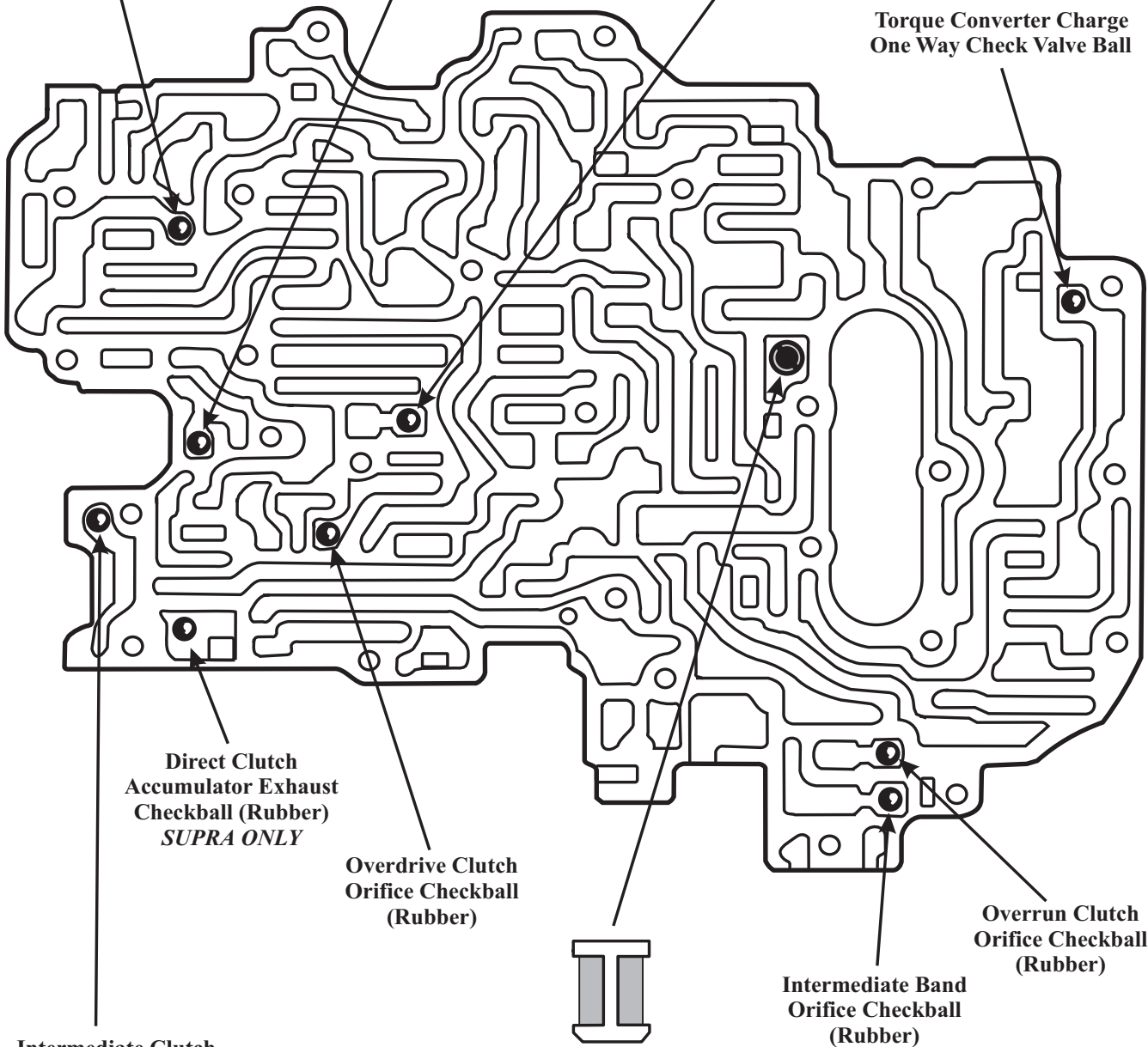
Solenoid Oil Screen 11.6 X 8.3mm
