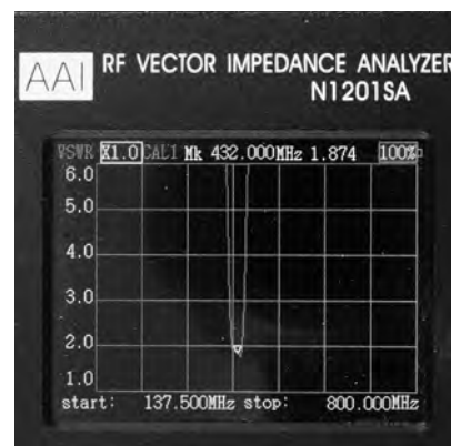
Figure 13 — Input VSWR of a band-pass filter with 50\ \Omega termination on the output showing the filter frequency range.
