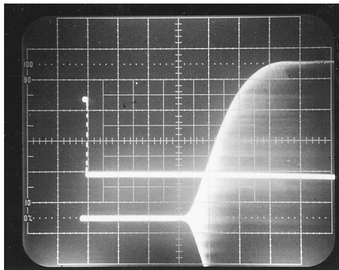
Fig. 4-8A — Oscilloscope Trace of RF Envelope
