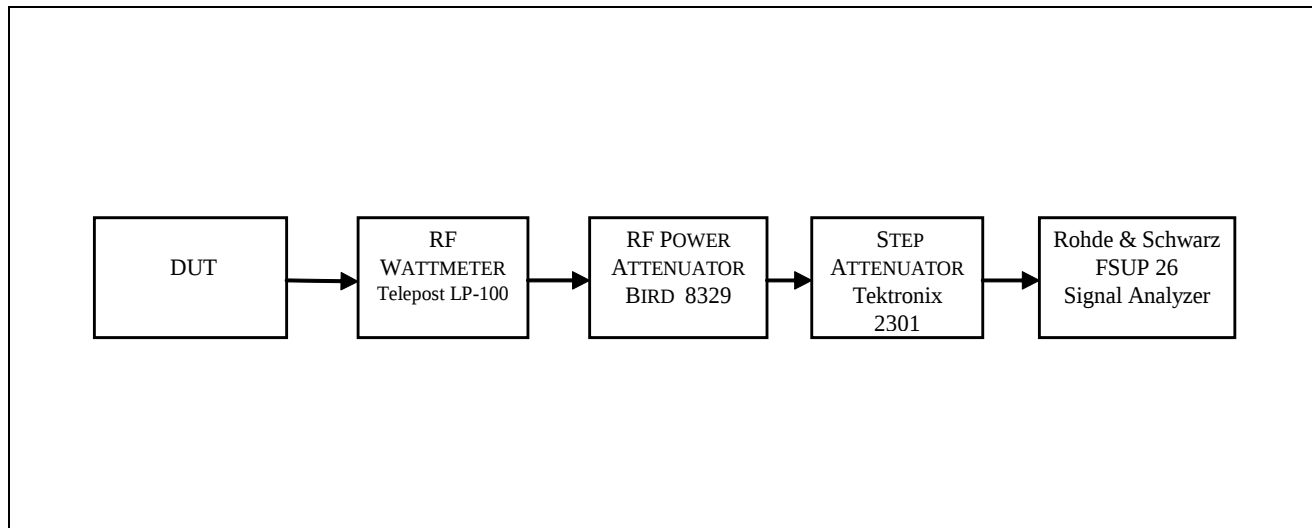
Fig. 4-11 — Phase Noise Test Hook-up
