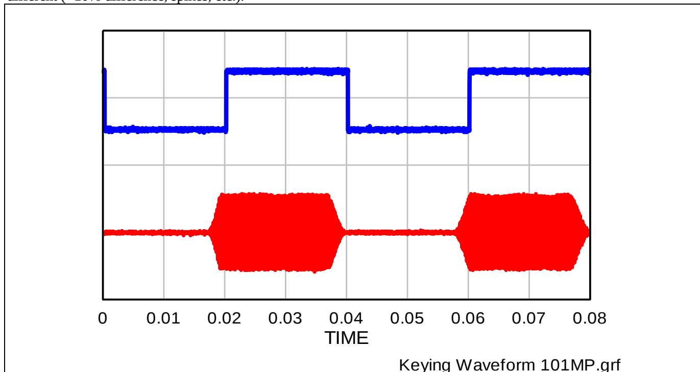
Fig. 4-7A — Oscilloscope Trace of RF Output Envelope
