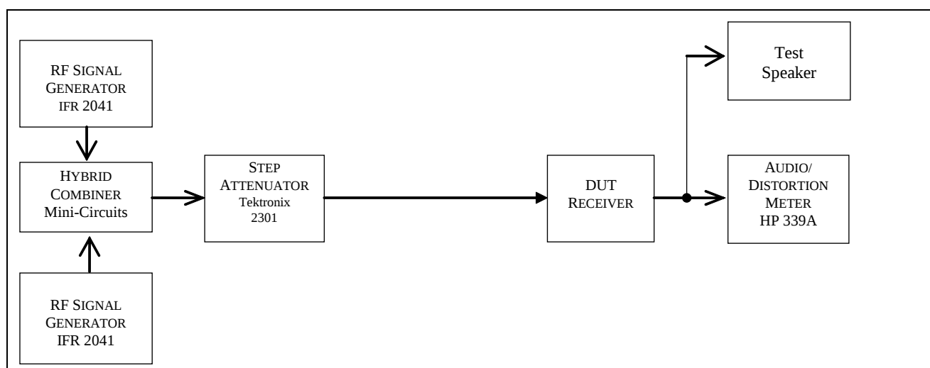
Fig. 5-9 — FM Adjacent Channel Selectivity Test Hook-up
