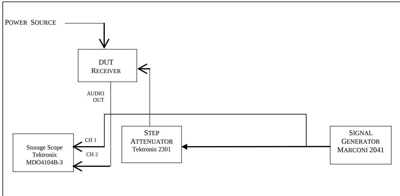
Fig. 5-16A — Notch Attack Time Test Hook-up
