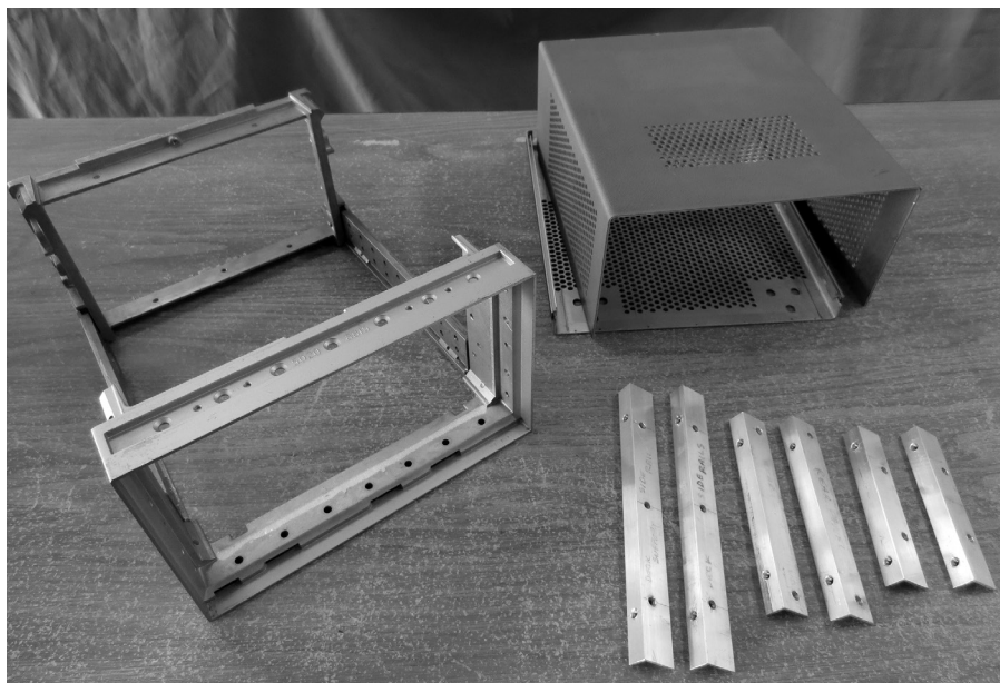
Figure 2 — Recovered instrument frame and new brackets.
