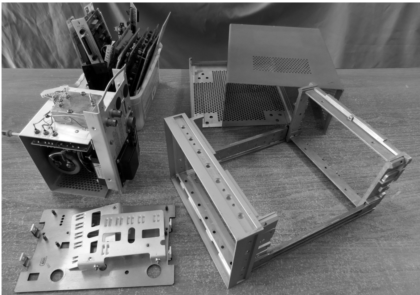
Figure 1 — Disassembled HP-436A power meter.
