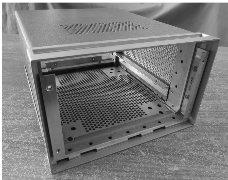
Figure 3 — Instrument frame with new brackets installed.
