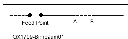
Figure 1 — One side of a symmetrical loaded dipole shows the gap between A and B where length is removed and a trap is inserted.
