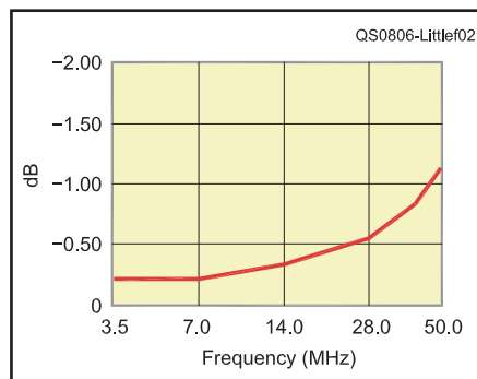
Figure 2 — Total loss of transformer and balun versus frequency.
