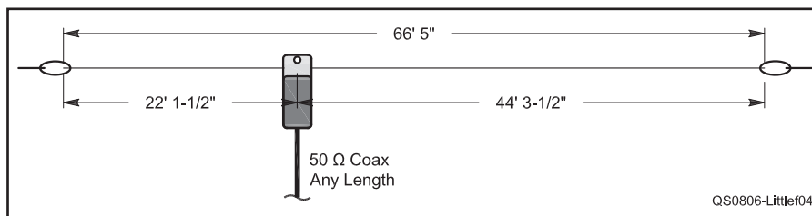
Figure 4 — Cutting dimensions for OCFD.
