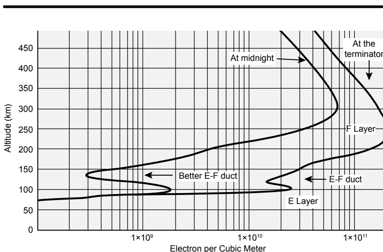
Figure 7 — The duct between the E and F layers of the ionosphere. Note the more pronounced duct at midnight, compared to the duct at the terminator. [Adapted from Robert R. Brown, NM7M, "On the SSW Path and 160-Meter Propagation," QEX, Nov/Dec 2000, pp. 3-9, Figure 1.]
