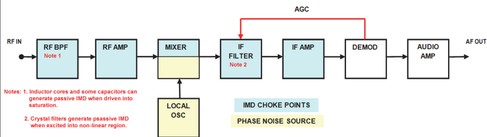
Simplified block diagram of superhet receiver
