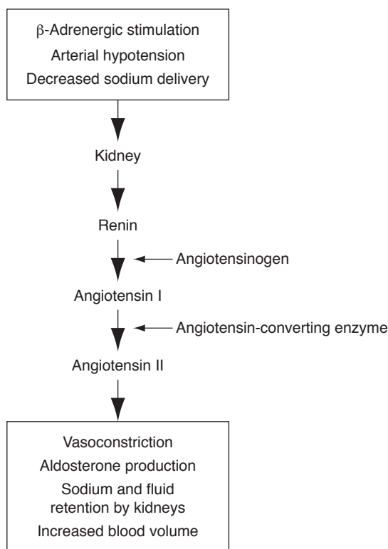
Figure 4-1 Renin-angiotensin-aldosterone system.
